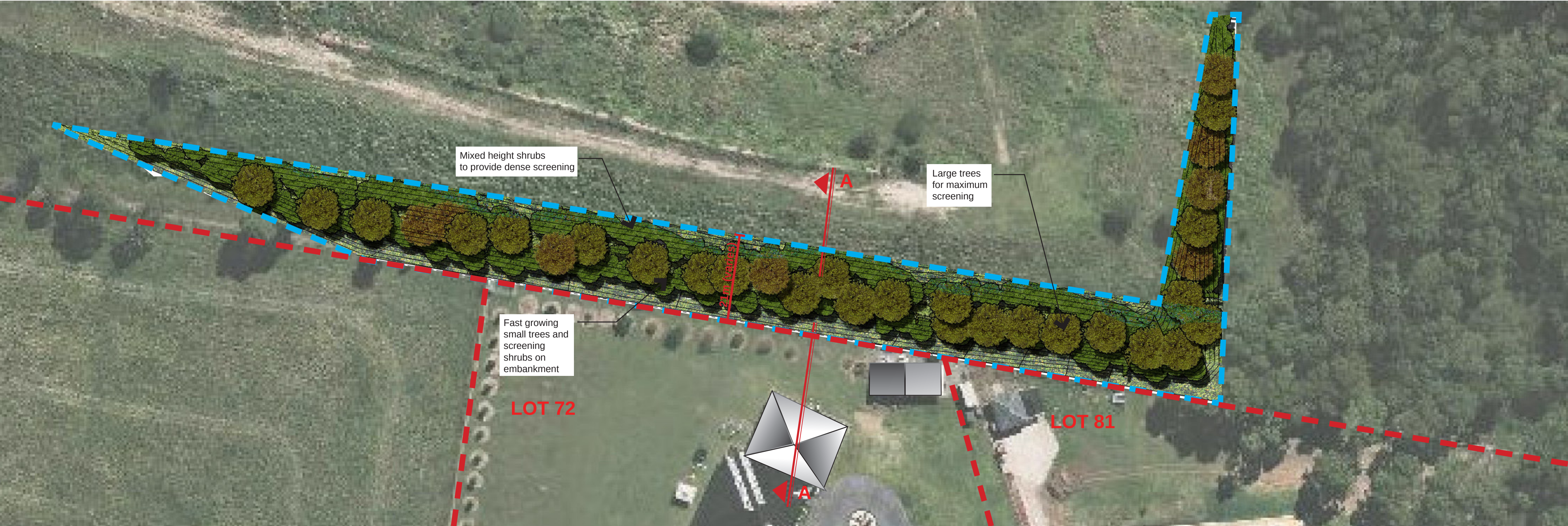
SOUTHERN BOUNDARY INTERFACE LANDSCAPE BUFFER PLAN 1:500 @ A1
