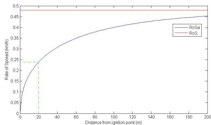
Figure 17. The accelerating rate of spread RoSa and the equilibrium rate of spread RoS against the distance from the ignition point D .
