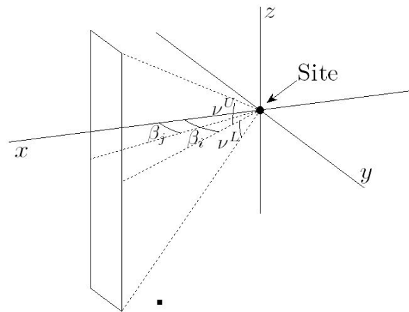
Figure 10. Any rectangle specified by a set of angles \beta_i , \beta_j , \nu_i^U , and \nu_i^L will have the same view factor relative to the site. Note that \nu_i^U > 0 and \nu_i^L < 0 , while \beta_i > 0 and \beta_j > 0 .
