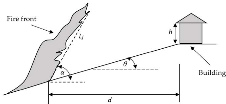
Figure 4. Typical building and fire front configuration.
