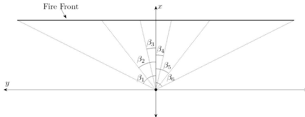
Figure 9. The discretisation of the fire front with respect to \beta using 6 uniformly distributed values \{\beta_i\}_{i=1}^6 looking from above. Note that \beta_1, \beta_2, \beta_3 > 0 while \beta_4, \beta_5, \beta_6 < 0 .
