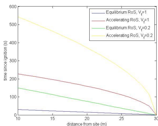
Figure 20. The progression of the fire front for modelling scenarios 5 through to 8. The yellow line represents the Case Study 2 scenario.
