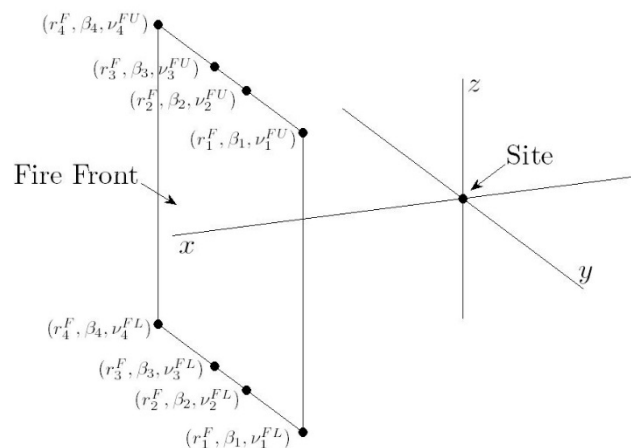
Figure 11. A flame front with top and bottom edge coordinates \{(r_i^F, \beta_i, \nu_i^{FU})\}_{i=1}^4 and \{(r_i^F, \beta_i, \nu_i^{FL})\}_{i=1}^4 respectively.
