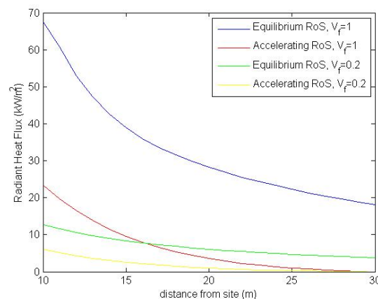
Figure 18. The radiant heat flux for models ignoring the 3 m obstructing wall. The yellow line represents the Case Study 2 scenario.
