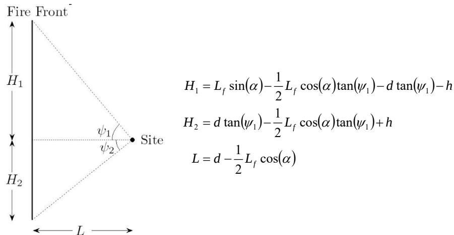
Figure 5. Geometrical representation of the side view of the site and vertical approximation of a fire front.
