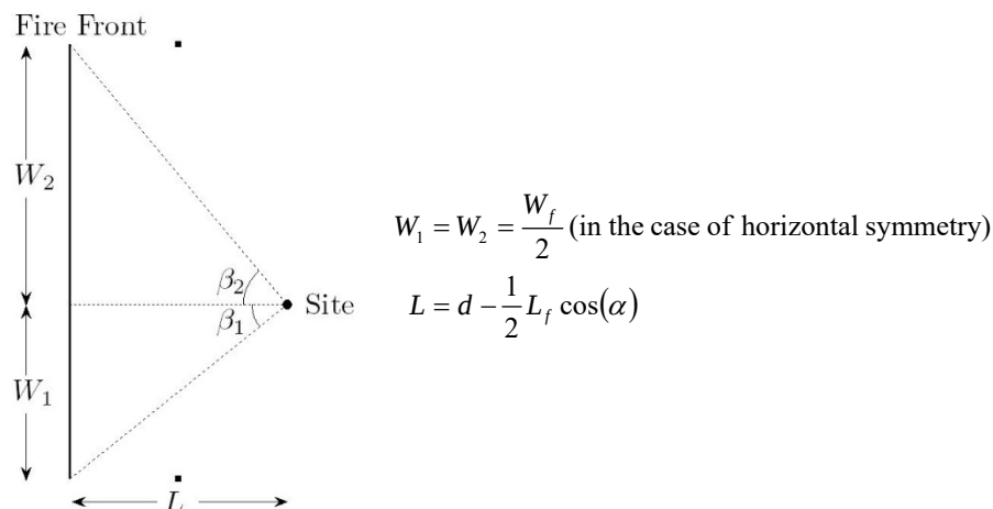
Figure 6. Geometrical representation of the birds-eye view of the site and vertical approximation of a fire front.
