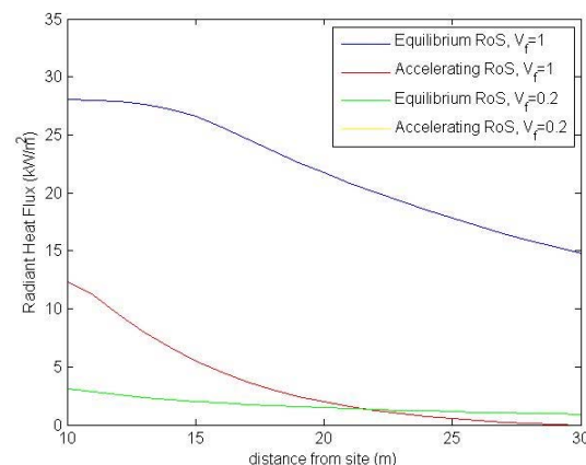
Figure 19. The radiant heat flux for models including the 3 m obstructing wall. The yellow line represents the Case Study 2 scenario.
