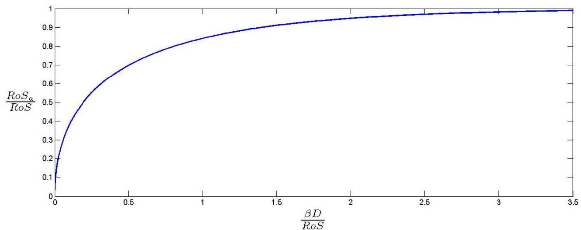
Figure 3. Plot of the ratio \frac{RoS_a}{RoS} against \frac{\beta D}{RoS} .
