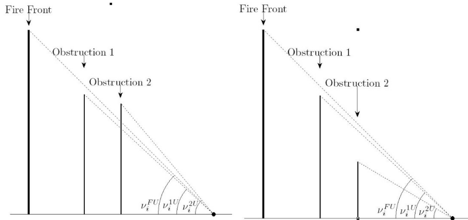
Figure 13. (Left) Obstruction 2 completely blocks the fire front from the site, so \nu_i^U = \nu_i^{FU} as the part of Obstruction 2 that extends above the view line of the top of the fire front does not contribute to blocking the fire front. (Right) Obstruction 1 partially blocks the fire front from the site, so \nu_i^U = \nu_i^{1U} .
