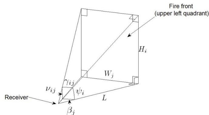
Figure 7. Geometrical representation of the upper-left quadrant of the fire front relative to the site.
