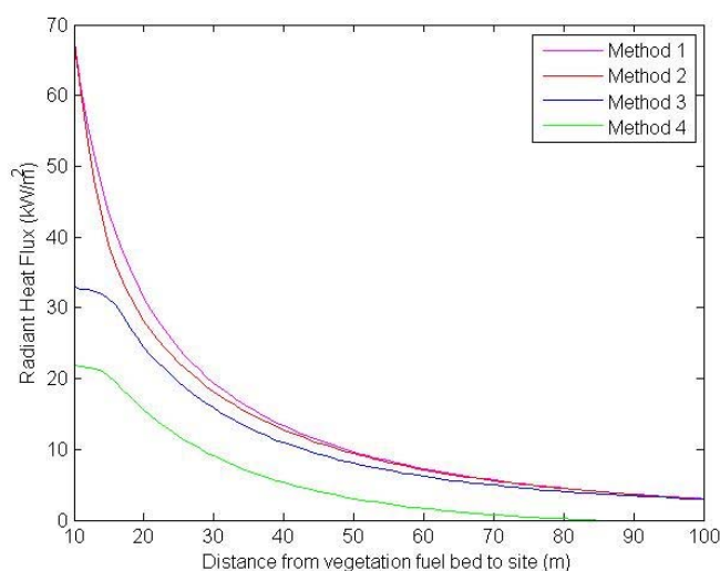
Figure 15. The radiant heat flux at the site as a function of the distance to the vegetation fuel bed.
