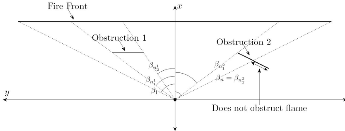
Figure 12. An obstruction may only partially obstruct the fire front and will only obstruct the fire front if it lies within the angular region.
