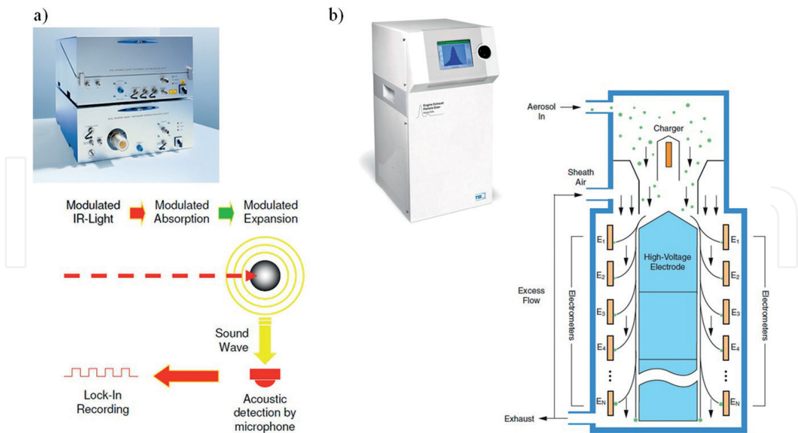
Figure 2. Equipment: (a) AVL MSS analyzers for the measurement of PM [13] and (b) TSI 3090 EEPSTM equipment for PM size distribution under actual conditions of operation [14].
