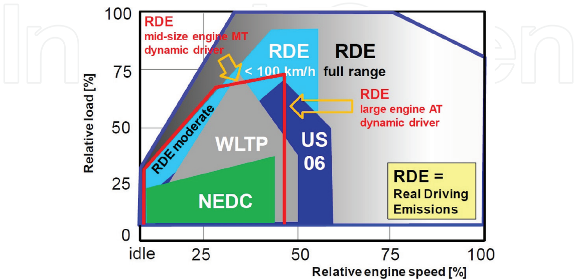
Figure 6. Engine parameters in different emission tests [22].
