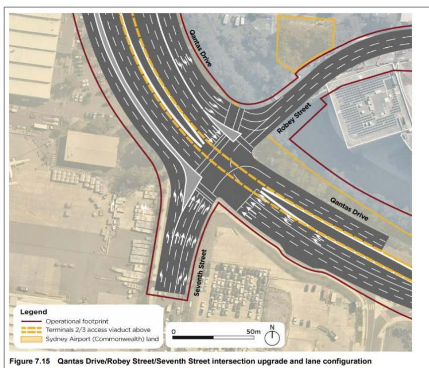
Figure 3 - Proposed Intersection Layout - Terminals 2/3 Egress
