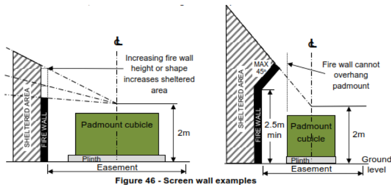
Figure 46 - Screen wall examples
