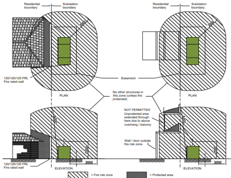
Figure 47 - Typical effect of screen walls
