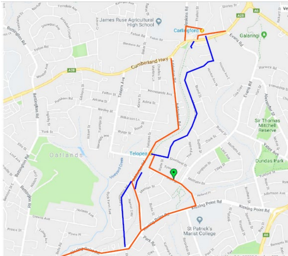
Figure 6-4 Identified Haulage Routes - Portion 2 (Main access via Adderton, Cumberland Highway and Kissing Point Rd/Sturt St)
