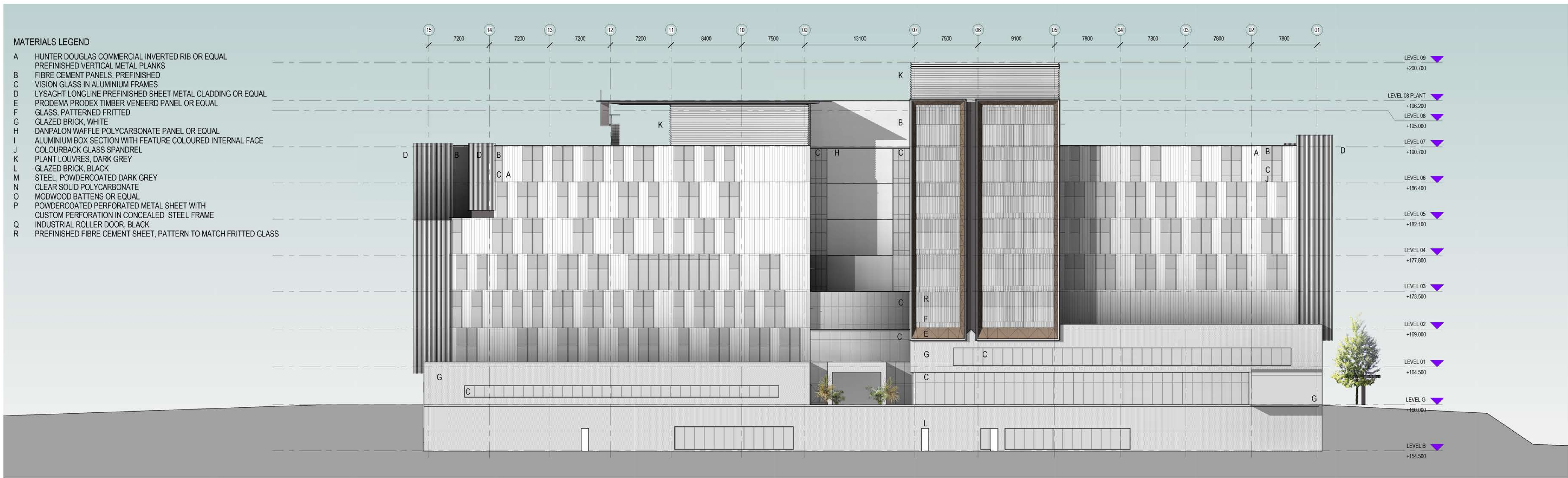
EAST ELEVATION
