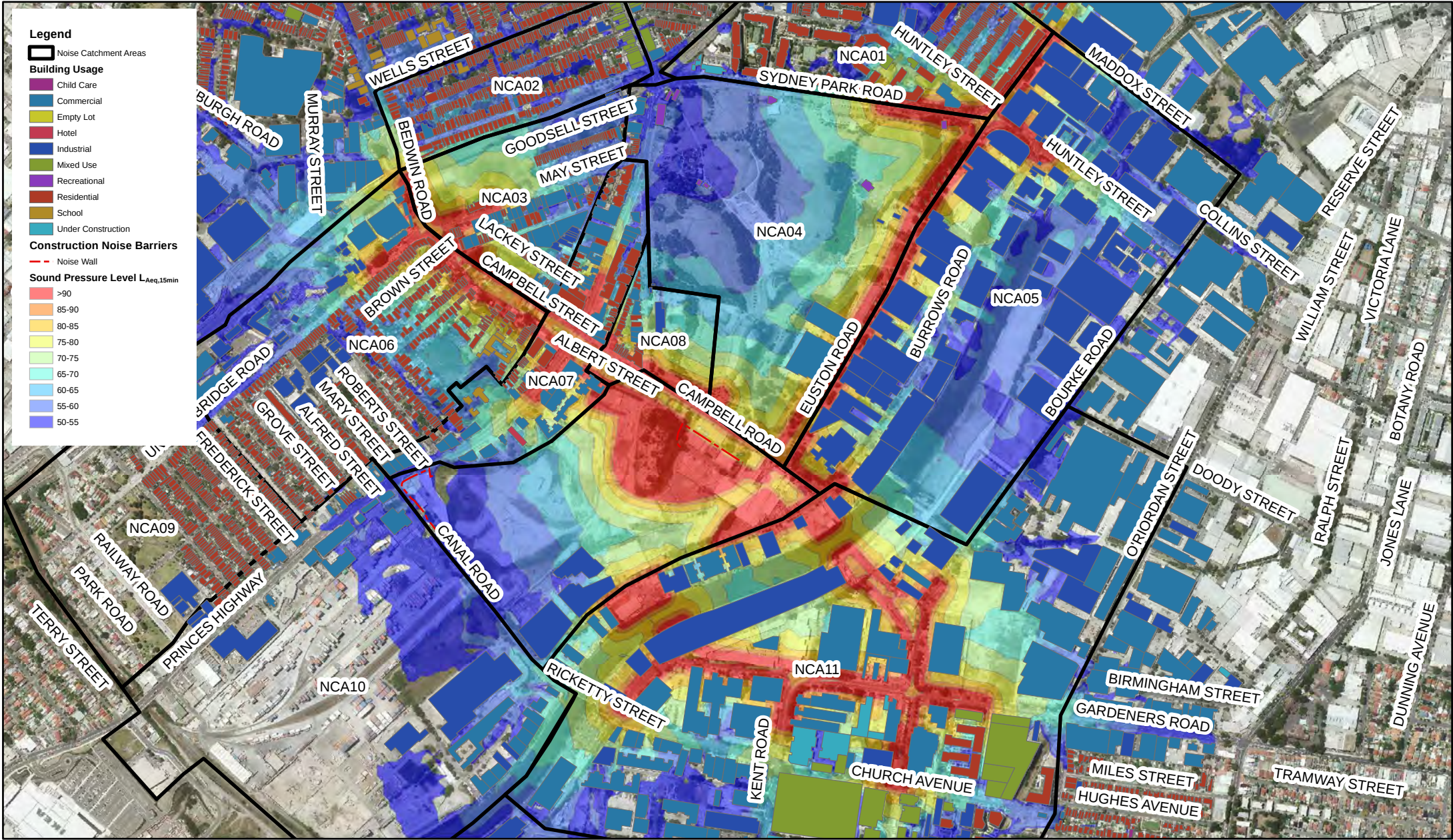
WestConnex Stage 2 - Construction Noise Assessment Surface works - Local road works including construction of the Alexandra Canal Bridge - Earthworks (No rock hammering) - Day
