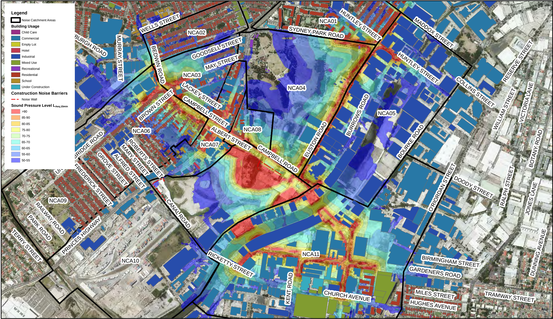
WestConnex Stage 2 - Construction Noise Assessment Surface works - Local road works including construction of the Alexandra Canal Bridge - Road tie-in works - Day
