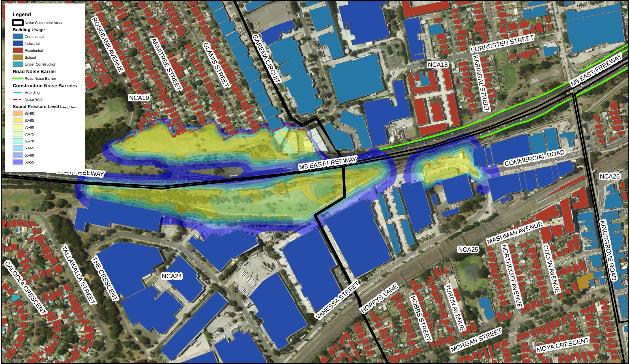
WestConnex Stage 2 - Construction Noise Assessment Tunnelling works - Site establishment - Power Generator - Day
