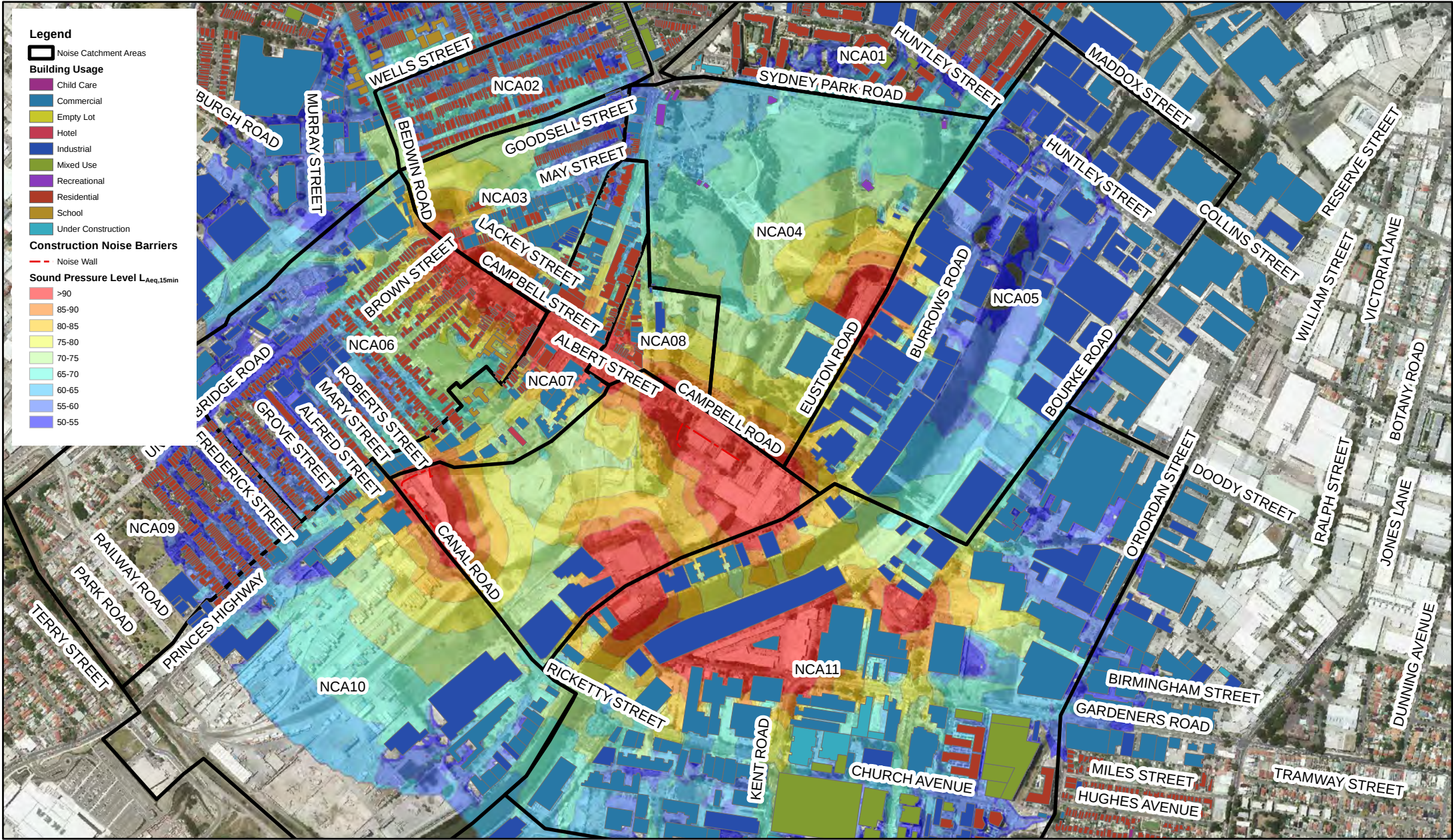
WestConnex Stage 2 - Construction Noise Assessment Surface works - Local road works including construction of the Alexandra Canal Bridge - Demolition of existing structures (Rock hammering only) - Day
