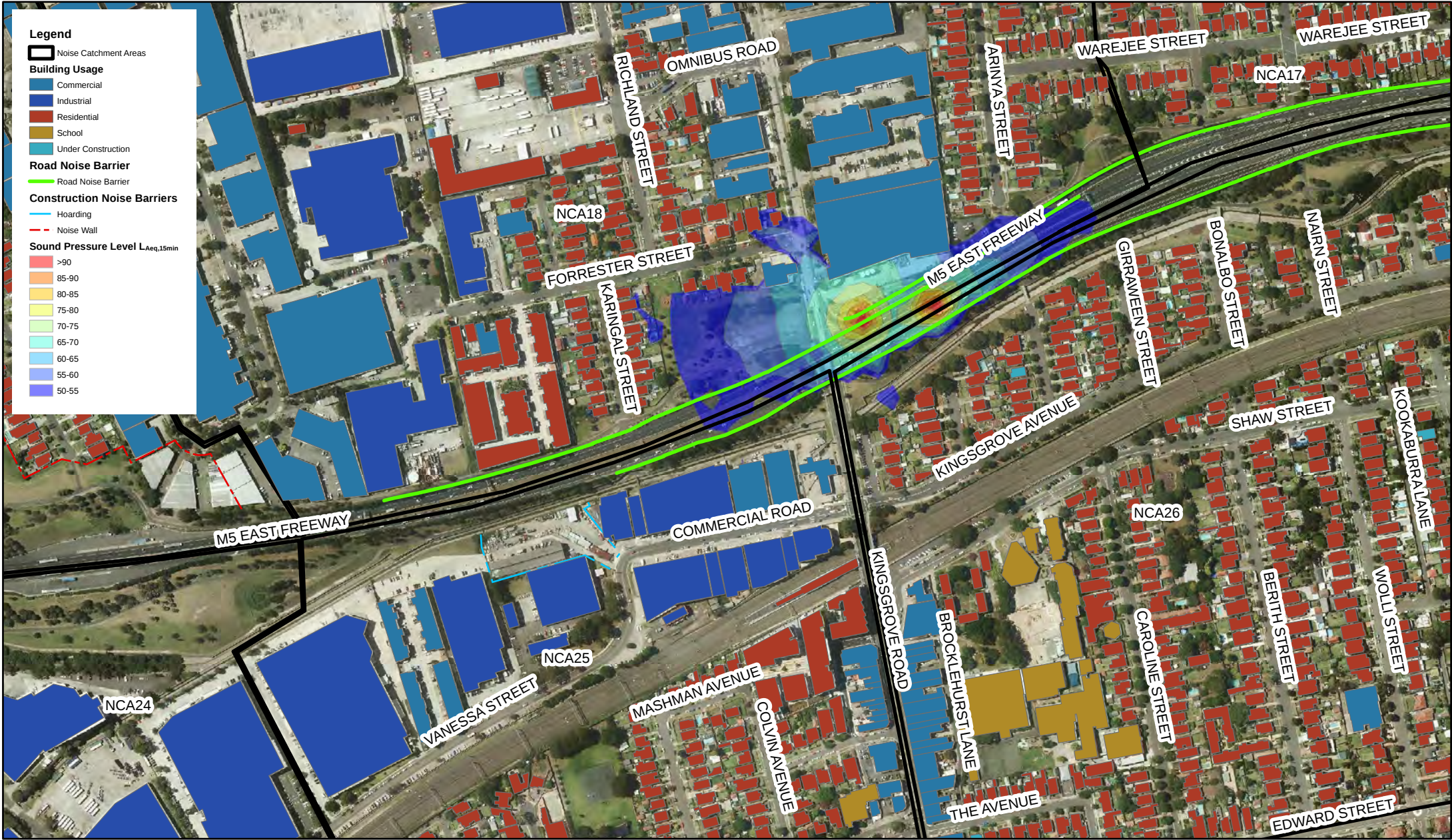
WestConnex Stage 2 - Construction Noise Assessment Surface works - Tolling infrastructure - Site establishment - Day
