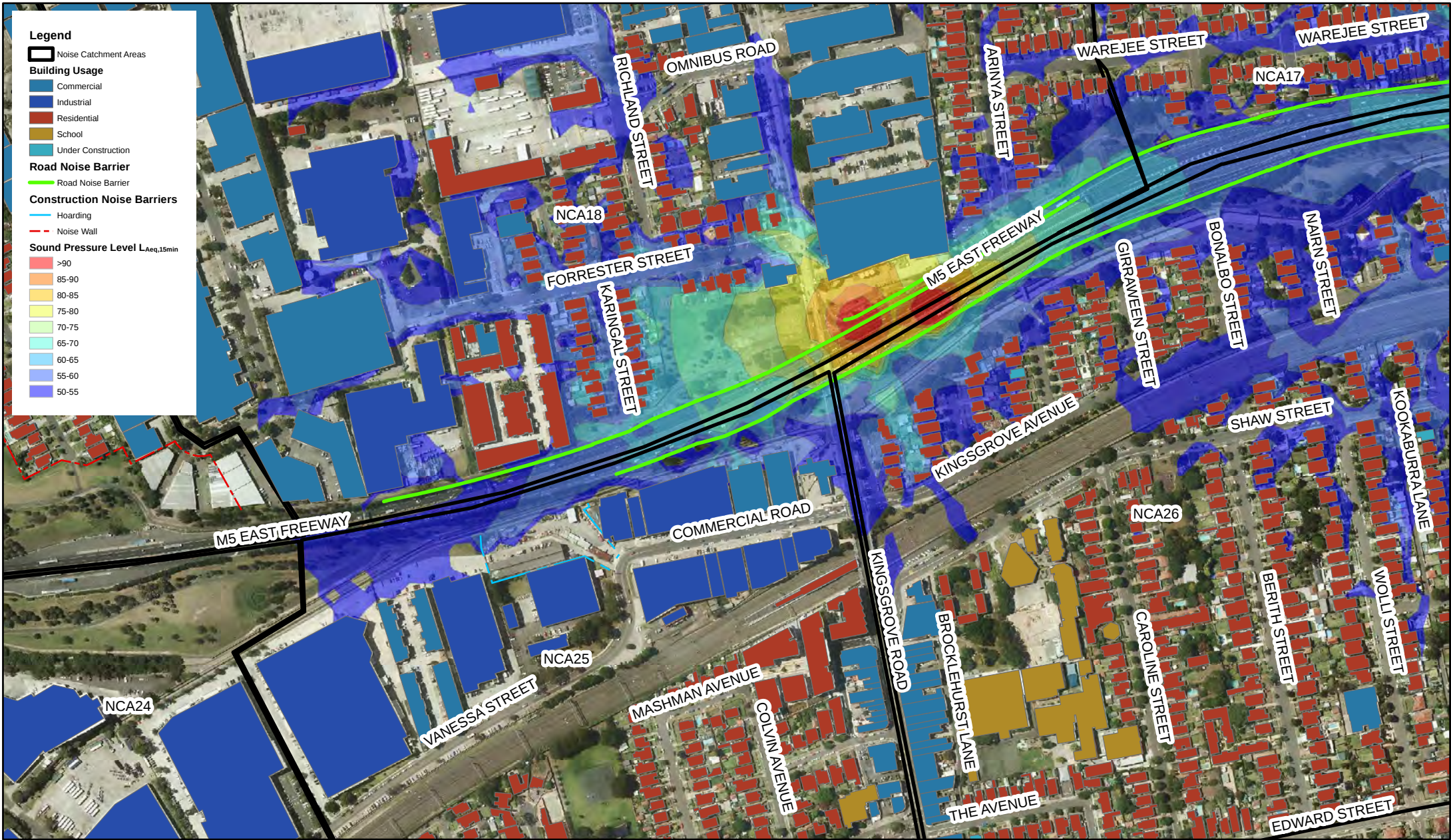
WestConnex Stage 2 - Construction Noise Assessment Surface works - Tolling infrastructure - Road works - Day
