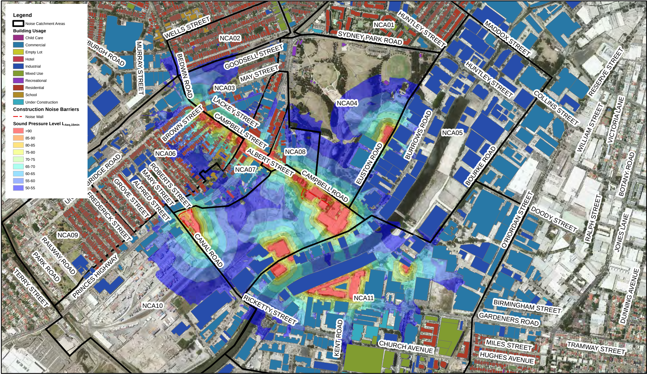
WestConnex Stage 2 - Construction Noise Assessment Surface works - Local road works including construction of the Alexandra Canal Bridge - Demolition of existing structures (No rock hammering) - Day
