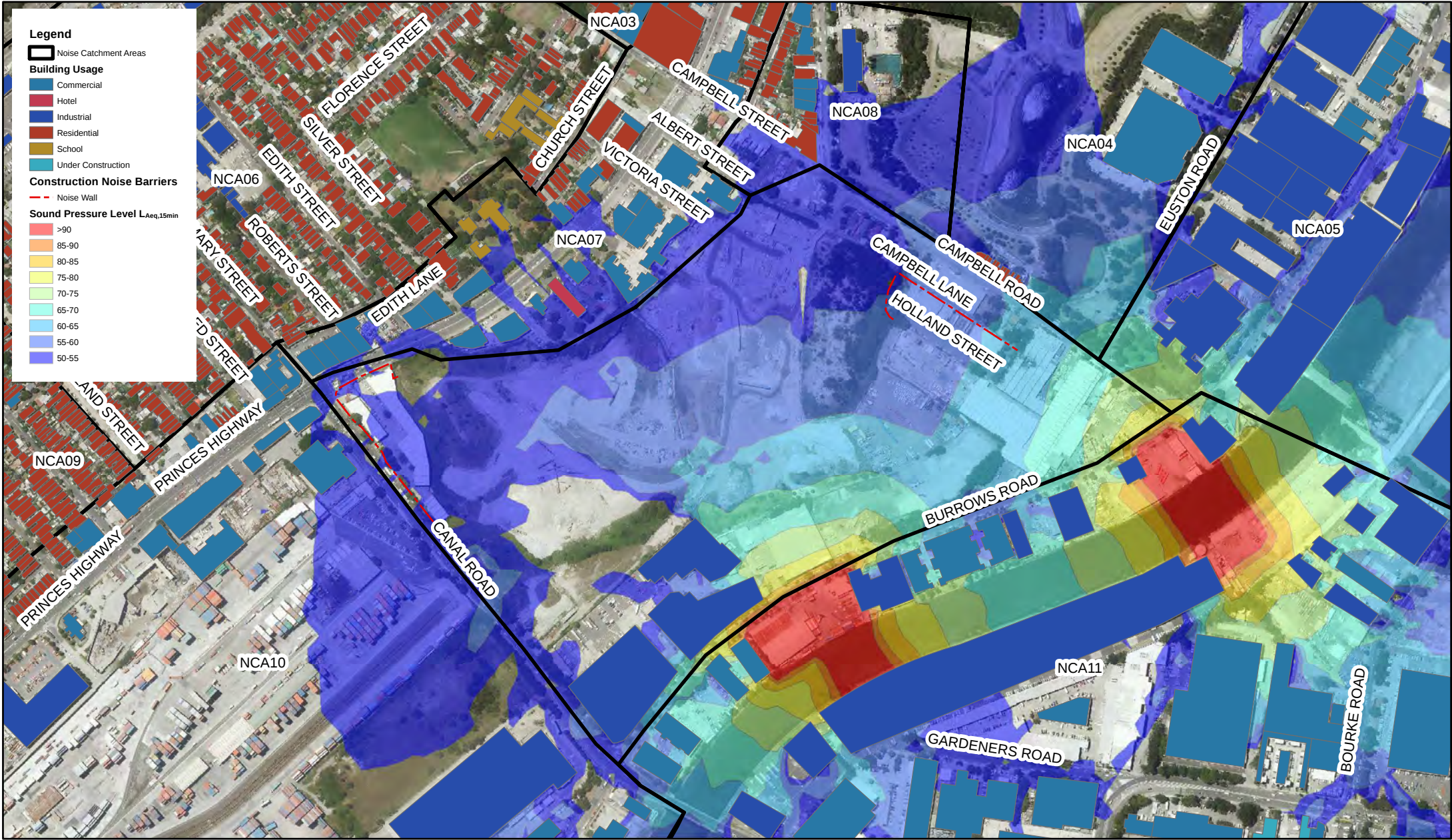
WestConnex Stage 2 - Construction Noise Assessment Surface works - Local road works including construction of the Alexandra Canal Bridge - Alexandra Canal Bridge - Day
