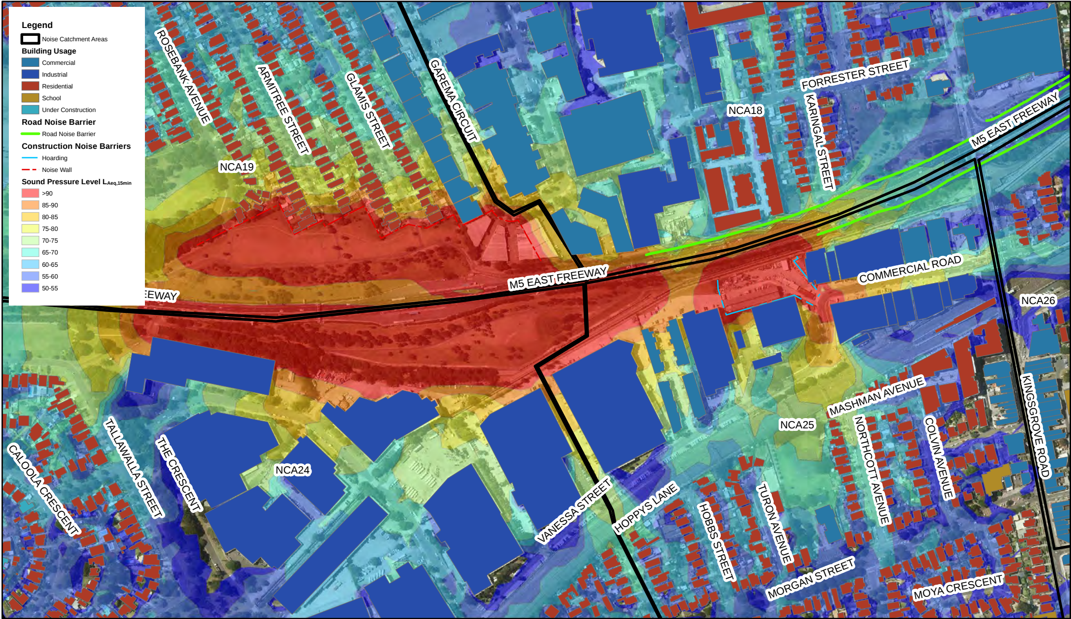
WestConnex Stage 2 - Construction Noise Assessment Surface works - General utility installation and relocation - Service installation and relocation - Day
