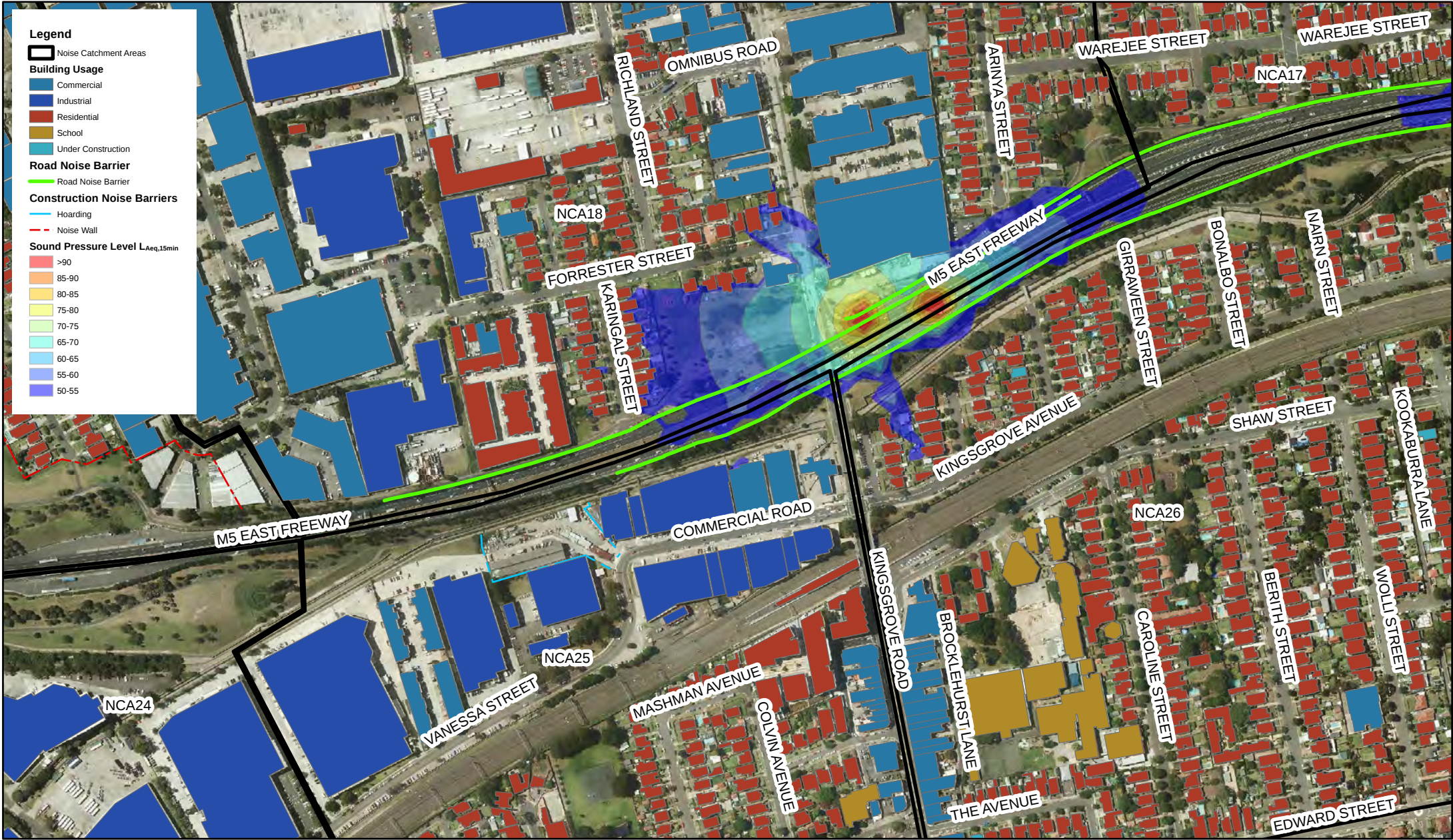
WestConnex Stage 2 - Construction Noise Assessment Surface works - Tolling infrastructure - Construction of toll gantries - Day
