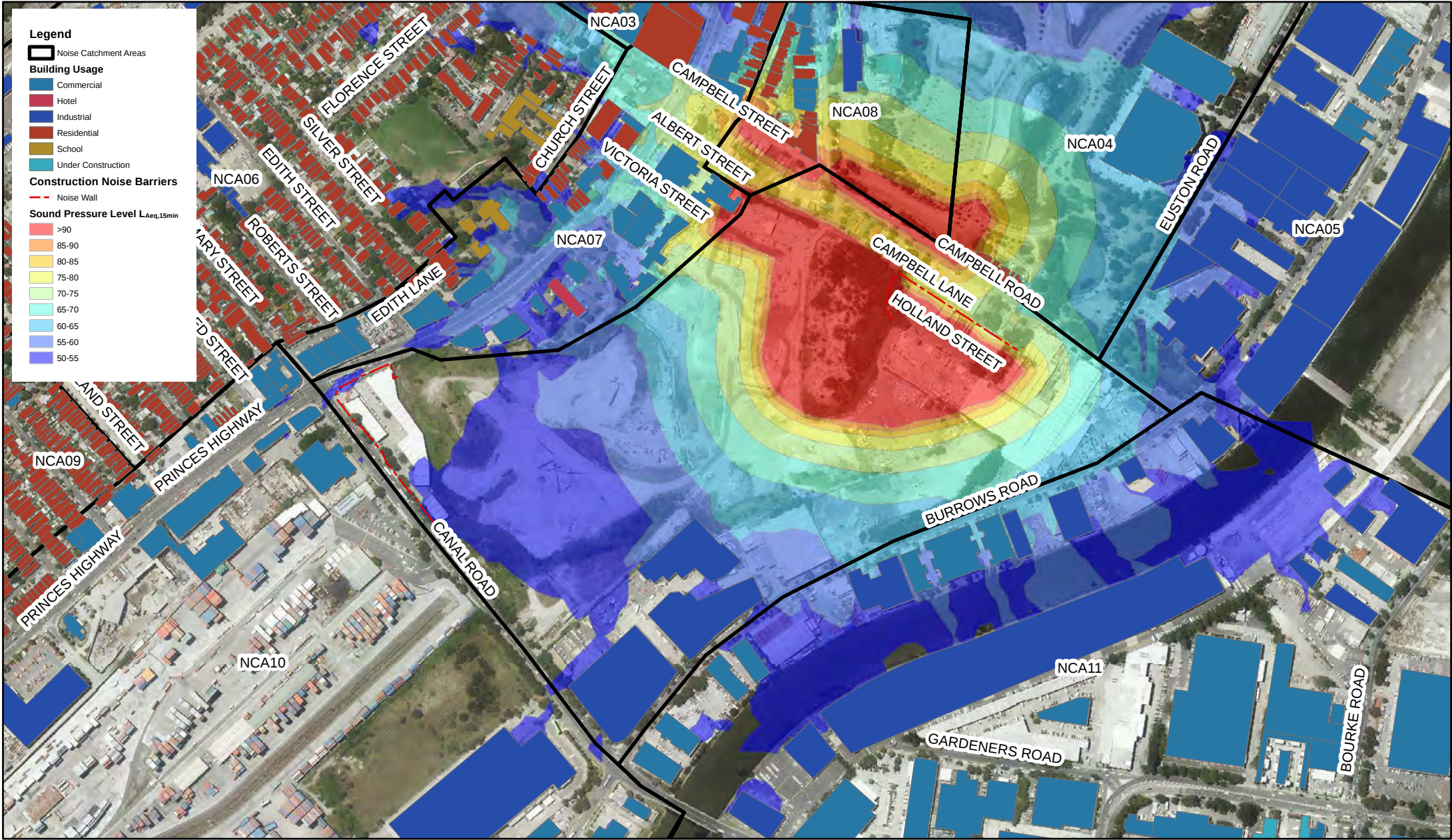
WestConnex Stage 2 - Construction Noise Assessment Surface works - Local road works including construction of the Alexandra Canal Bridge - Pedestrian bridges to Campbell Rd - Day
