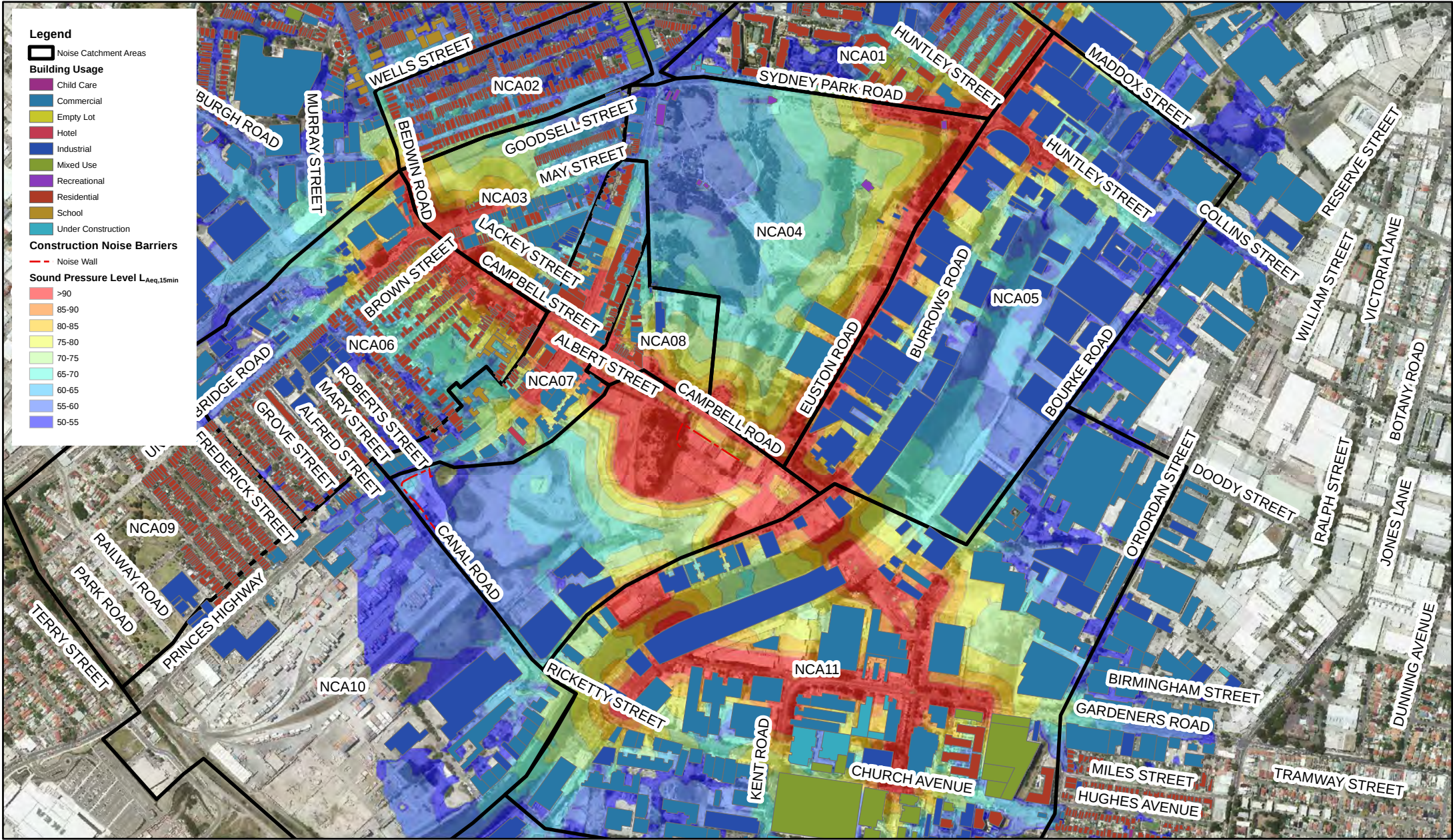
WestConnex Stage 2 - Construction Noise Assessment Surface works - Local road works including construction of the Alexandra Canal Bridge - Kerbing and drainage - Day
