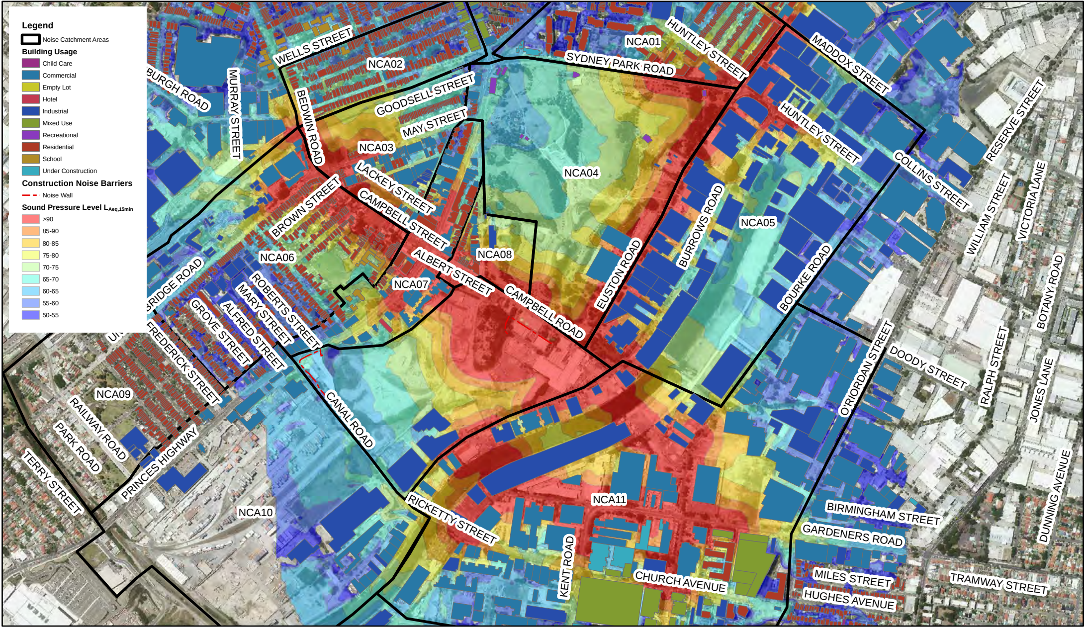
WestConnex Stage 2 - Construction Noise Assessment Surface works - Local road works including construction of the Alexandra Canal Bridge - Earthworks (Rock hammering only) - Day
