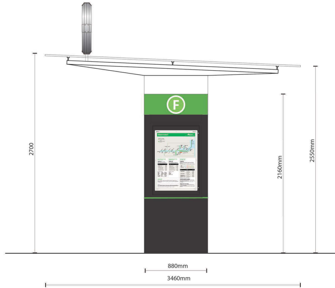
SIDE ELEVATION
