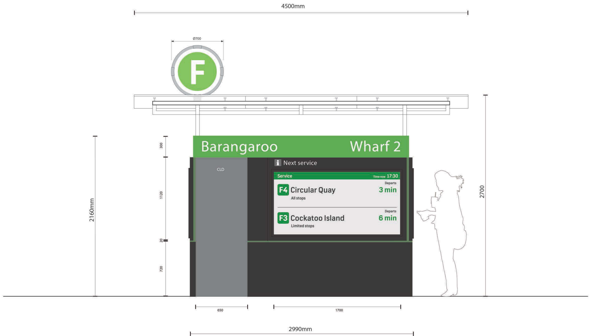
FRONT ELEVATION
