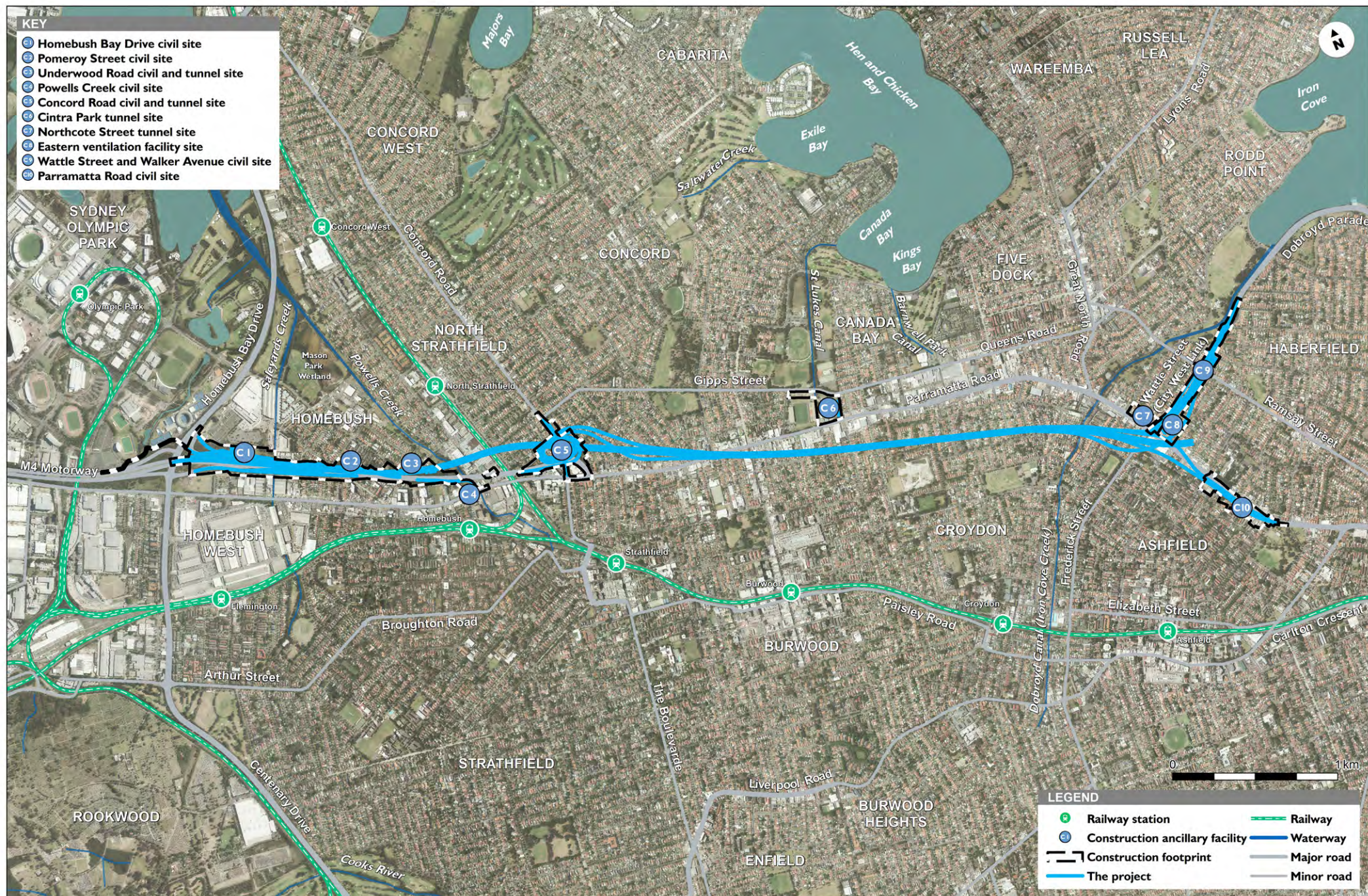
Figure 2.2 Overview of construction footprint and construction ancillary facilities
