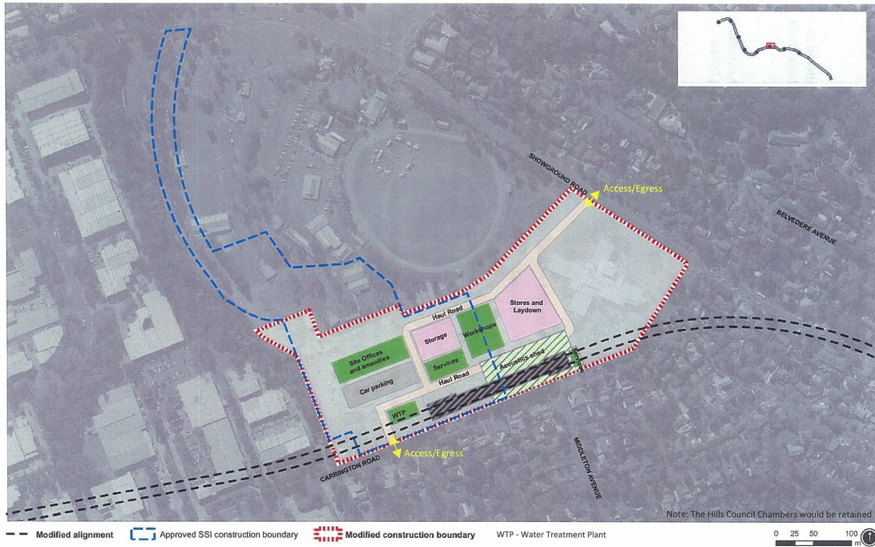
Figure 4-2: Proposed Modification to the Construction Site Boundary and Site Layout
