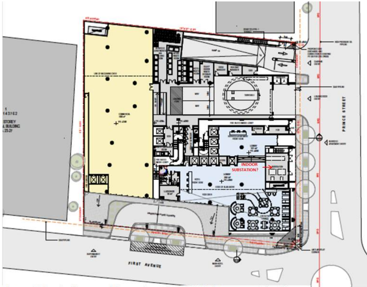
Figure 5: Typical ground floor plan at 17-21 First Avenue, Blacktown
