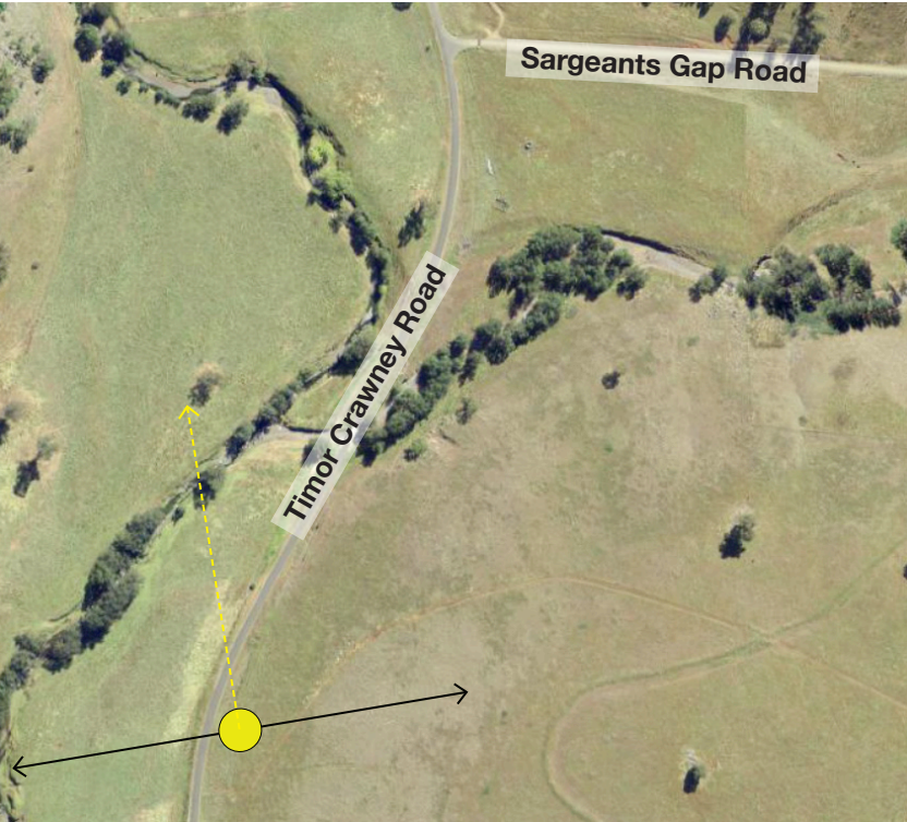
Figure D10B Photomontage Location Aerial image - Source: Six Maps
