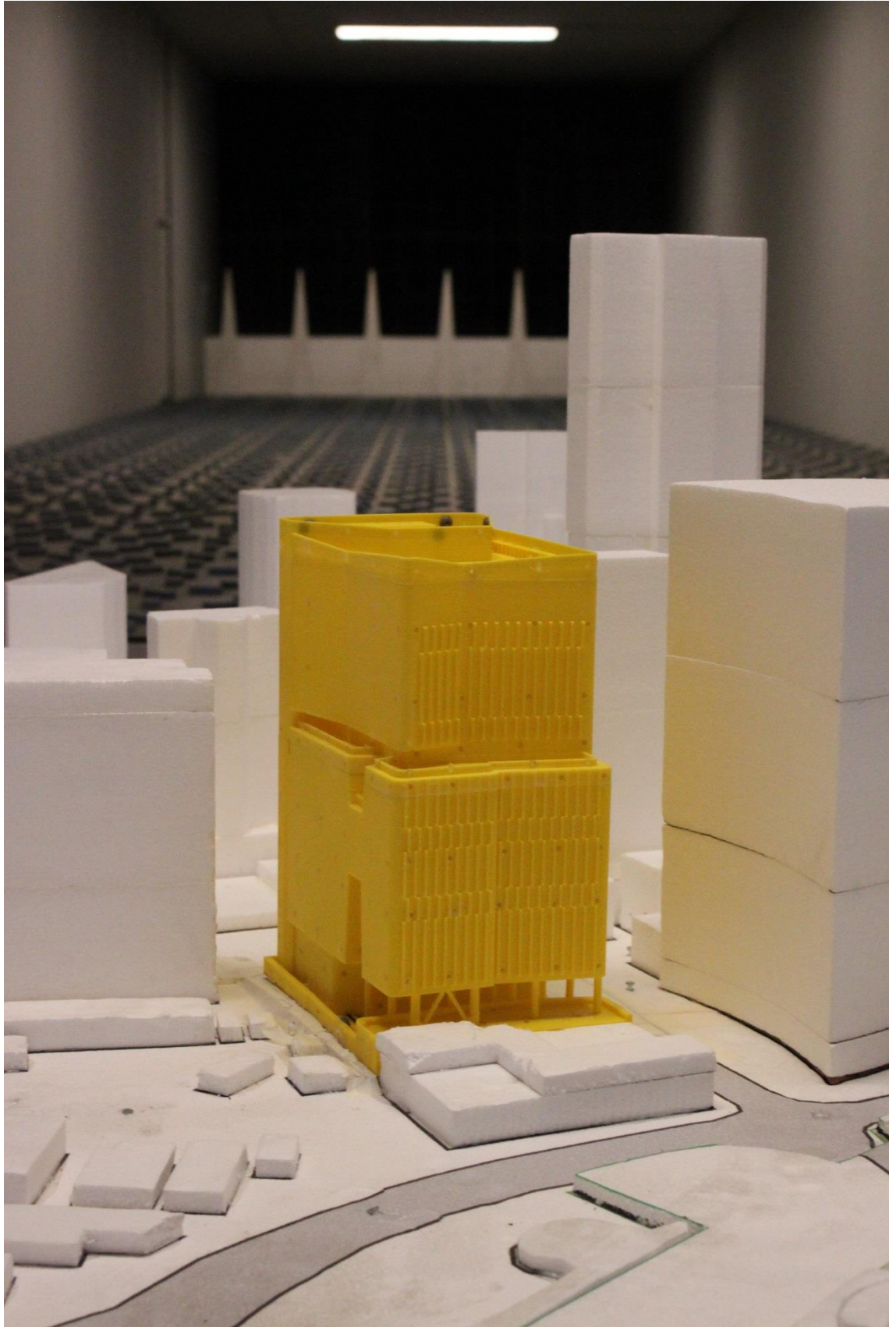
Figure 1e: Photograph of the Wind Tunnel Model (view from the west)
