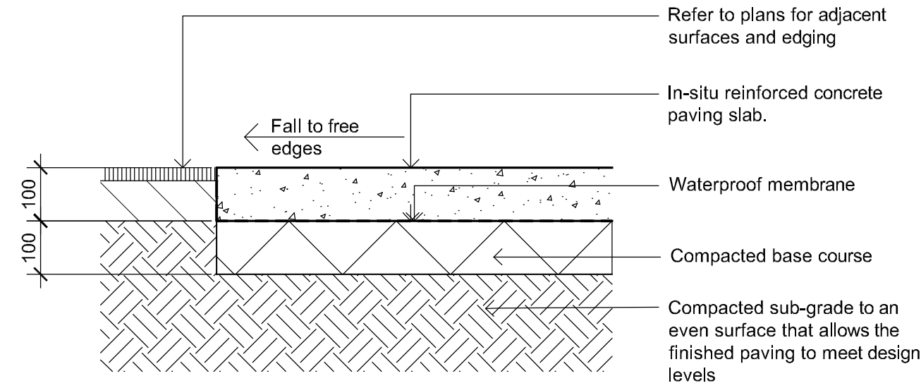
05 Insitu Concrete Paving - On grade 501 1:10
