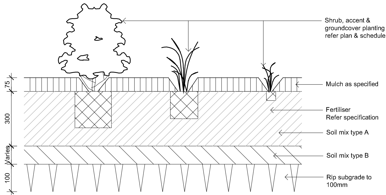
03 Detail Shrub Accent & Groundcover Planting on Grade 501 1:10
