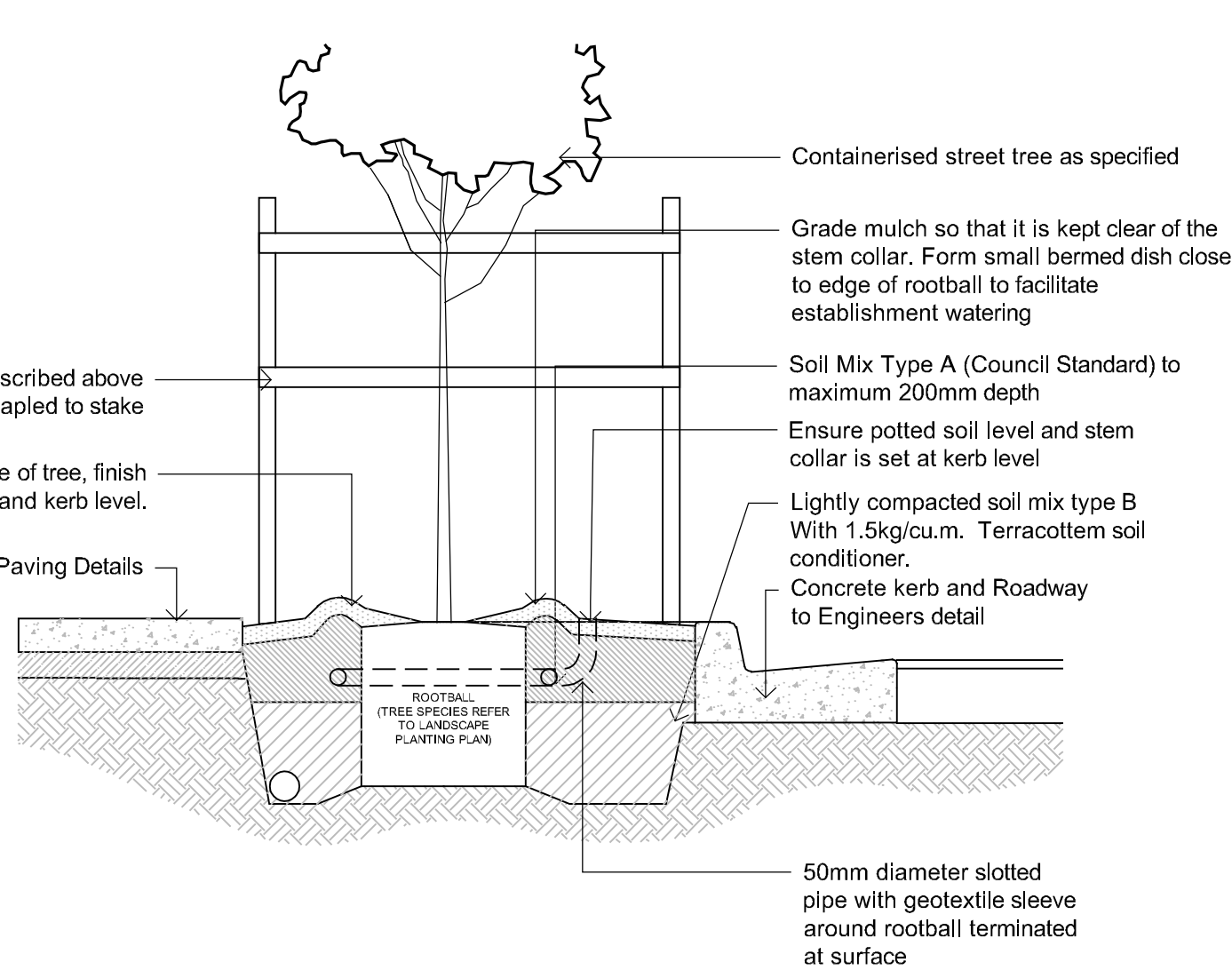
06 TREE PLANTING IN FOOTPATH AND SECTION 501 1:20
