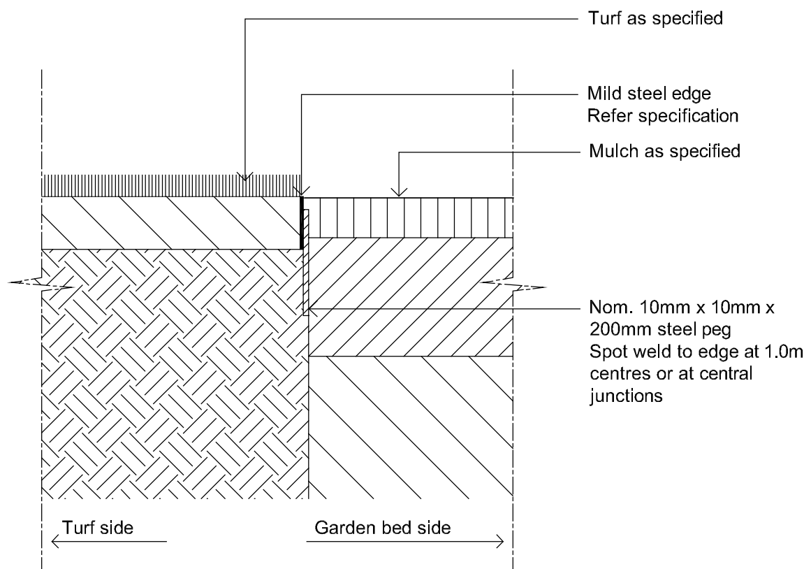
04 TYPICAL MILD STEEL EDGE 501 SCALE 1:10
