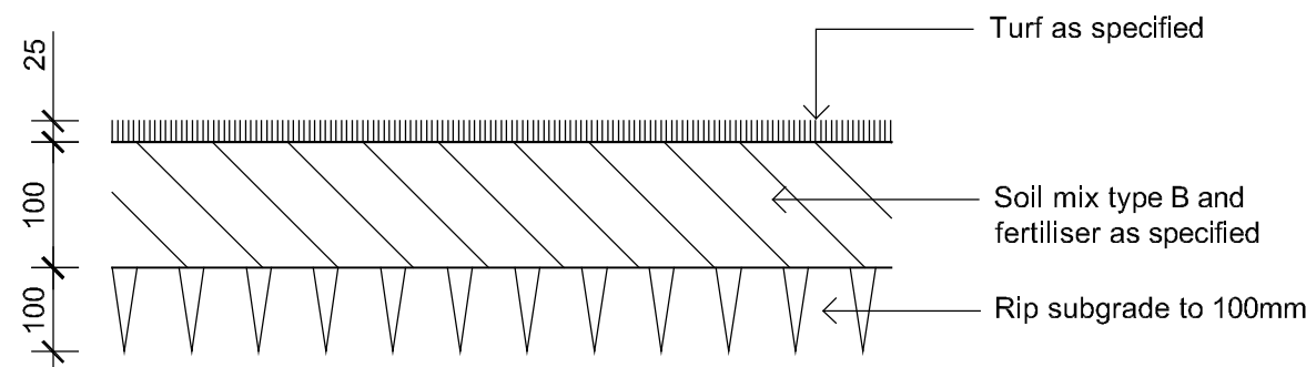
02 Detail Turf on Even Grade 501 1:10
