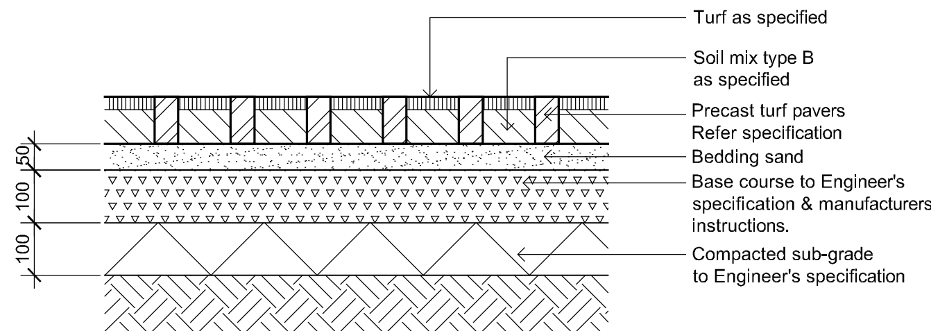
07 TURF PAVERS ON GRADE 501 SCALE 1:10
