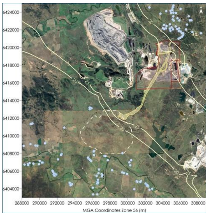
Figure E-6: Predicted annual average PM 10 concentrations due to emissions from the Project and other sources in Scenario 1 (µg/m 3 )
