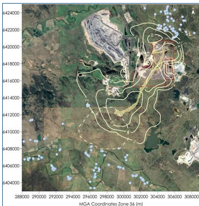
Figure E-4: Predicted maximum 24-hour average PM_{10} concentrations due to emissions from the Project in Scenario 1 ( \mu g/m^3 )
