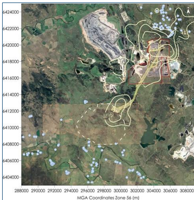
Figure E-35: Predicted 1-hour average \text{NO}_2 concentrations due to emissions from the Project in Scenario 3 ( \mu\text{g}/\text{m}^3 ) (hypothetical 100% conversion of \text{NO}_x to \text{NO}_2 )
