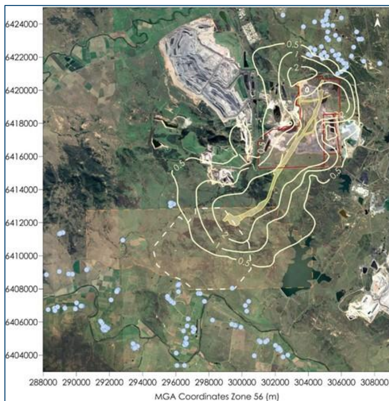
Figure E-1: Predicted maximum 24-hour average PM_{2.5} concentrations due to emissions from the Project in Scenario 1 ( \mu g/m^3 )
