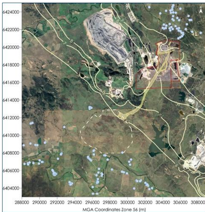
Figure E-23: Predicted annual average PM_{2.5} concentrations due to emissions from the Project and other sources in Scenario 3 ( \mu g/m^3 )
