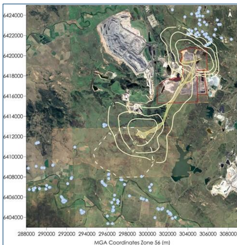
Figure E-14: Predicted maximum 24-hour average PM_{10} concentrations due to emissions from the Project in Scenario 2 ( \mu g/m^3 )
