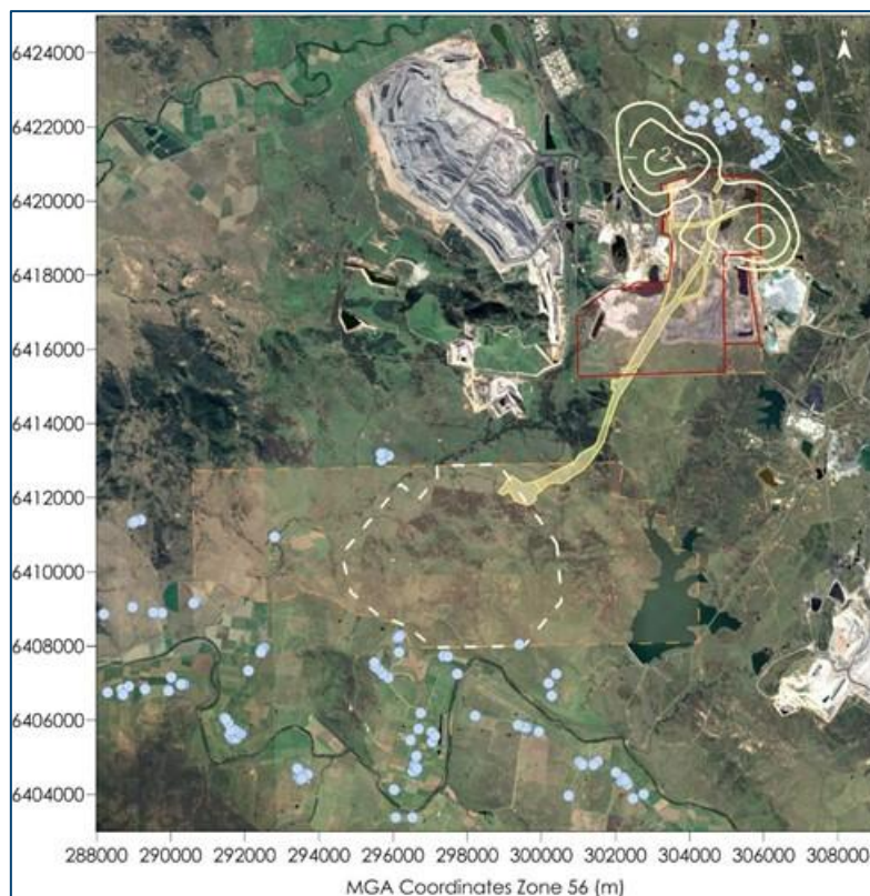
Figure E-36: Predicted annual average \text{NO}_2 concentrations due to emissions from the Project in Scenario 3 ( \mu\text{g}/\text{m}^3 ) (hypothetical 100% conversion of \text{NO}_x to \text{NO}_2 )
