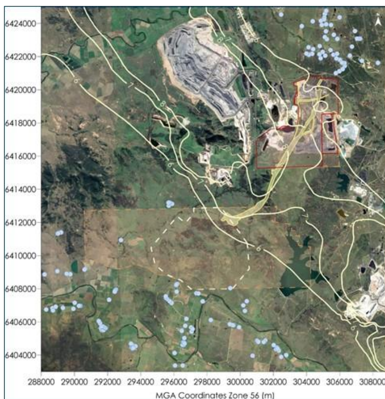
Figure E-3: Predicted annual average PM_{2.5} concentrations due to emissions from the Project and other sources in Scenario 1 ( \mu g/m^3 )
