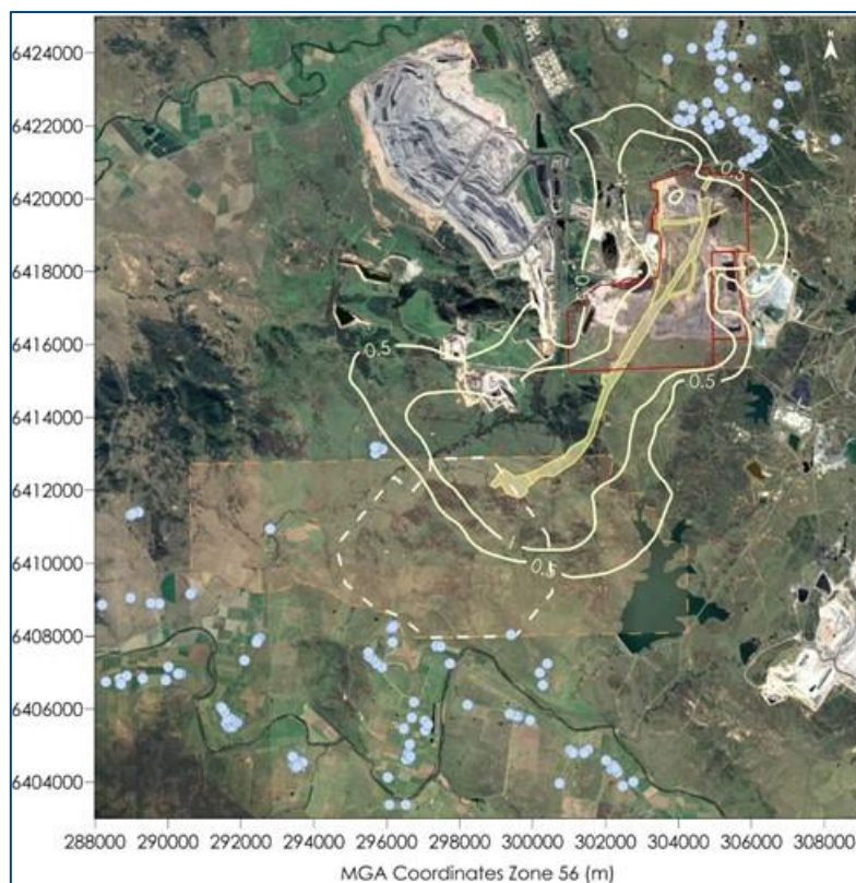
Figure E-5: Predicted annual average PM 10 concentrations due to emissions from the Project in Scenario 1 (µg/m 3 )
