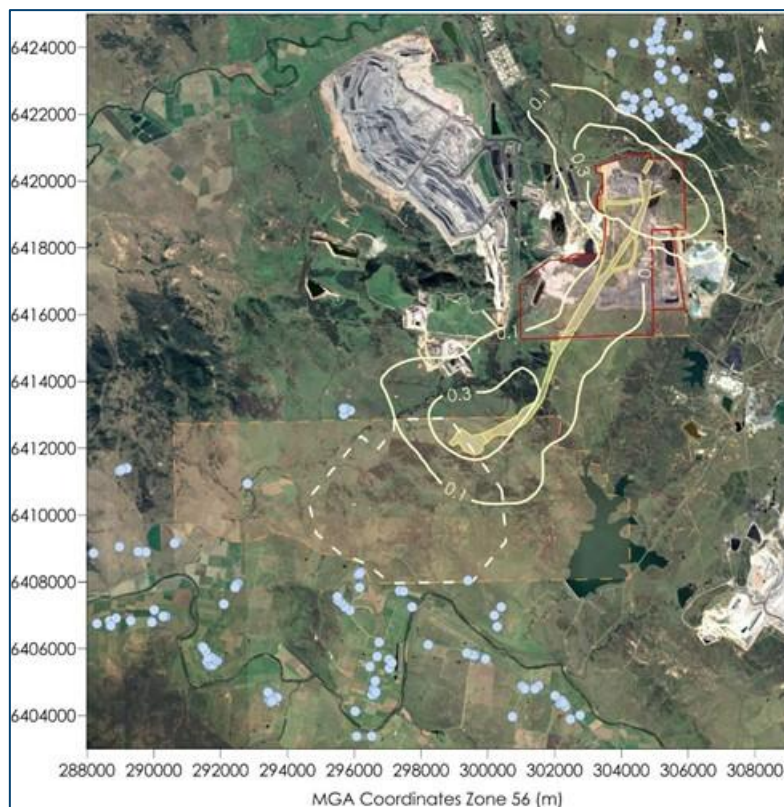
Figure E-12: Predicted annual average PM 2.5 concentrations due to emissions from the Project in Scenario 2 (µg/m 3 )
