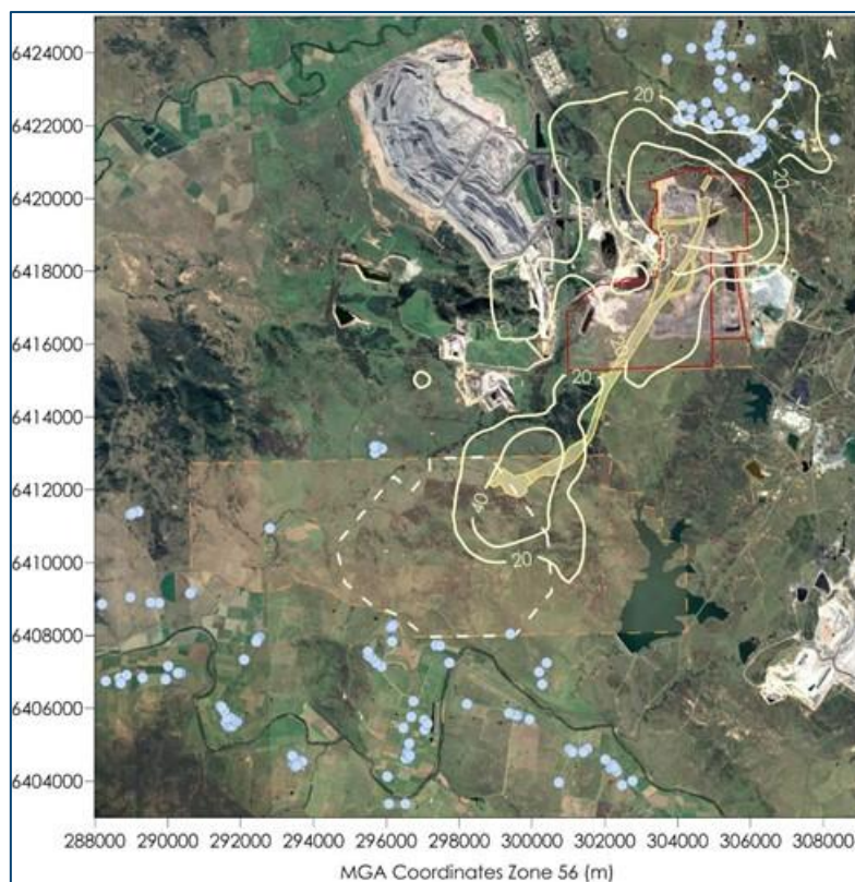
Figure E-33: Predicted 1-hour average NO 2 concentrations due to emissions from the Project in Scenario 2 (µg/m 3 ) (hypothetical 100% conversion of NO x to NO 2 )
