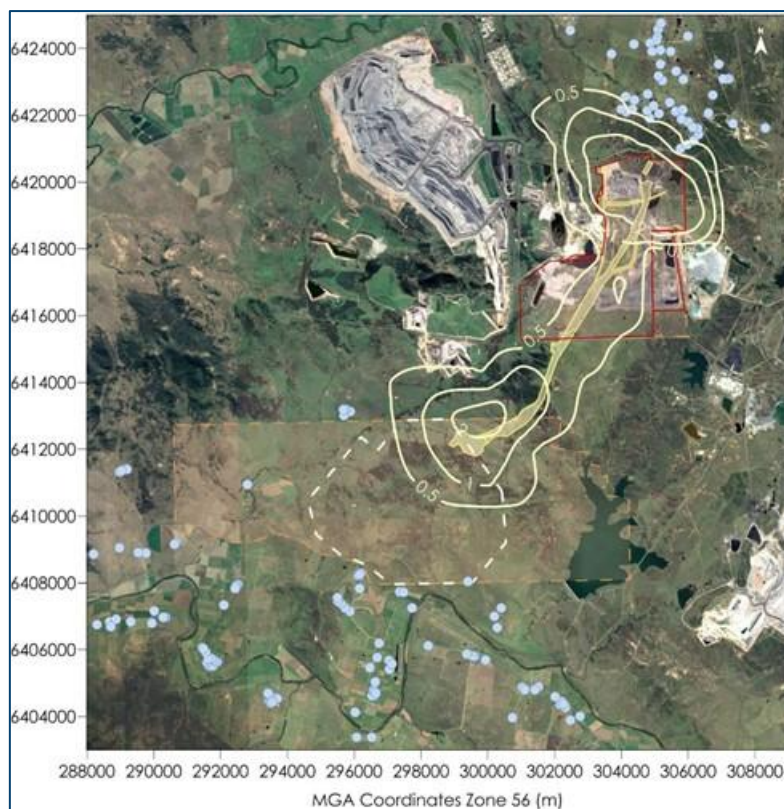
Figure E-11: Predicted maximum 24-hour average PM 2.5 concentrations due to emissions from the Project in Scenario 2 (µg/m 3 )
