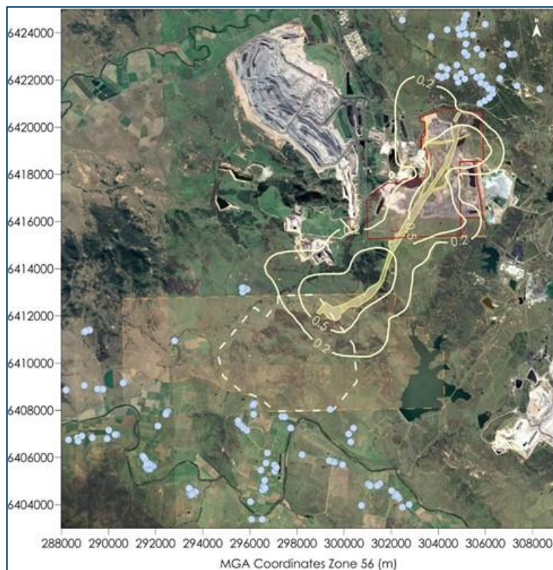
Figure E-2: Predicted annual average PM_{2.5} concentrations due to emissions from the Project in Scenario 1 ( \mu g/m^3 )
