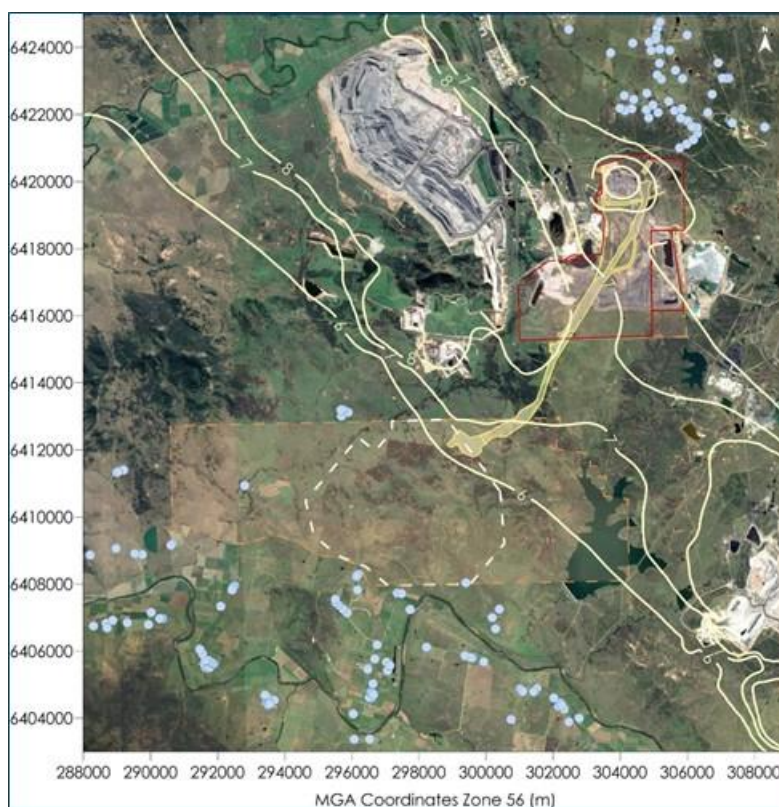
Figure E-13: Predicted annual average PM_{2.5} concentrations due to emissions from the Project and other sources in Scenario 2 ( \mu g/m^3 )
