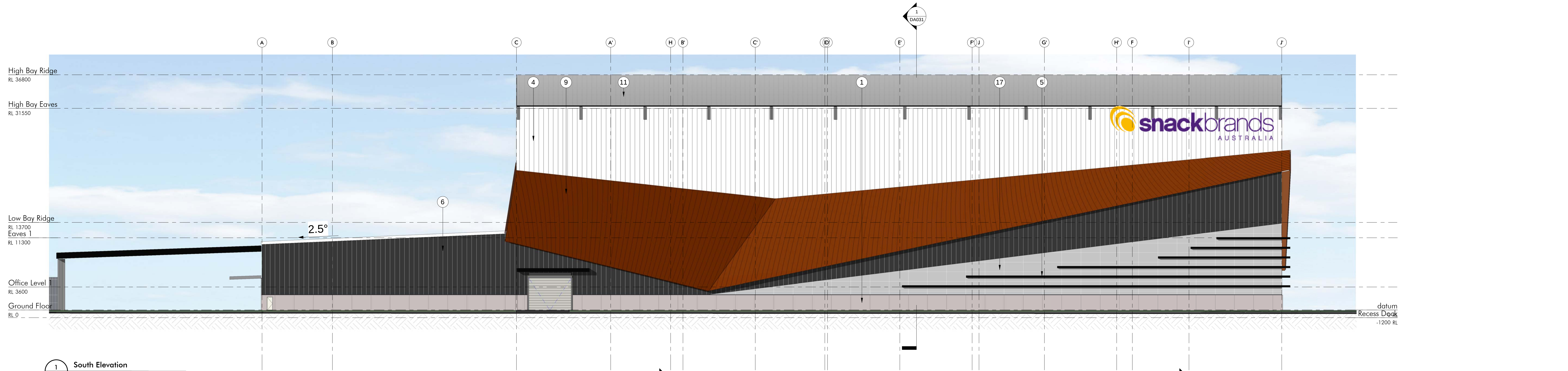
1 South Elevation 1 : 250
