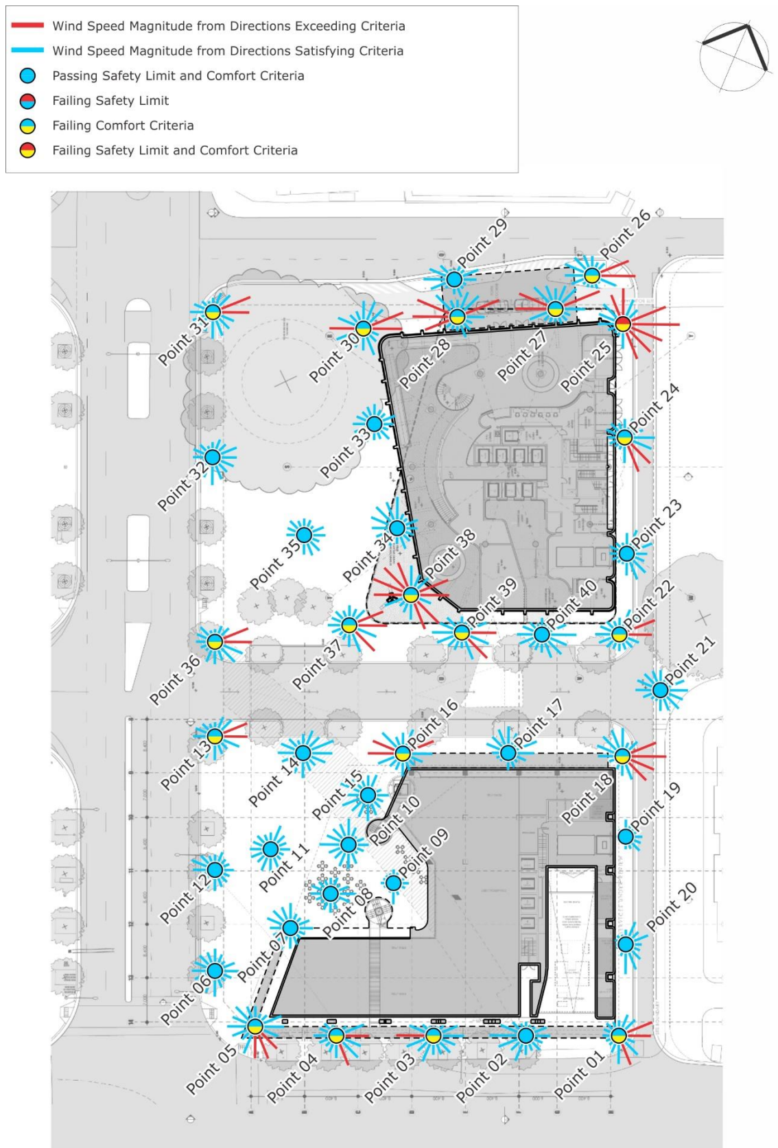
Figure 6: Wind Tunnel Results – Ground Lower and Upper Plans (results shown without treatments applied)
