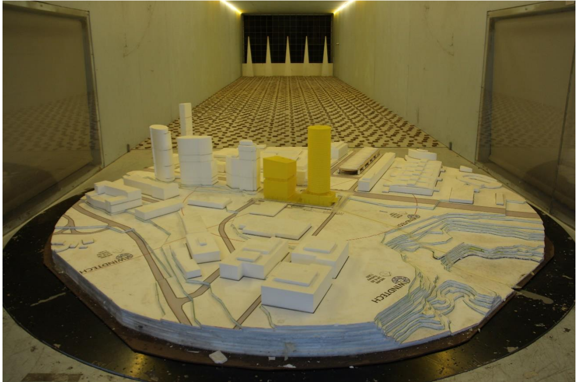
Figure 1b: Photograph of the Wind Tunnel Model – Proposed Surrounds Scenario (view from the north-east)
