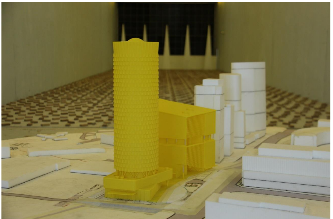
Figure 1e: Photograph of the Wind Tunnel Model – Proposed Surrounds Scenario (view from the north-west)
