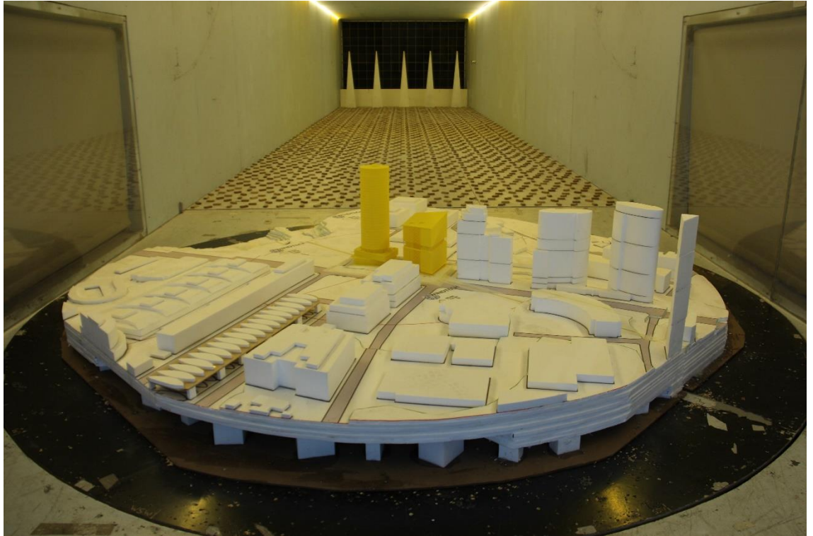
Figure 1d: Photograph of the Wind Tunnel Model – Proposed Surrounds Scenario (view from the south-west)
