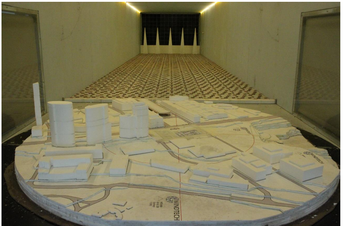
Figure 1g: Photograph of the Wind Tunnel Model – Existing Surrounds Scenario (view from the east)
