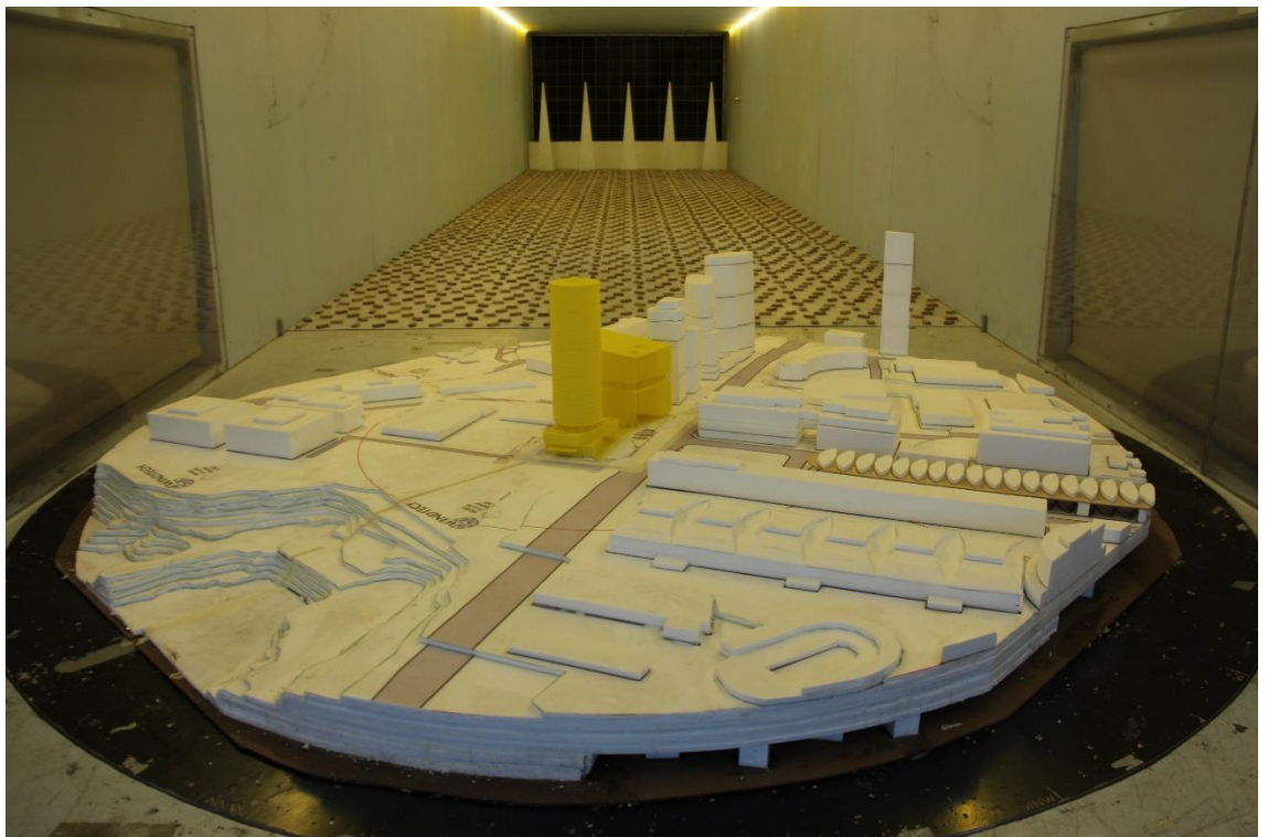
Figure 1c: Photograph of the Wind Tunnel Model – Proposed Surrounds Scenario (view from the north-west)
