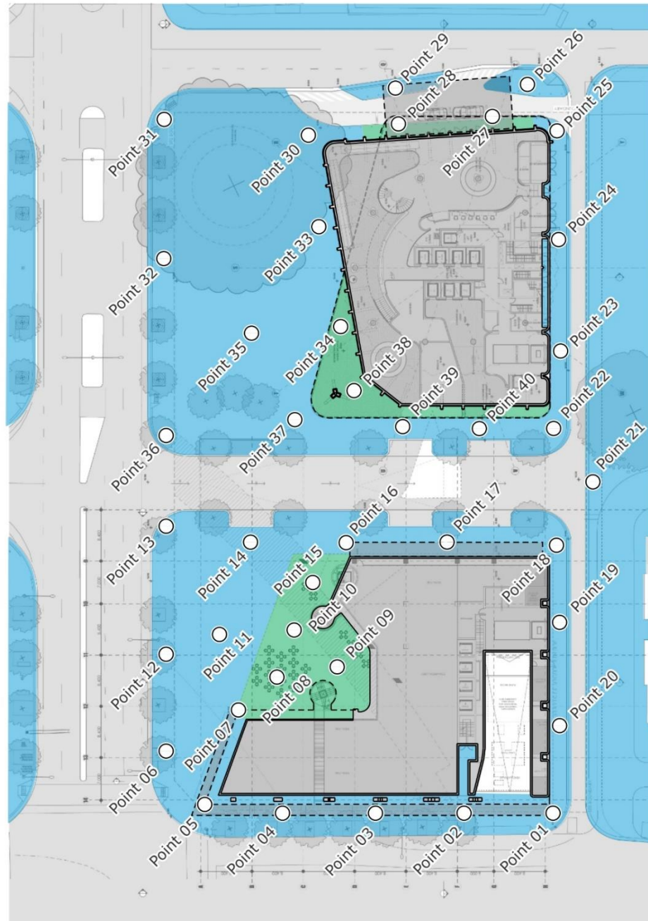
Figure 5: Study Point Locations and Target Wind Speed Criteria Ground Lower and Upper Plans
