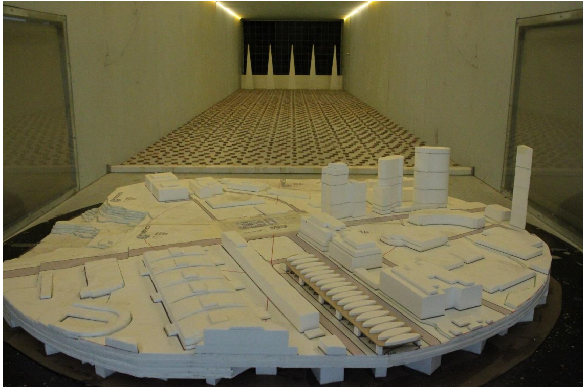
Figure 1f: Photograph of the Wind Tunnel Model – Existing Surrounds Scenario (view from the west)
