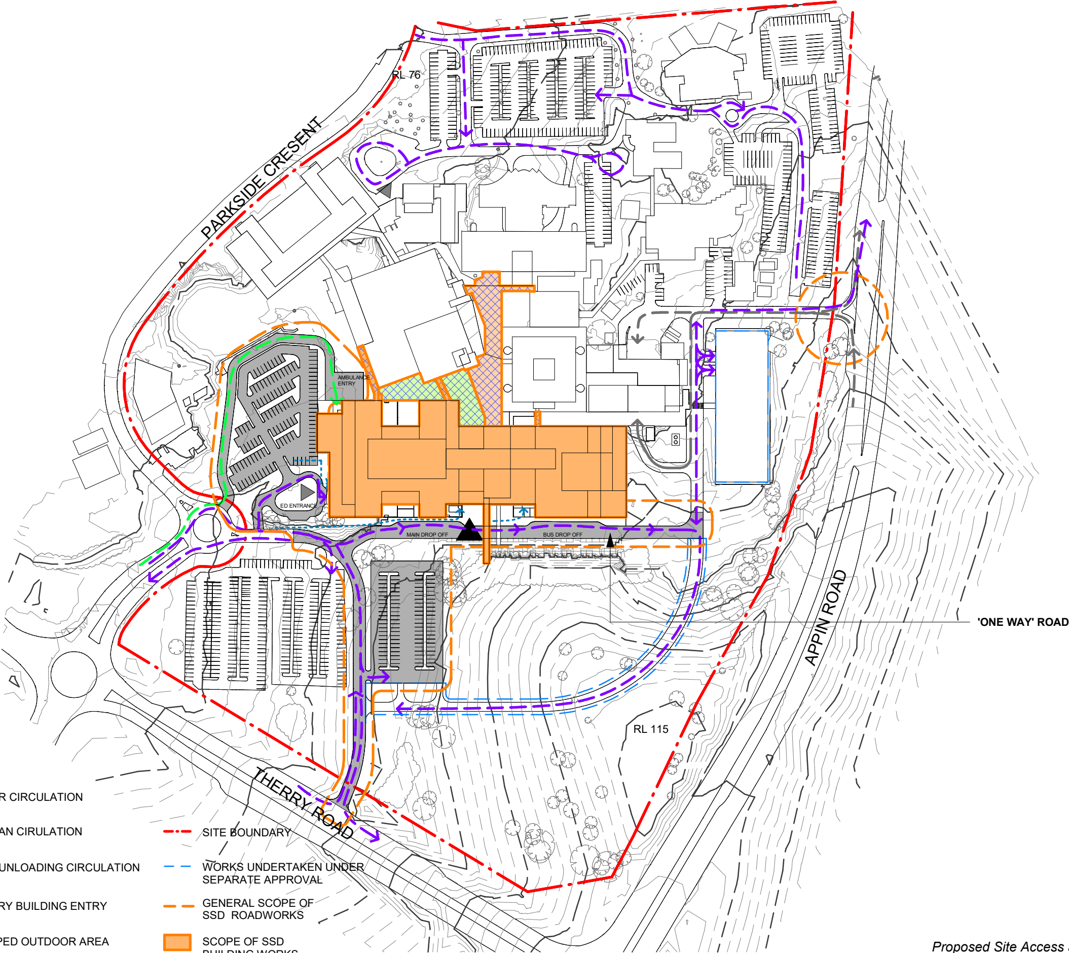
Proposed Site Access and Circulation
