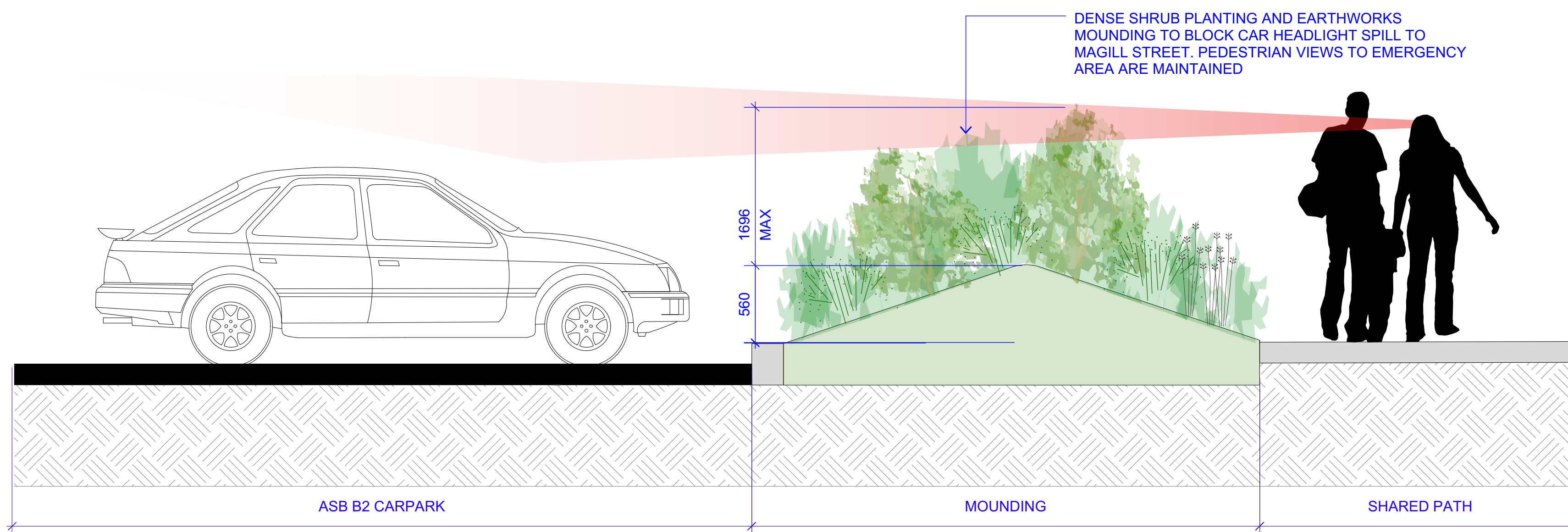
3 ASB BASEMENT 2 | CAR HEADLIGHT SPILL EXTENT DETAIL 1:25 @ A1 or 1:50 @ A3
