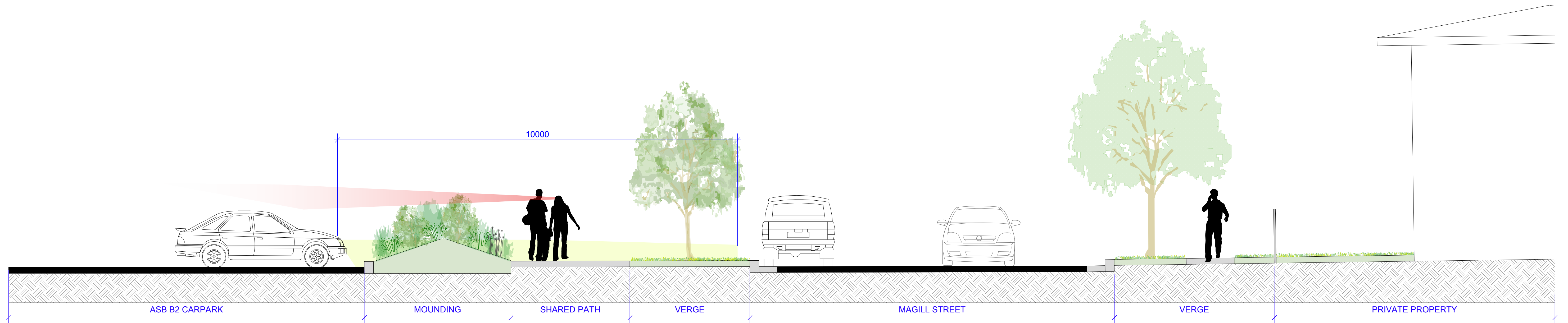
1 ASB BASEMENT 2 | CAR HEADLIGHT SPILL EXTENT 10m 1:50 @ A1 or 1:100 @ A3
