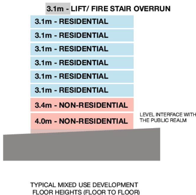
Figure 10: Typical floor to floor heights for mixed use buildings
