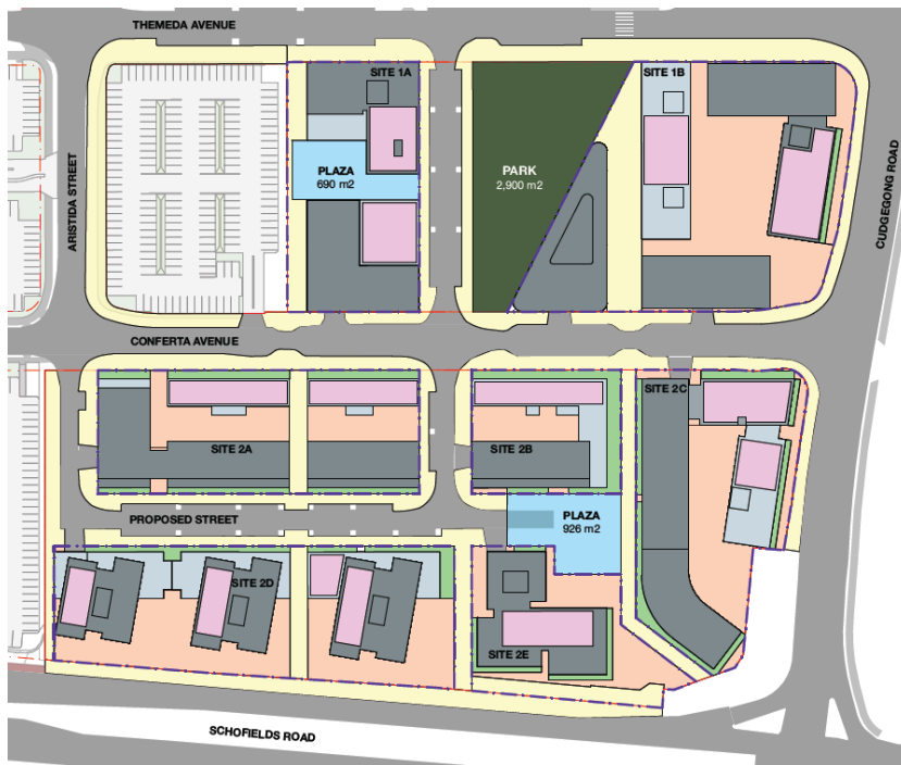
Figure 8: Proposed private open space under Concept Proposal (rooftop gardens coloured pink)
