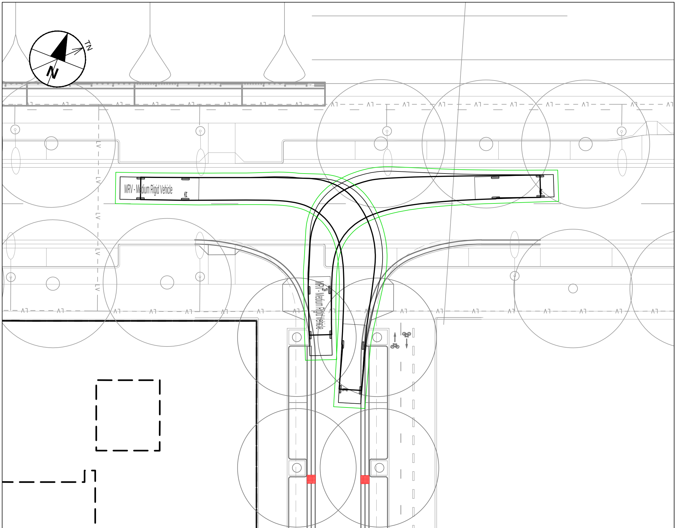
INSET 1 - VEHICLE TRACKING - RIGHT TURNS Scale 1:250
