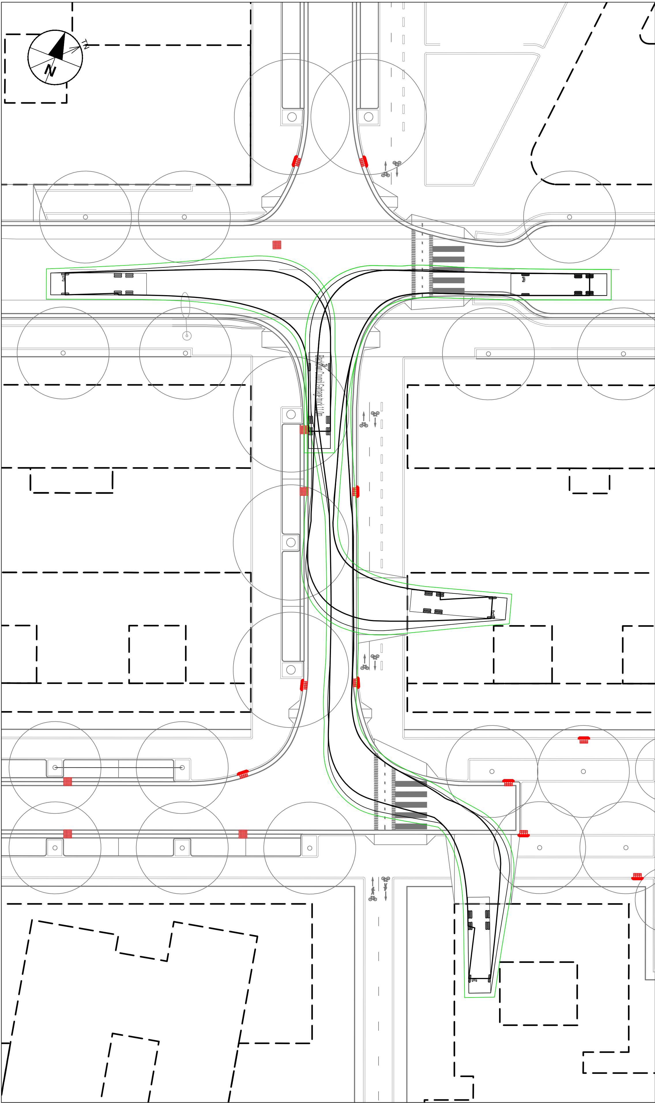
INSET 5 - TURNS INTO BUILDINGS Scale 1:250
