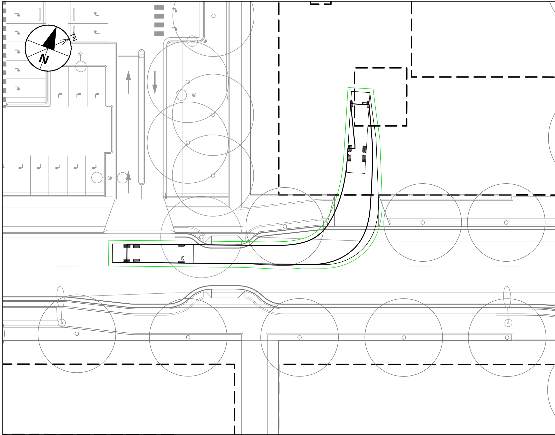
INSET 2 - VEHICLE TRACKING - LEFT TURNS Scale 1:250
