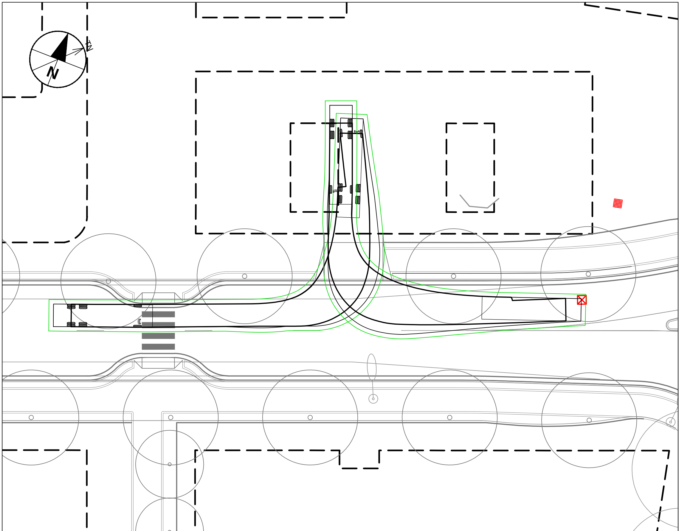
INSET 4 - LEFT TURNS Scale 1:250
