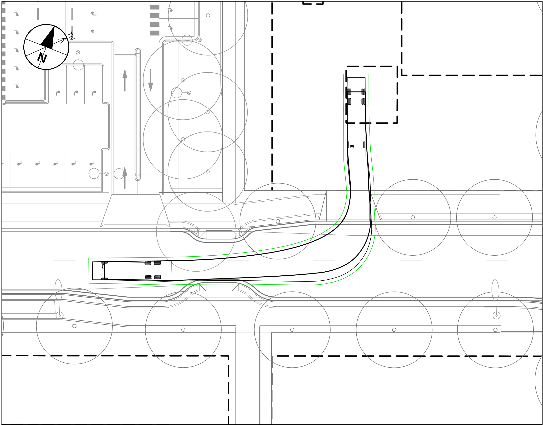
INSET 2 - VEHICLE TRACKING - RIGHT TURNS Scale 1:250
