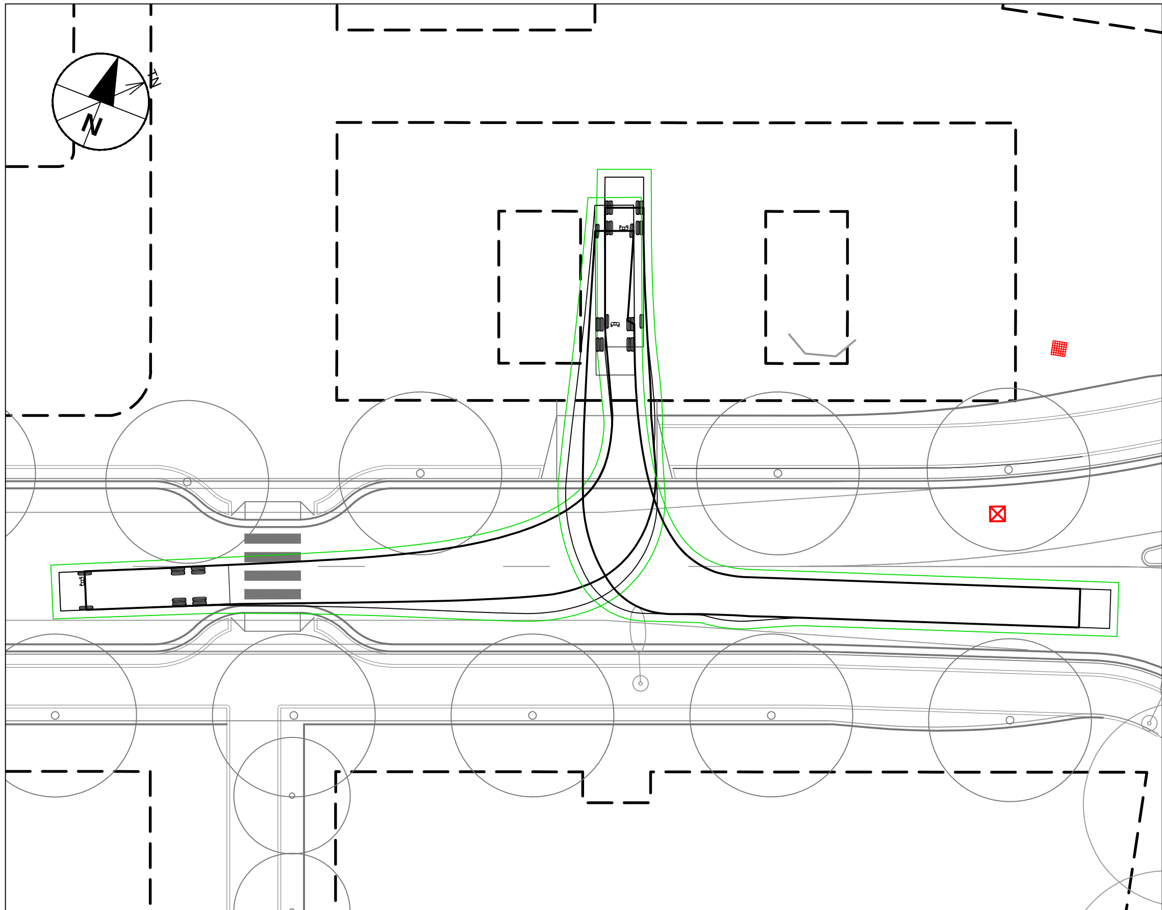
INSET 4 - RIGHT TURNS Scale 1:250
