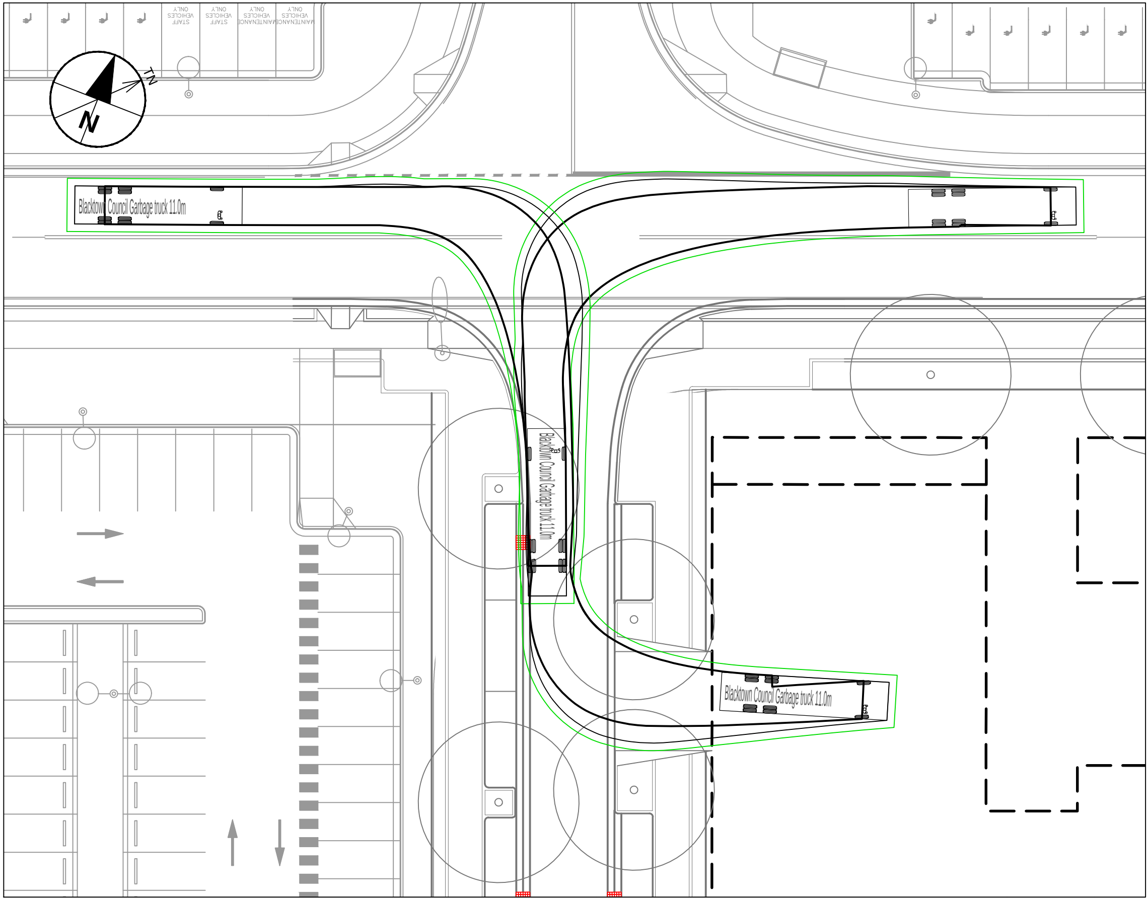
INSET 3 - VEHICLE TRACKING - RIGHT TURNS
