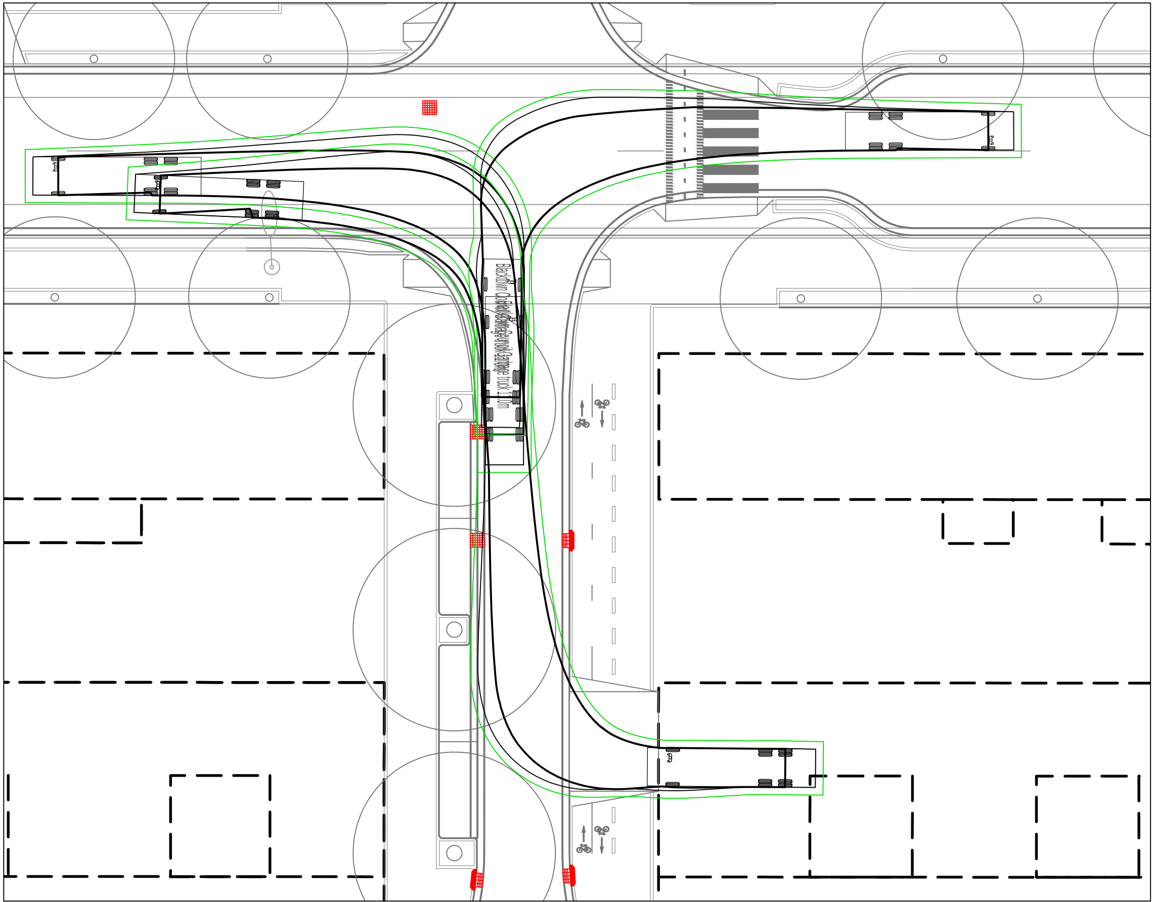
INSET 5 - RIGHT TURN FROM BUILDING Scale 1:250
