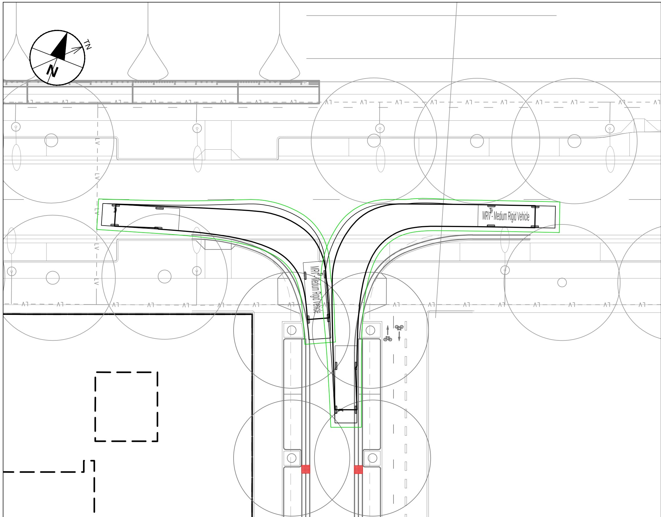
INSET 1 - VEHICLE TRACKING - LEFT TURNS Scale 1:250
