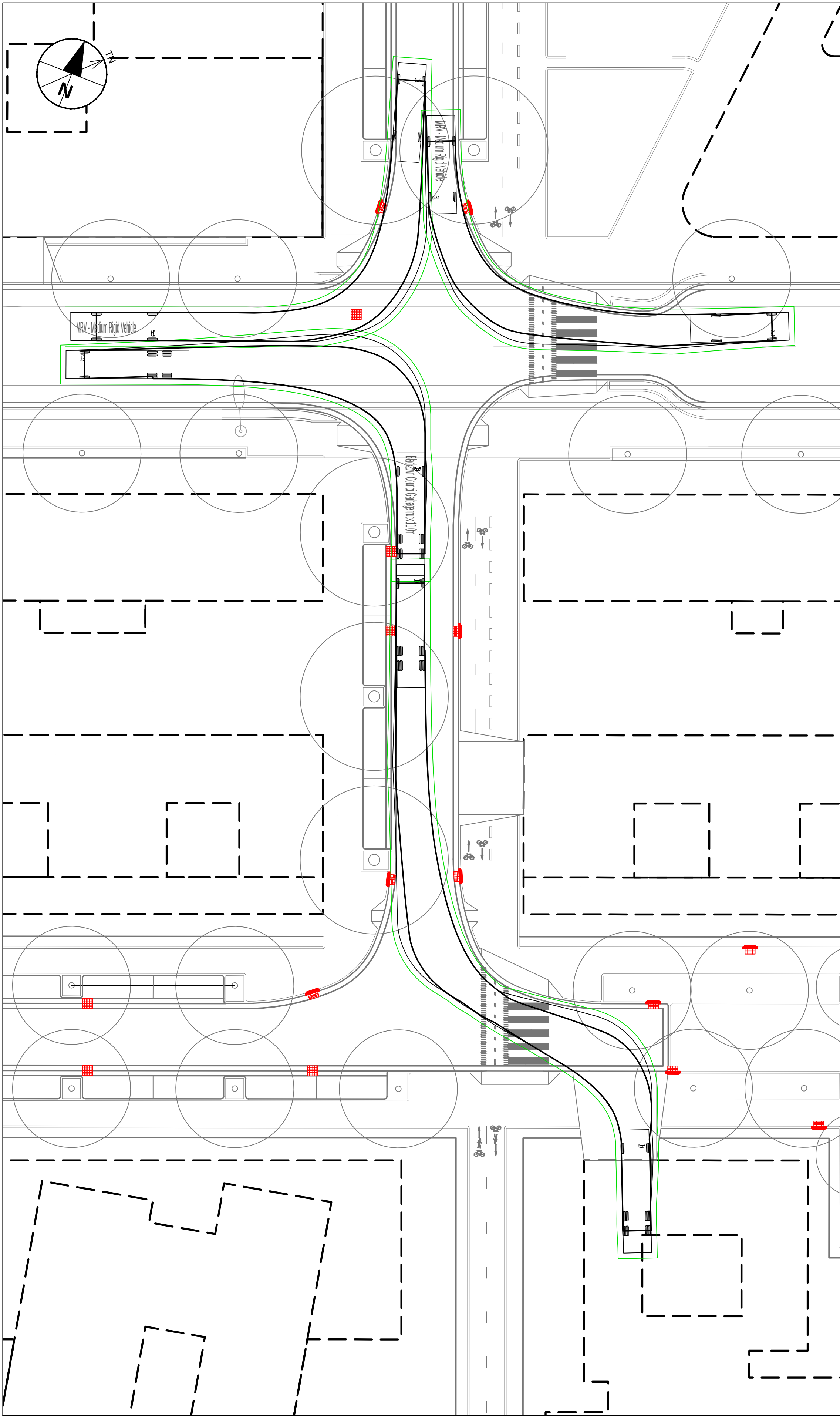
INSET 5 - LEFT TURNS Scale 1:250
