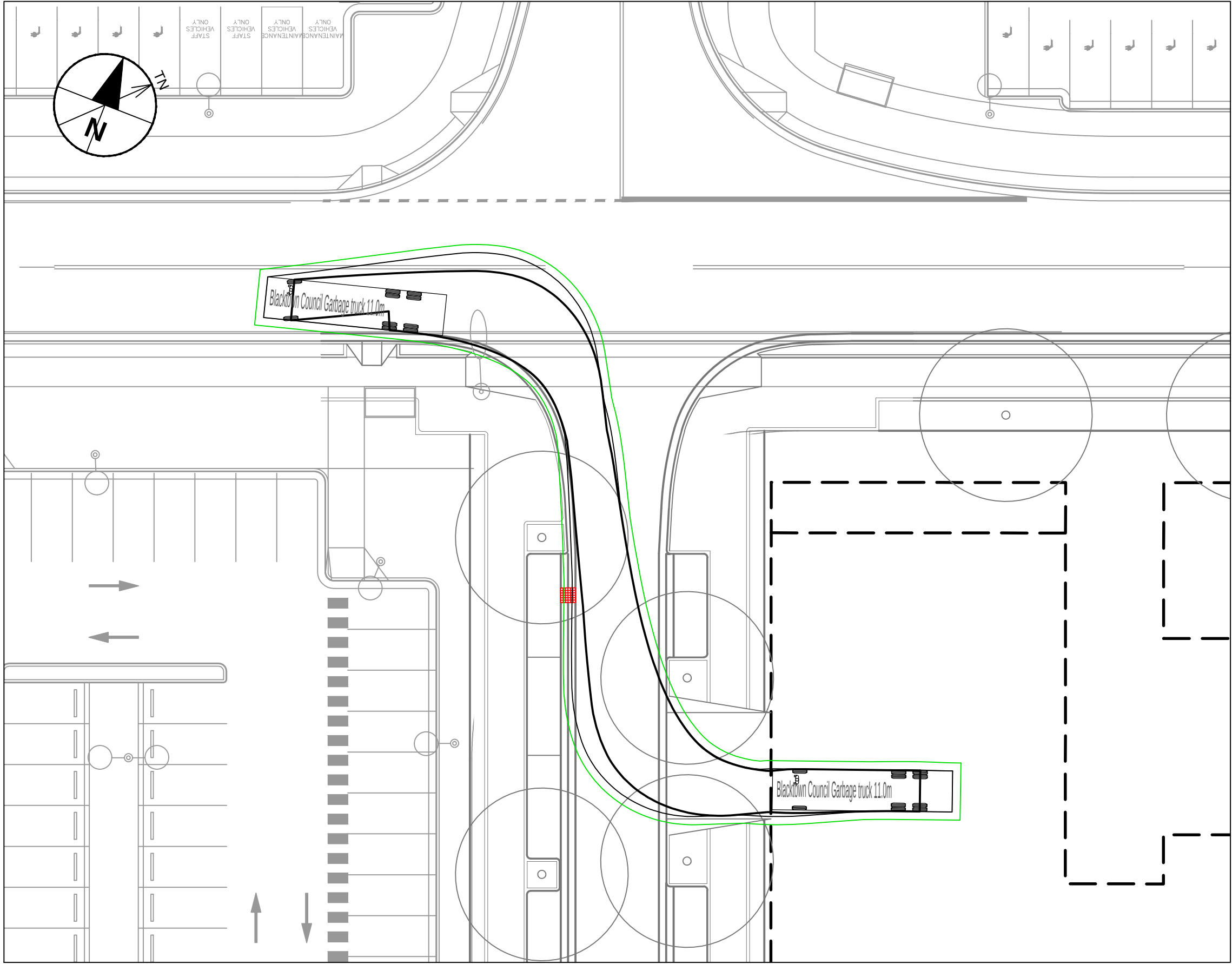
INSET 3 - FROM BUILDING LEFT TURN TO STREET
