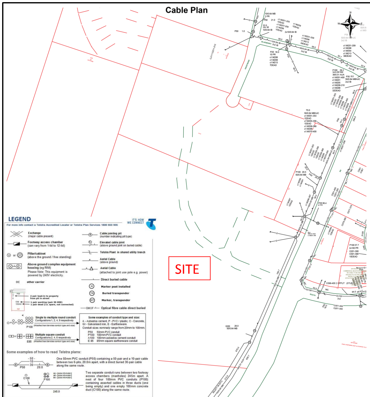
Figure 4: Telstra – Existing telecommunication assets (Cable Plan)
