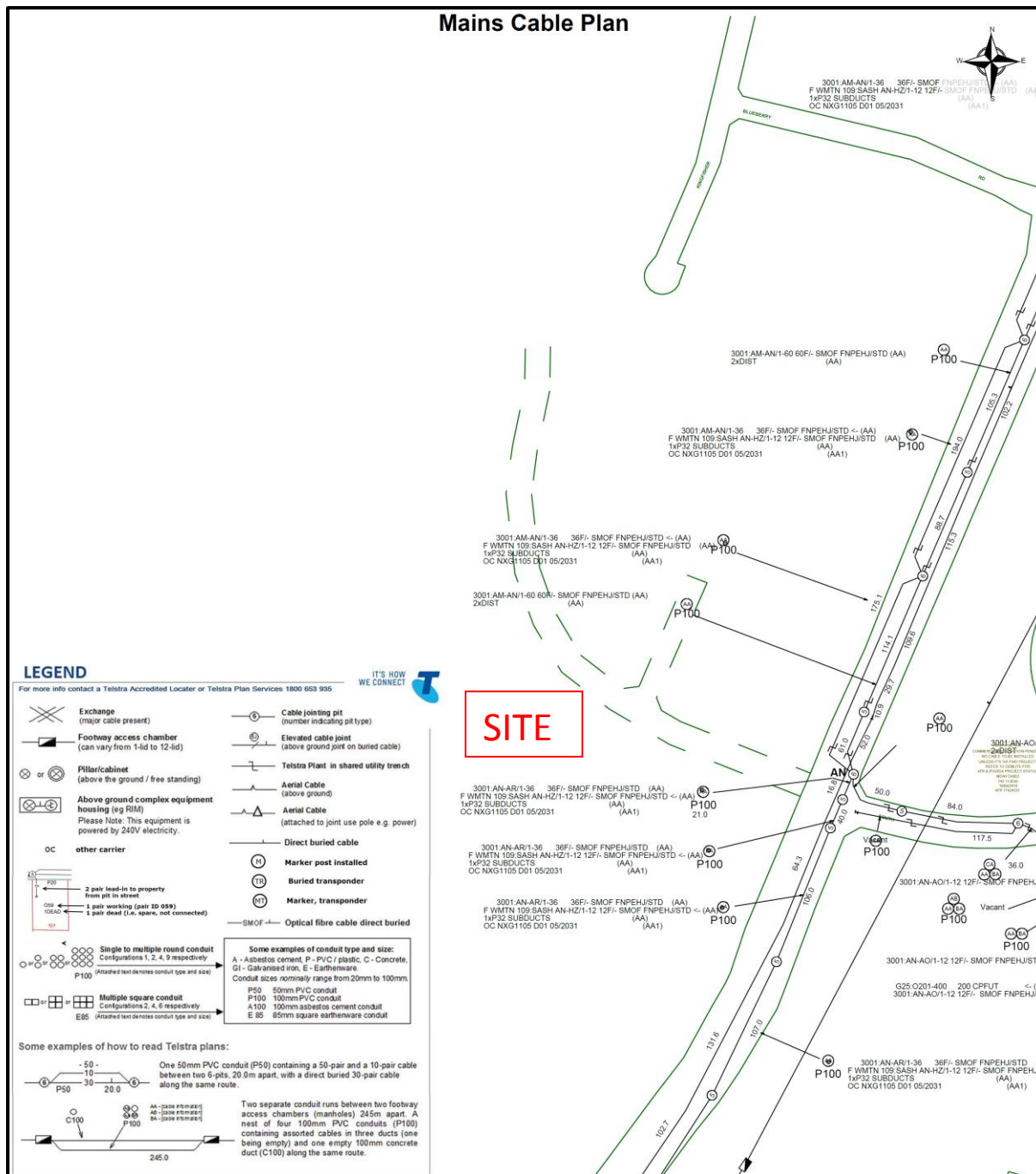
Figure 5: Telstra – Existing telecommunication assets (Mains Cable Plan)
