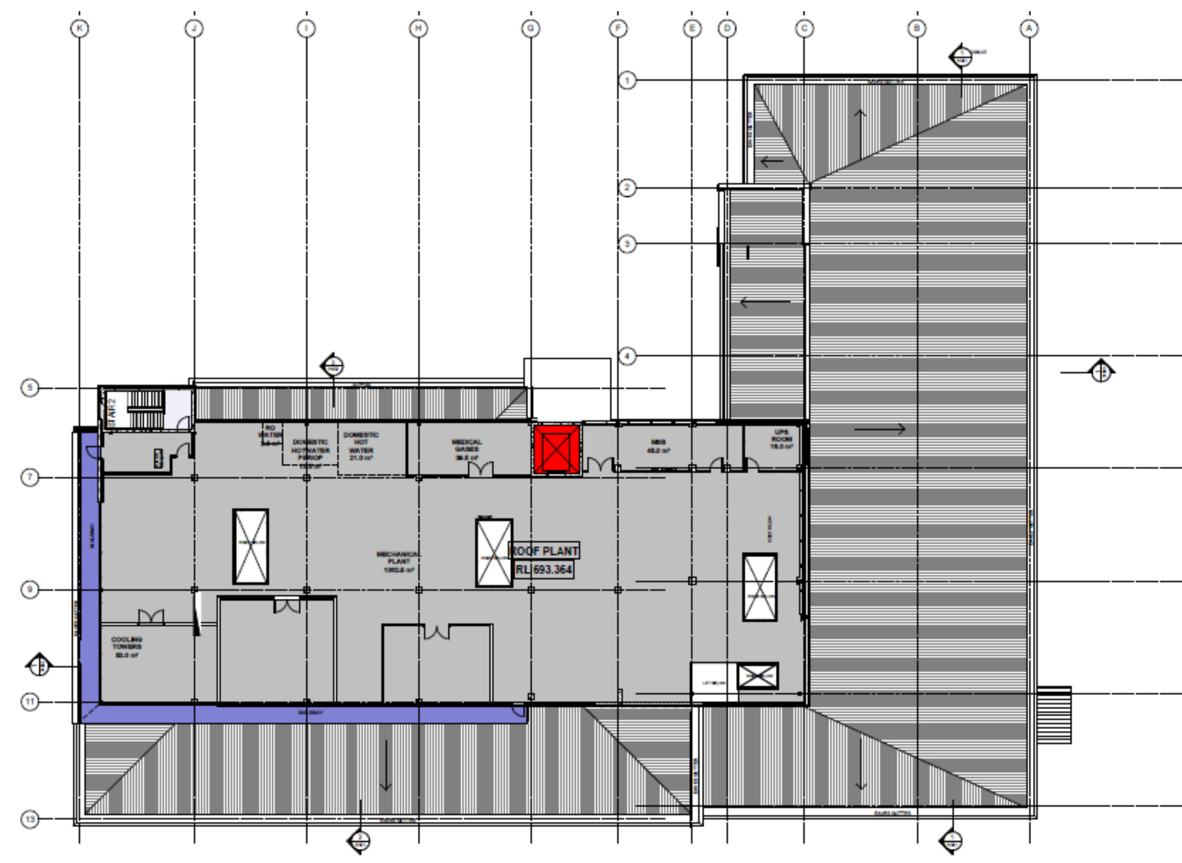
LEVEL 3 PLANT LEVEL FLOOR PLAN
