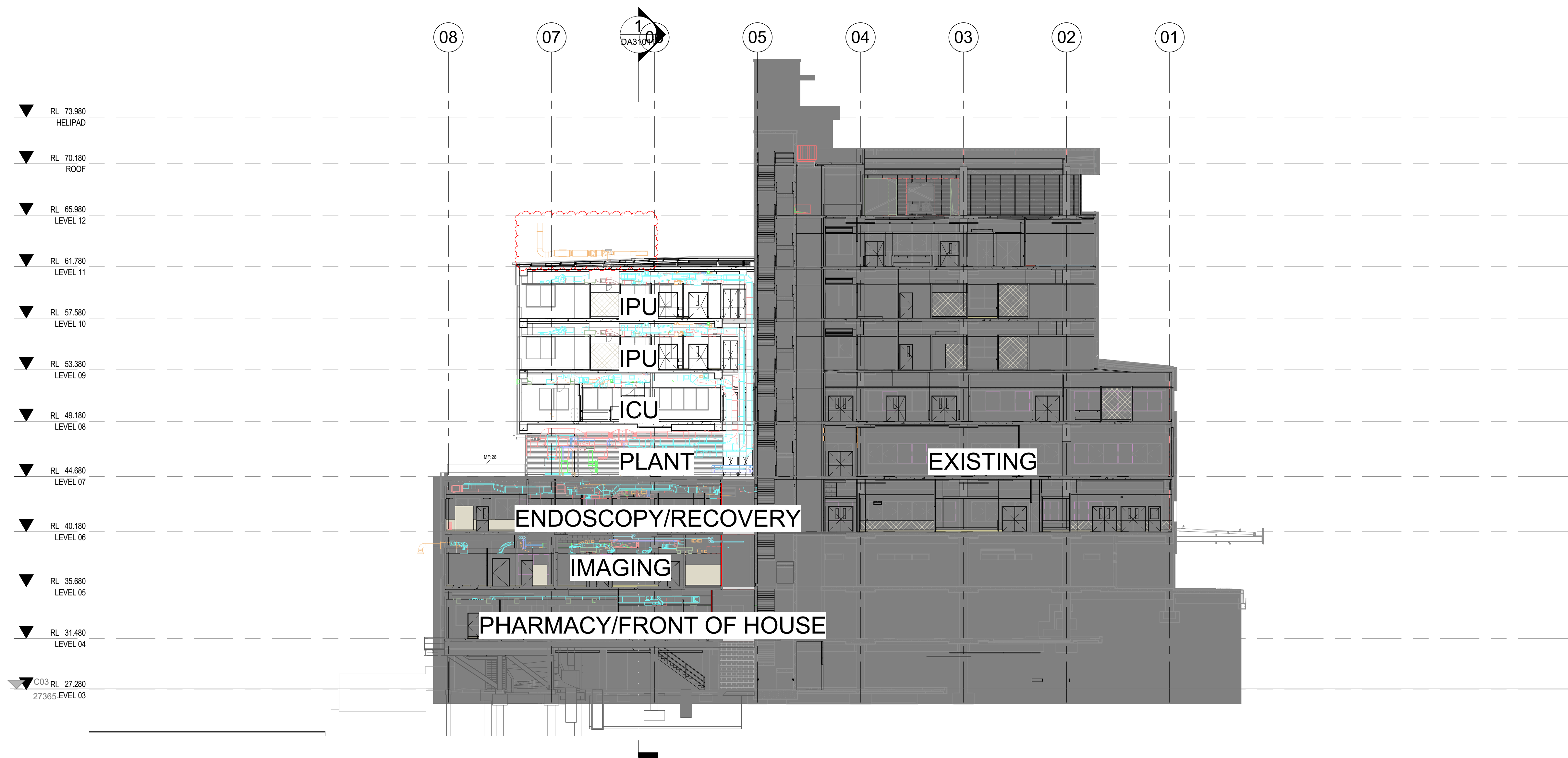
1 Overall Building Section N-S NTX SSDA A22073 1 : 200
