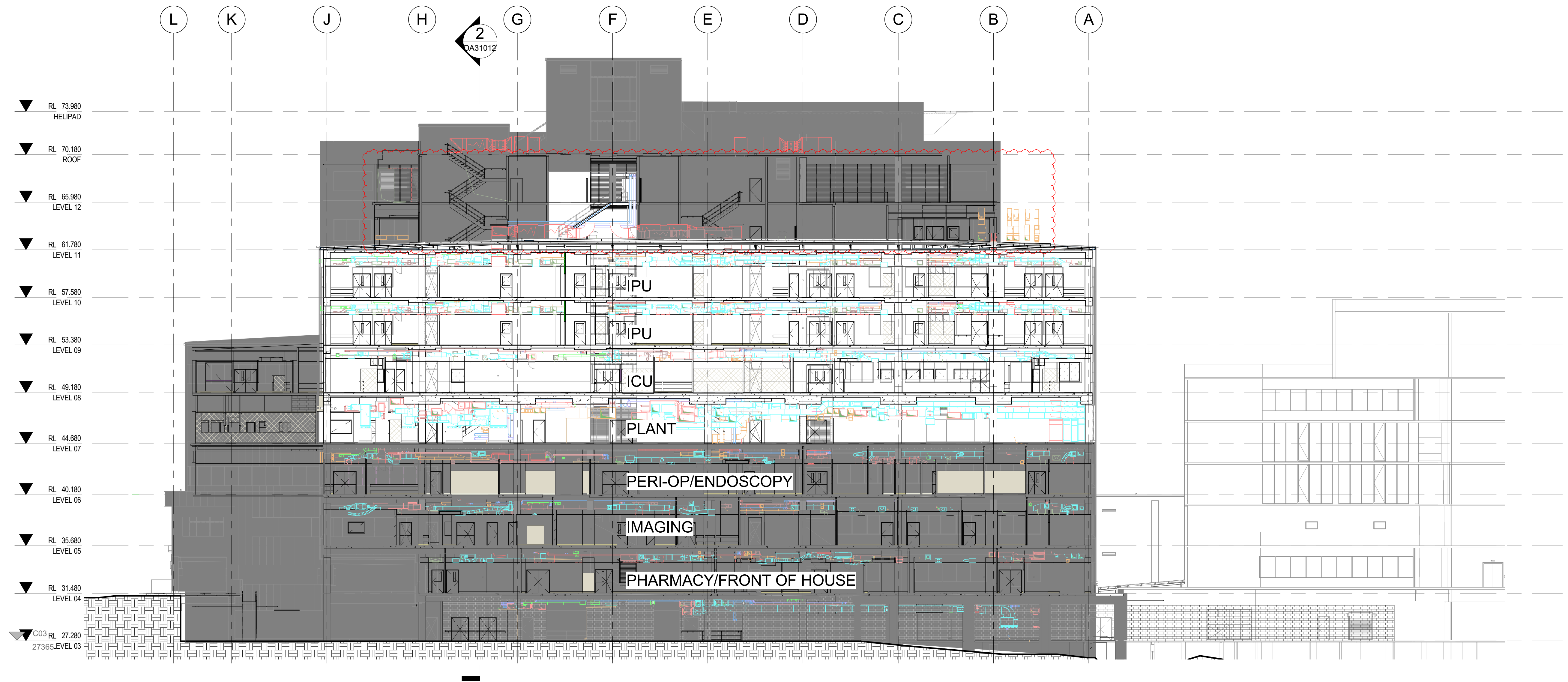
1 North Tower Building Section E-W NTX SSDA 1 : 200
