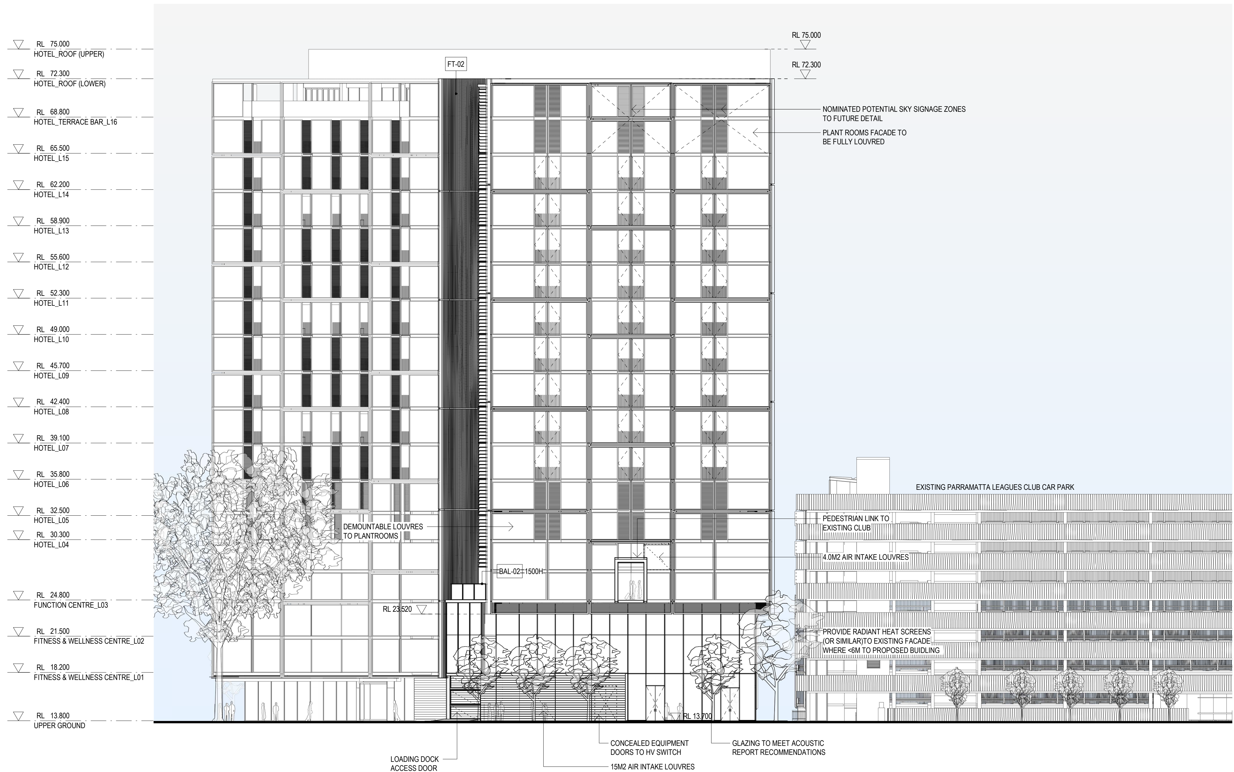
1 GA ELEVATION - NORTH-EAST (EAST) DA_1101 1:200
