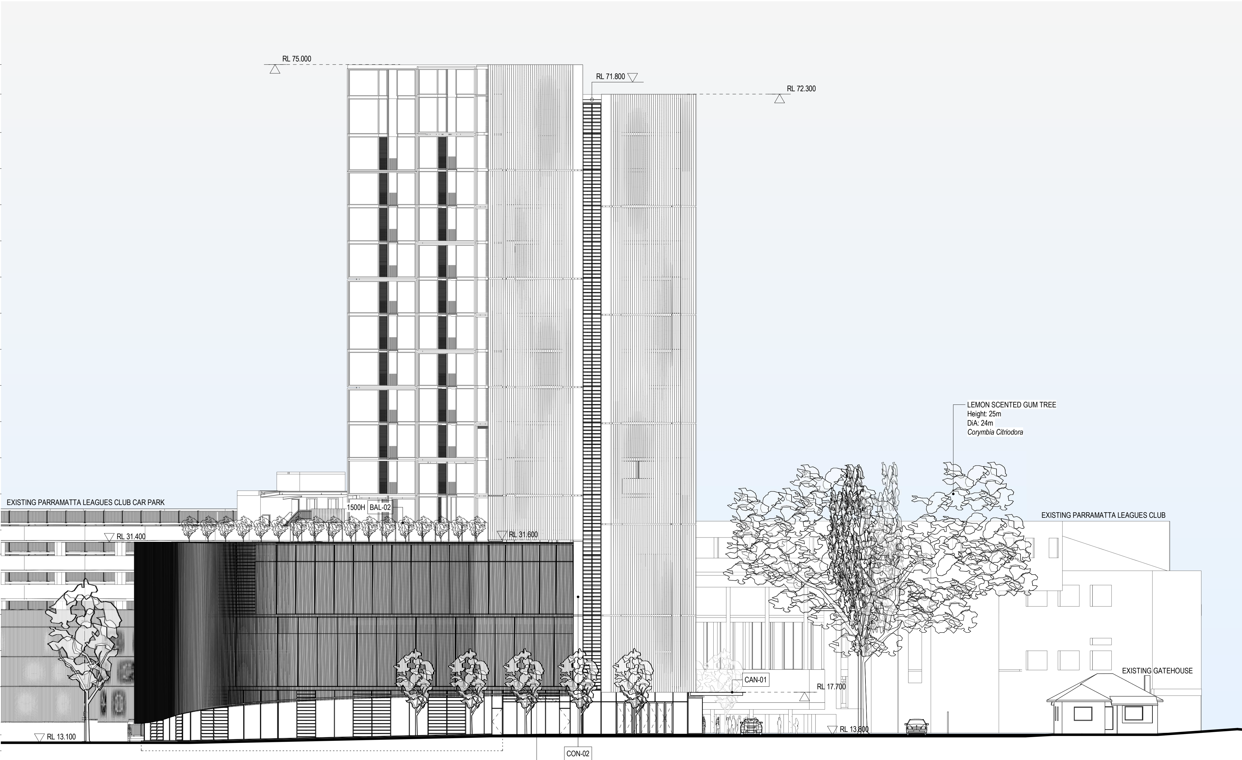
1 GA ELEVATION - SOUTH (WEST) DA_1101 1:200
