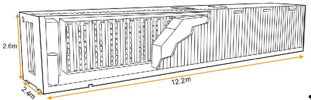
Figure 3: Layout of an individual battery unit enclosure (Planager Pty Ltd 2021)
