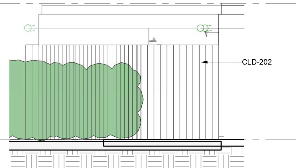
6 VIE ENCLOSURE - NORTH ELEVATION 3 16-05 SCALE 1 : 50
