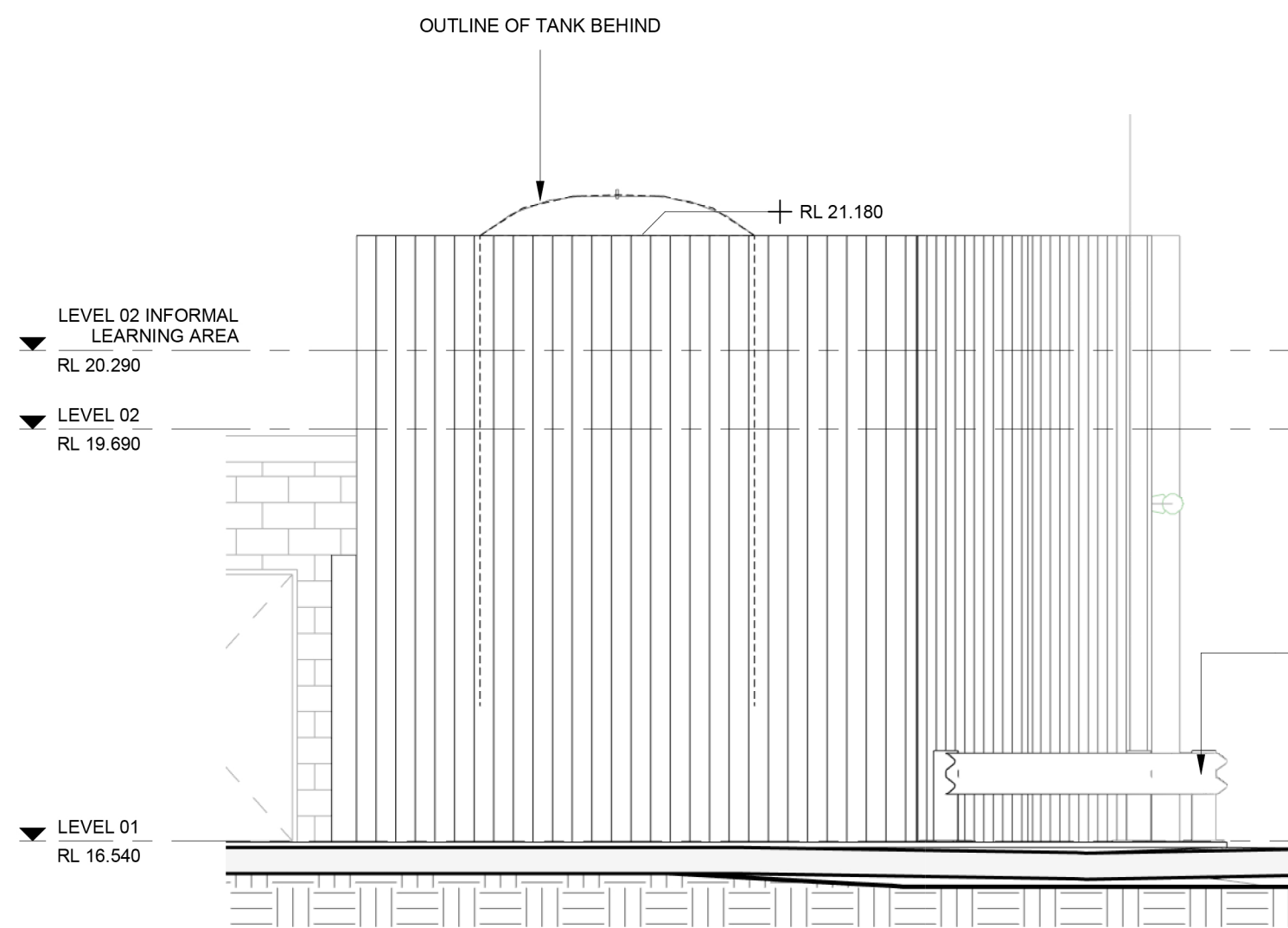
4 VIE ENCLOSURE - SOUTH ELEVATION 16-05 SCALE 1 : 50
