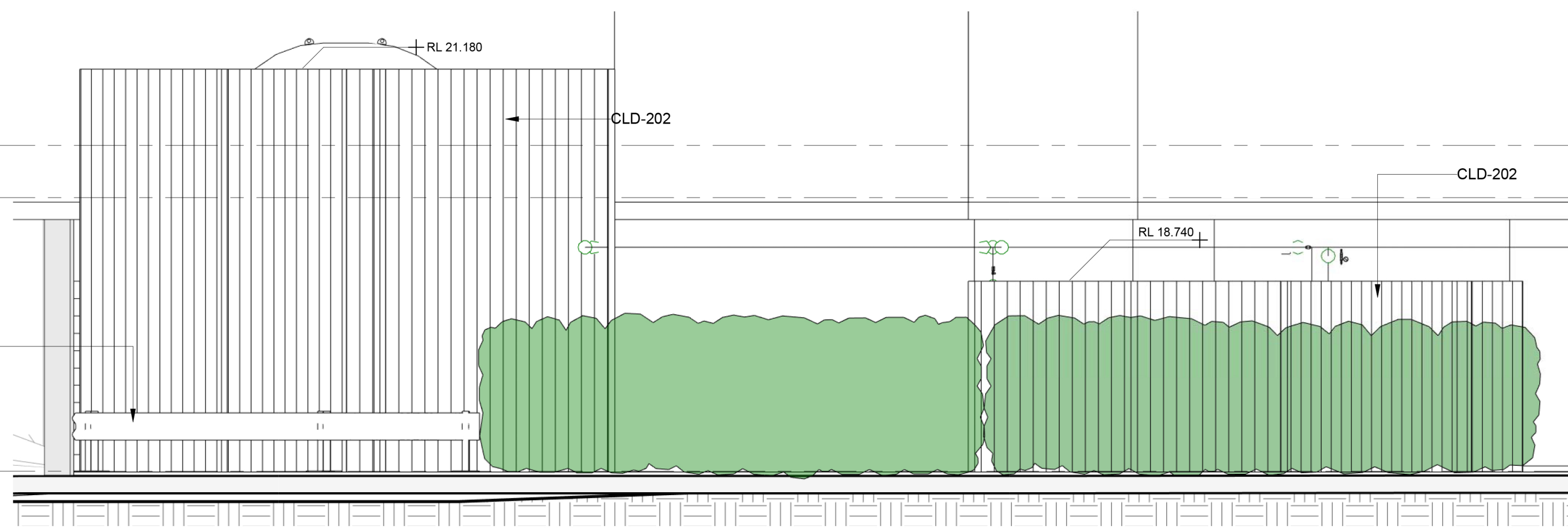
5 VIE ENCLOSURE - EAST ELEVATION 16-05 SCALE 1 : 50
