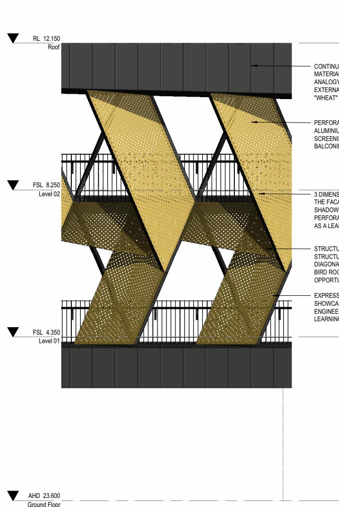
2 Kernel Facade Elevation 1:50
