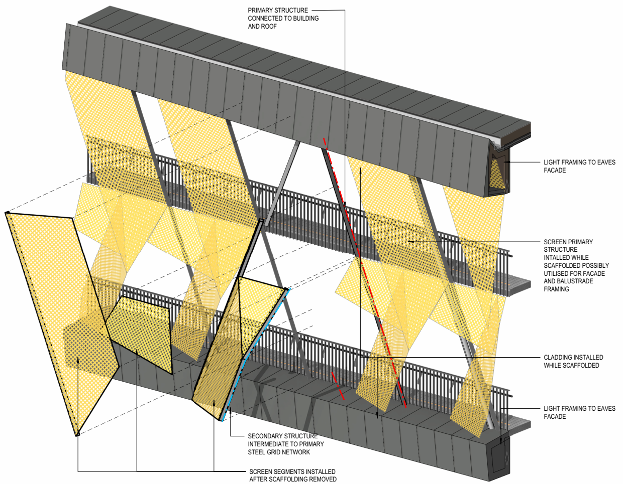
9 Kernel Alternative Assembly
