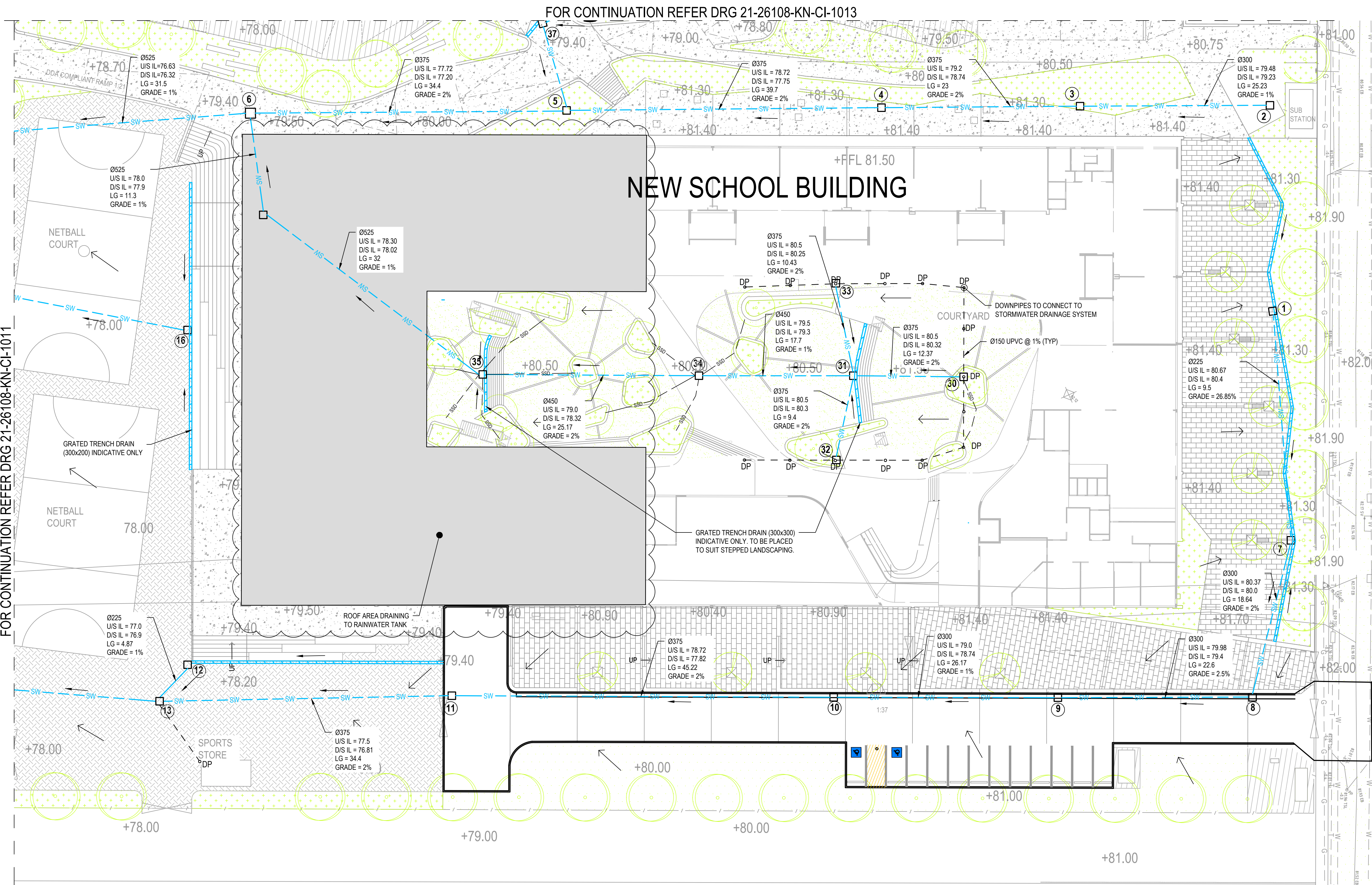
STORMWATER DRAINAGE PLAN
