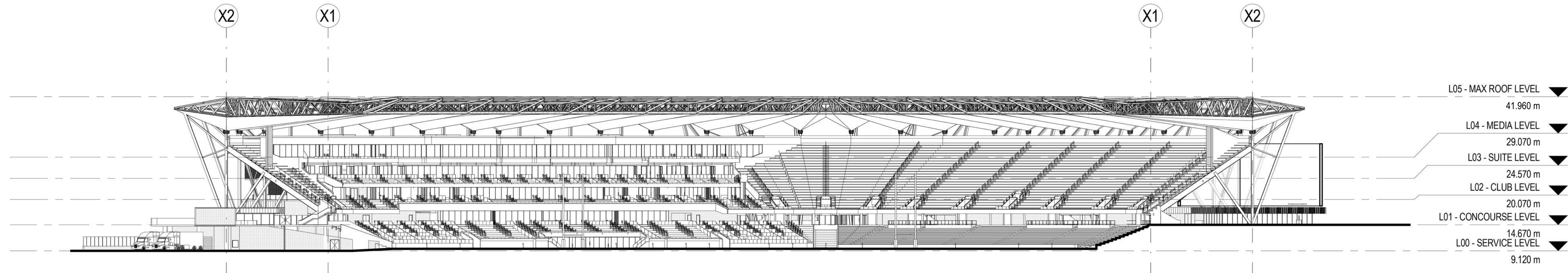
3 CORNER SECTION - LOOKING NORTH WEST 1 : 500
