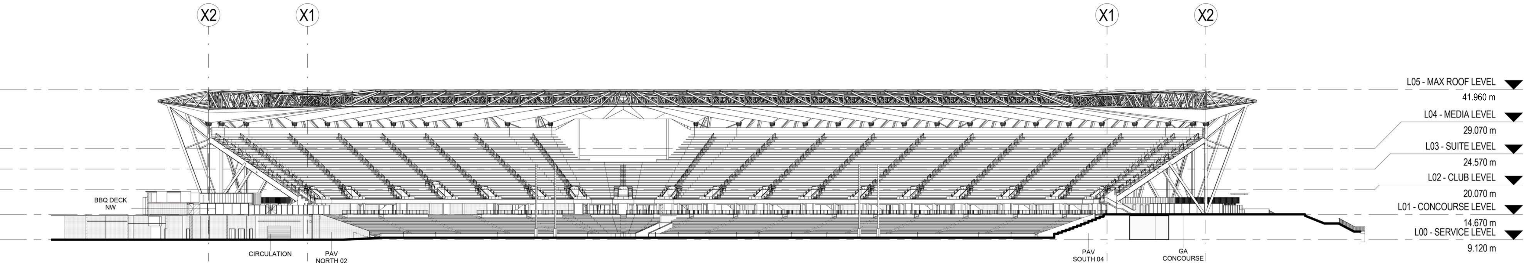
4 CORNER SECTION - LOOKING NORTH EAST 1 : 500
