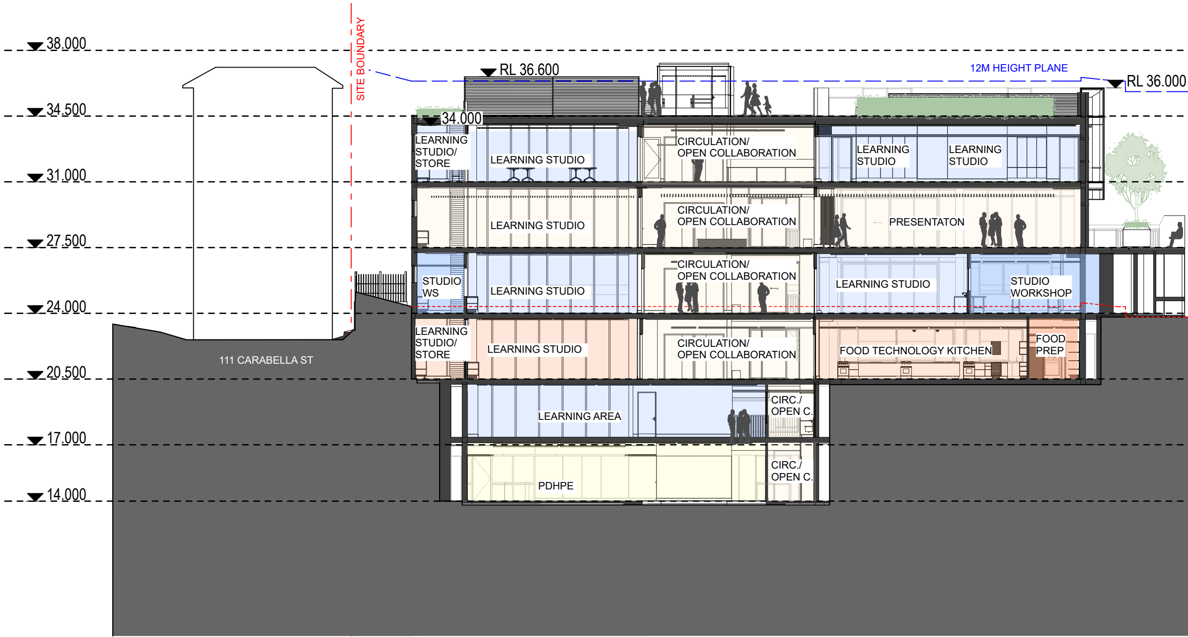
1 SECTION C Learning Hub 1:200
