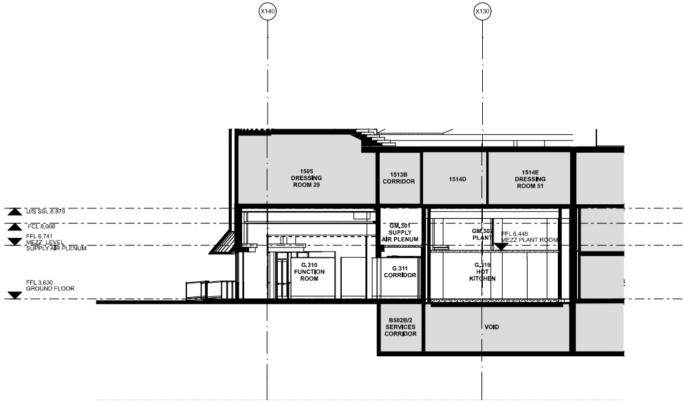
1 FUNCTION CENTRE N-S SECTION 1 LOOKING EAST 1:100
