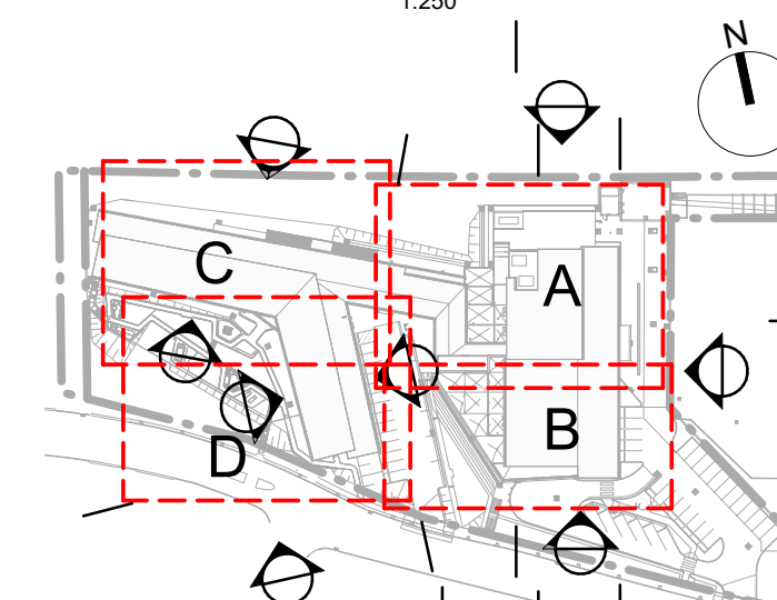
ZONES SHOWN FOR: AA-10 GENERAL ARRANGEMENT PLANS AA-11 SUPERSTRUCTURE PLANS AA-13 REFLECTED CEILING PLANS AA-14 FFE PLANS AA-15 FINISHES PLANS
