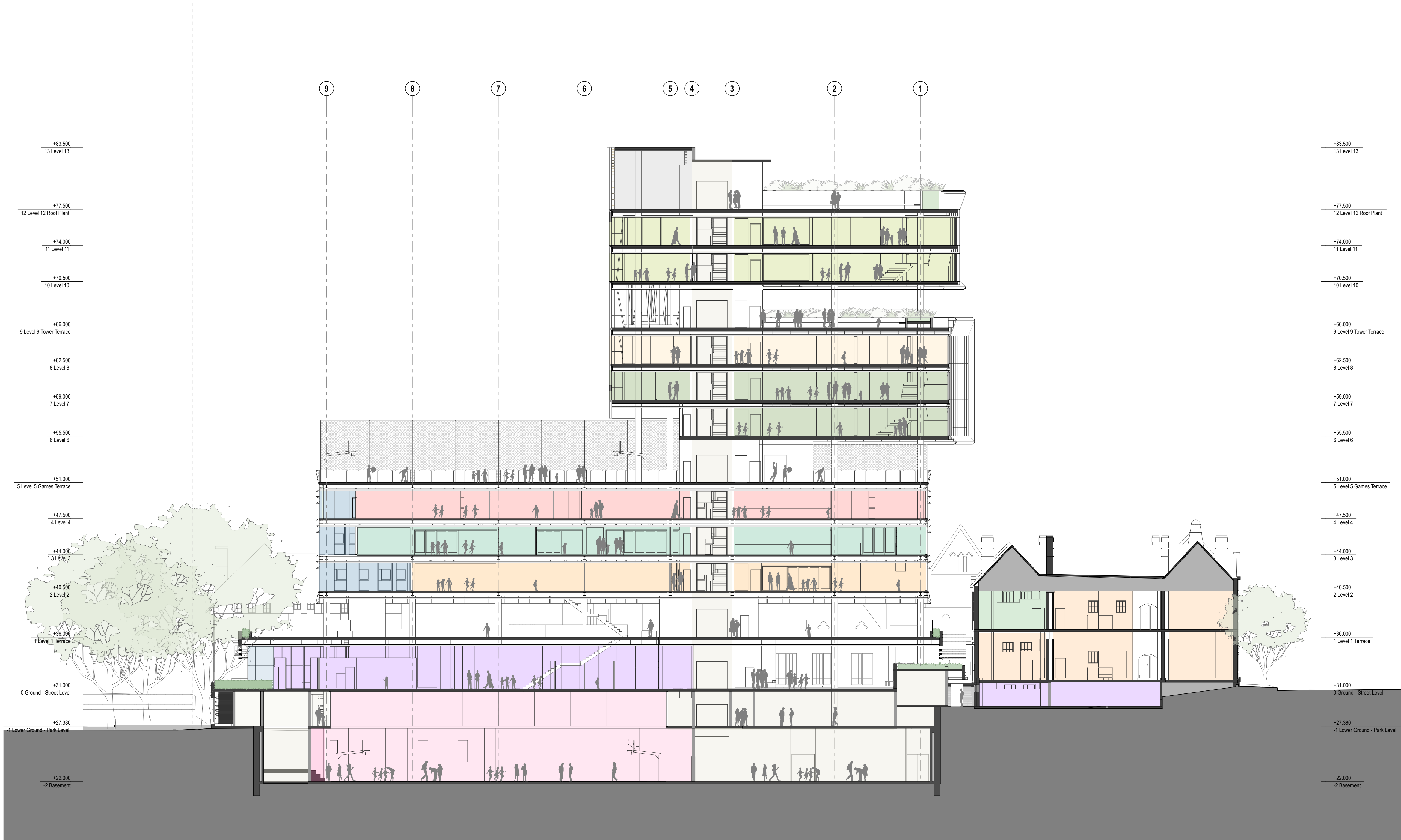
Cross Section A 1:200
