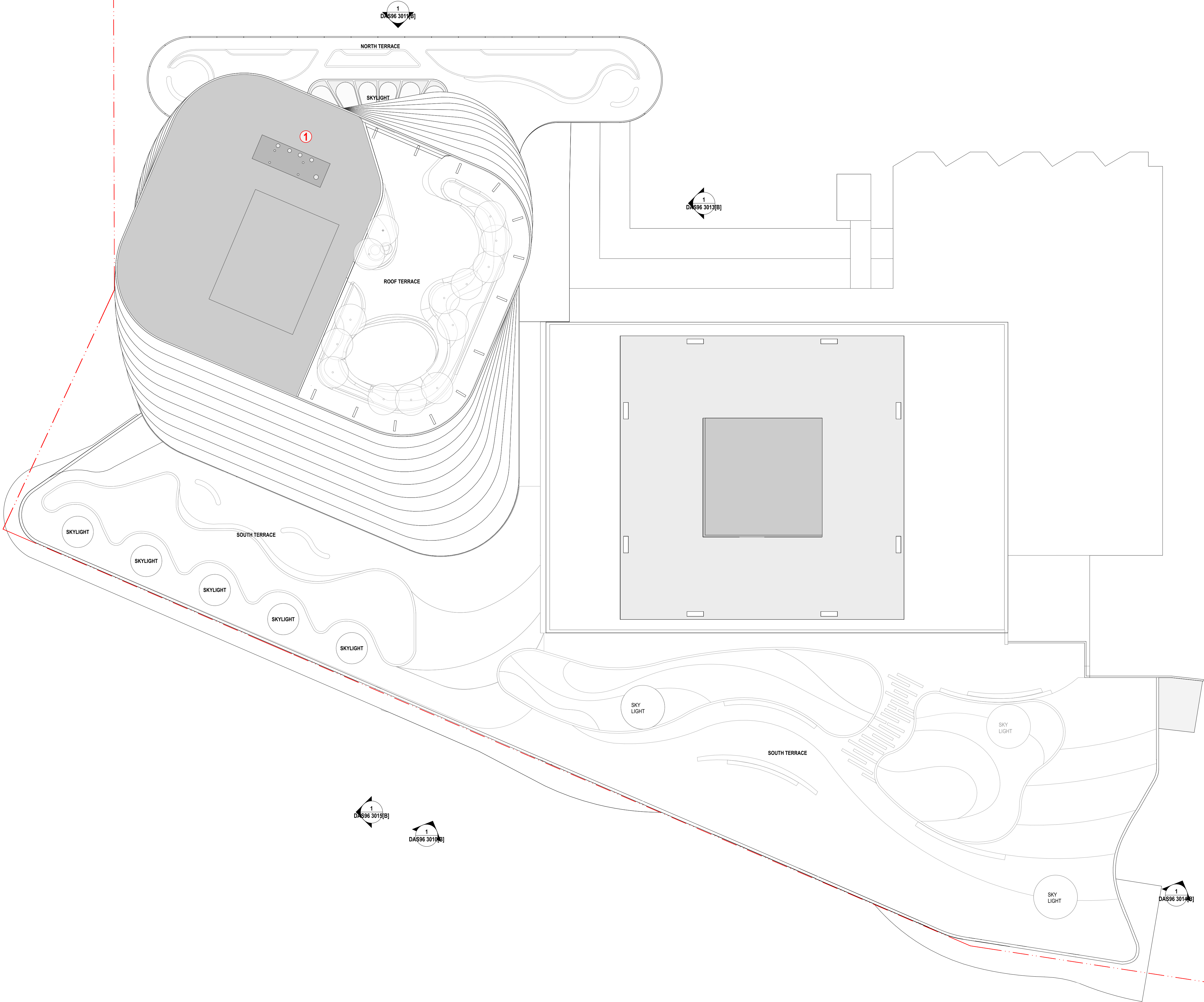
General Arrangement Proposed - RF Roof
