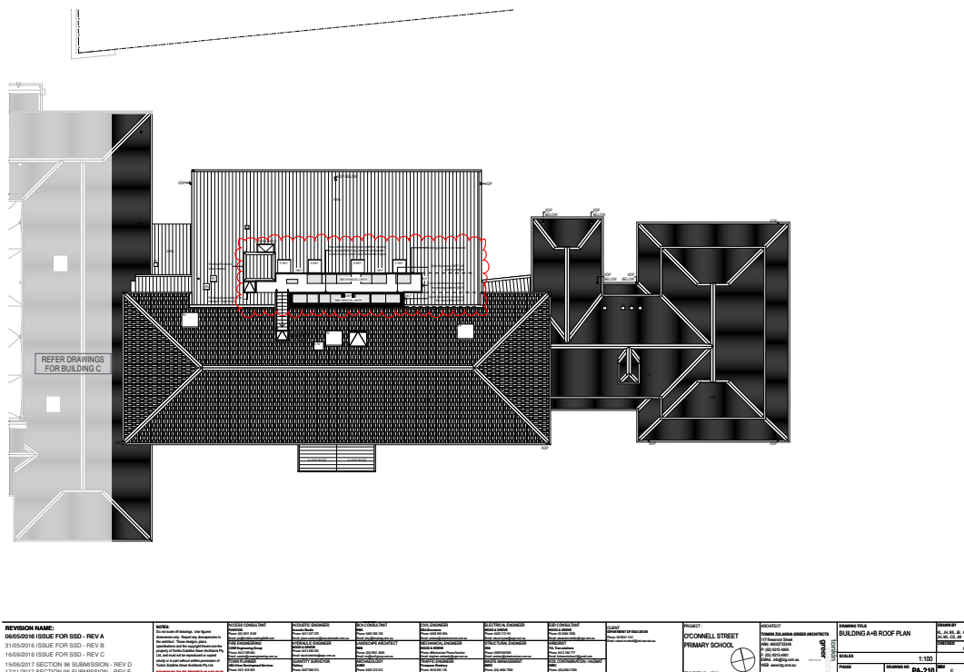
Figure 27: Building B Roof Plan, showing the revised layout of the plant platform.
