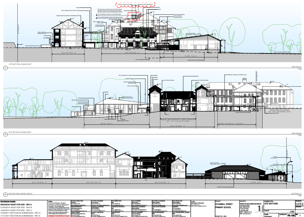
Figure 25: Sections, showing the revised layout of the condenser units. The site section looking east shows the significantly reduced impact of the plant platform following the proposed revisions.
