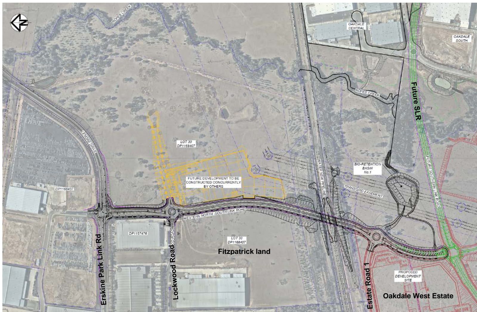
Figure 5: WNSLR
