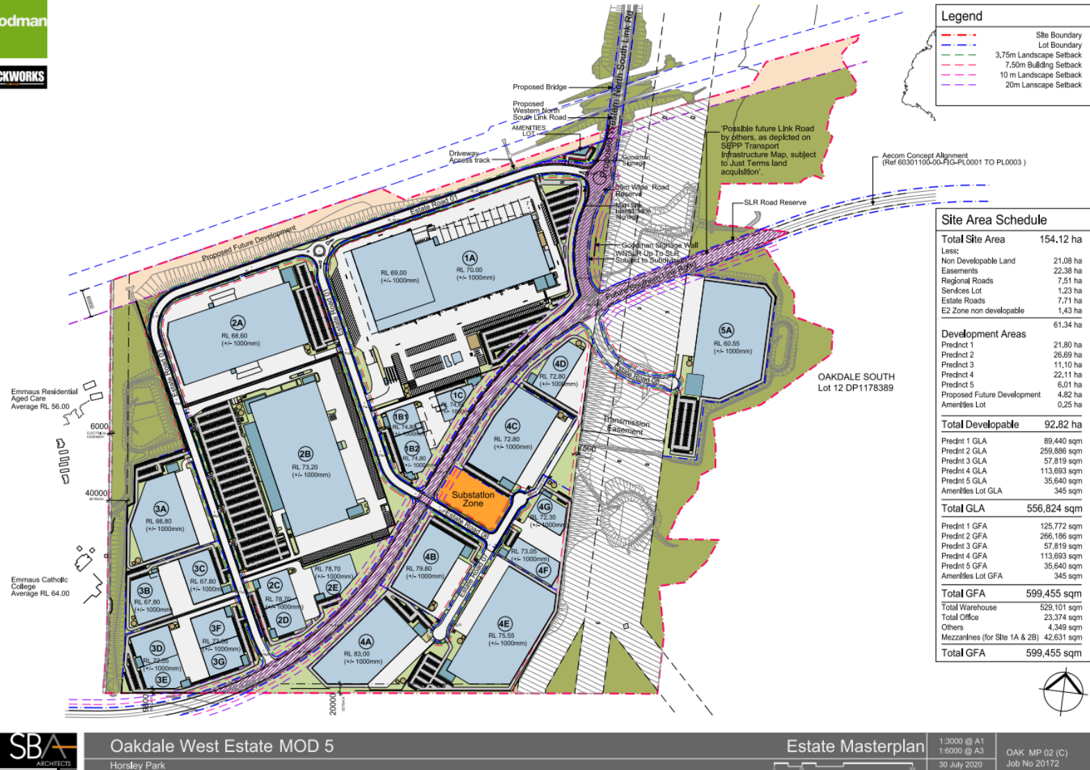
Figure 1: Concept Proposal Layout (MOD 5)
