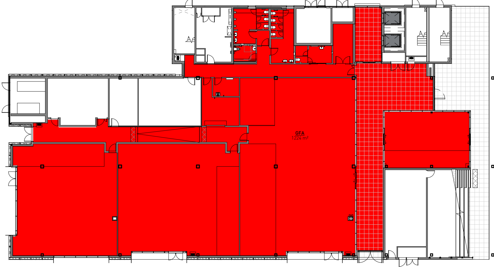
2 DA GFA - GROUND FLOOR 1 : 300
