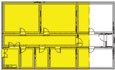
Building 10A S.E. Asian Tropical 350m 2
