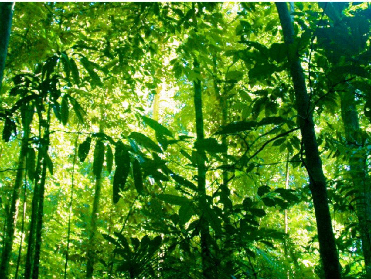
African Highlands Vegetation
