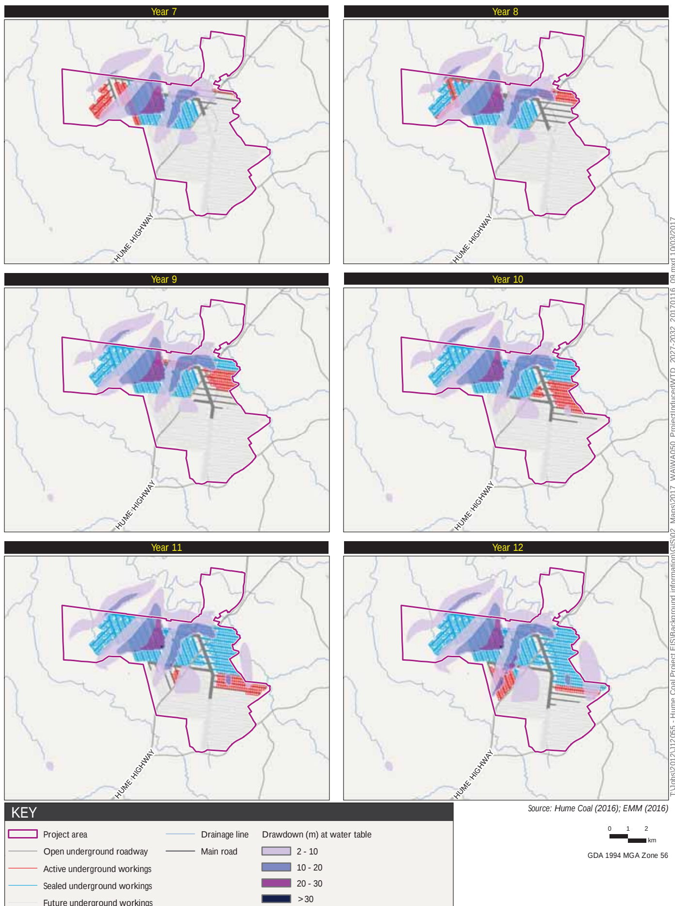
Project water table drawdown: Year 7 - Year 12 Hume Coal Project Water Assessment Figure M.1b (Appendix M)
