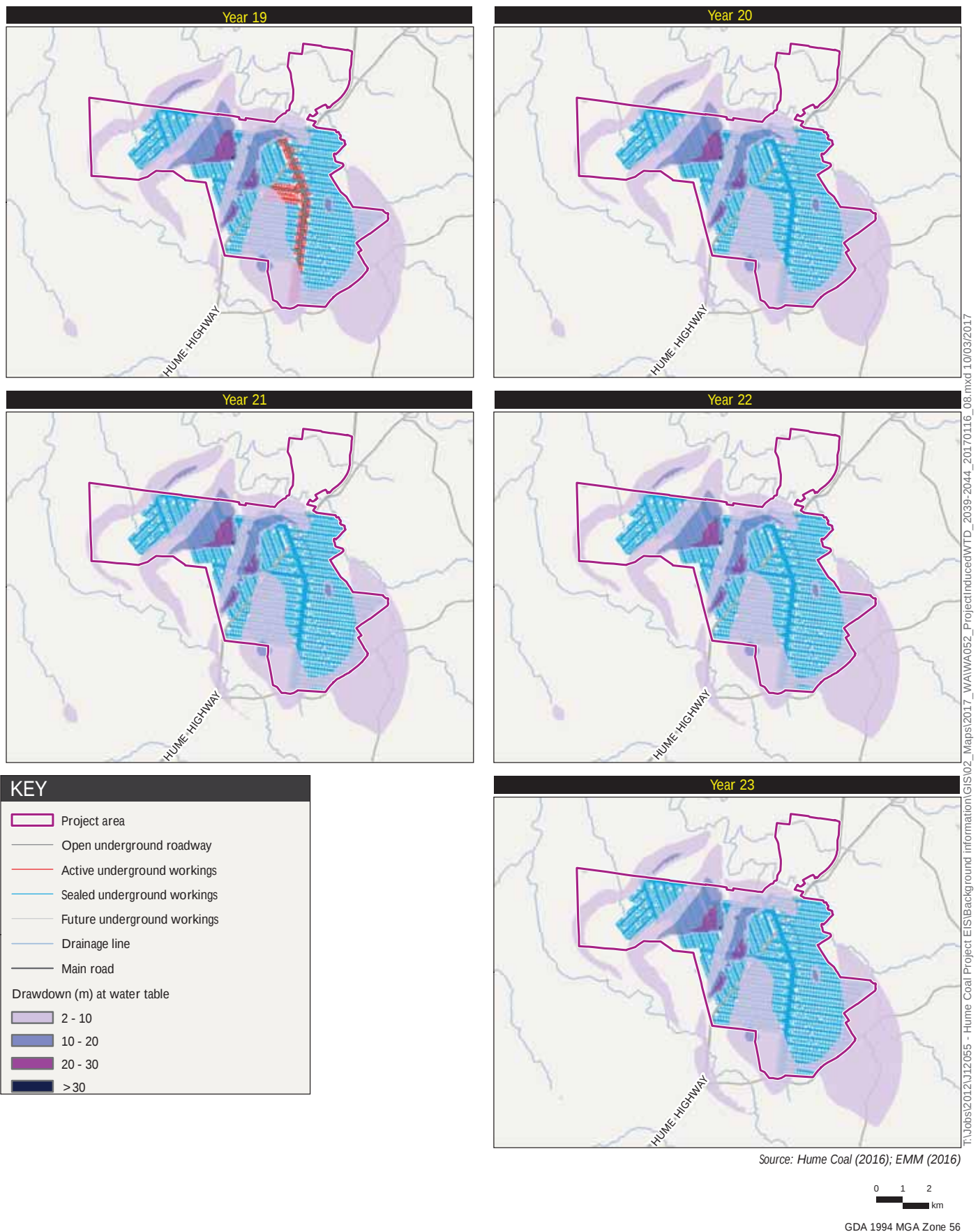
Project water table drawdown: Year 19 - Year 23 Hume Coal Project Water Assessment Figure M.1d (Appendix M)
