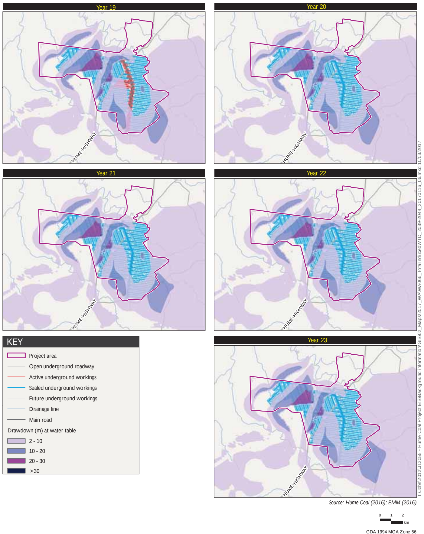
Total water table drawdown: Year 19 - Year 23 Hume Coal Project Water Assessment Figure M.2d (Appendix M)
