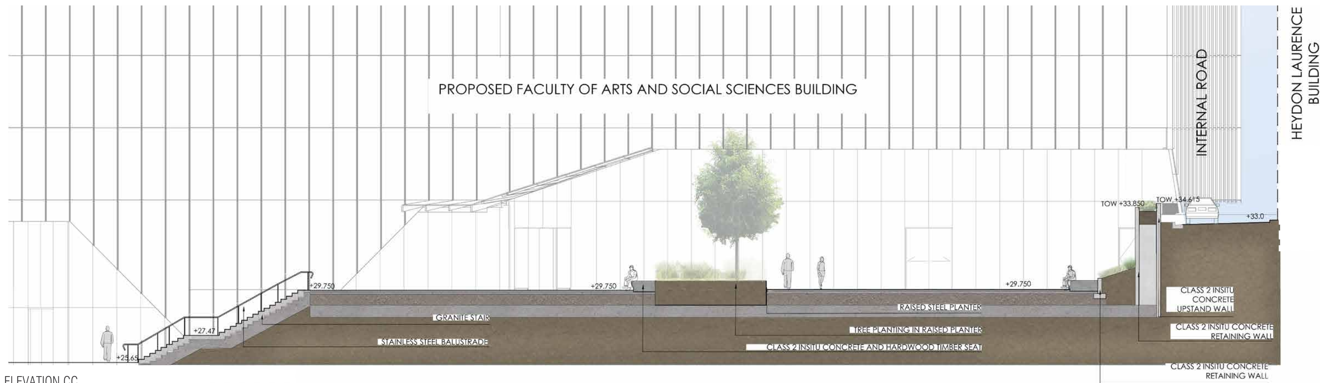
ELEVATION CC SCALE 1:100 @ A1
