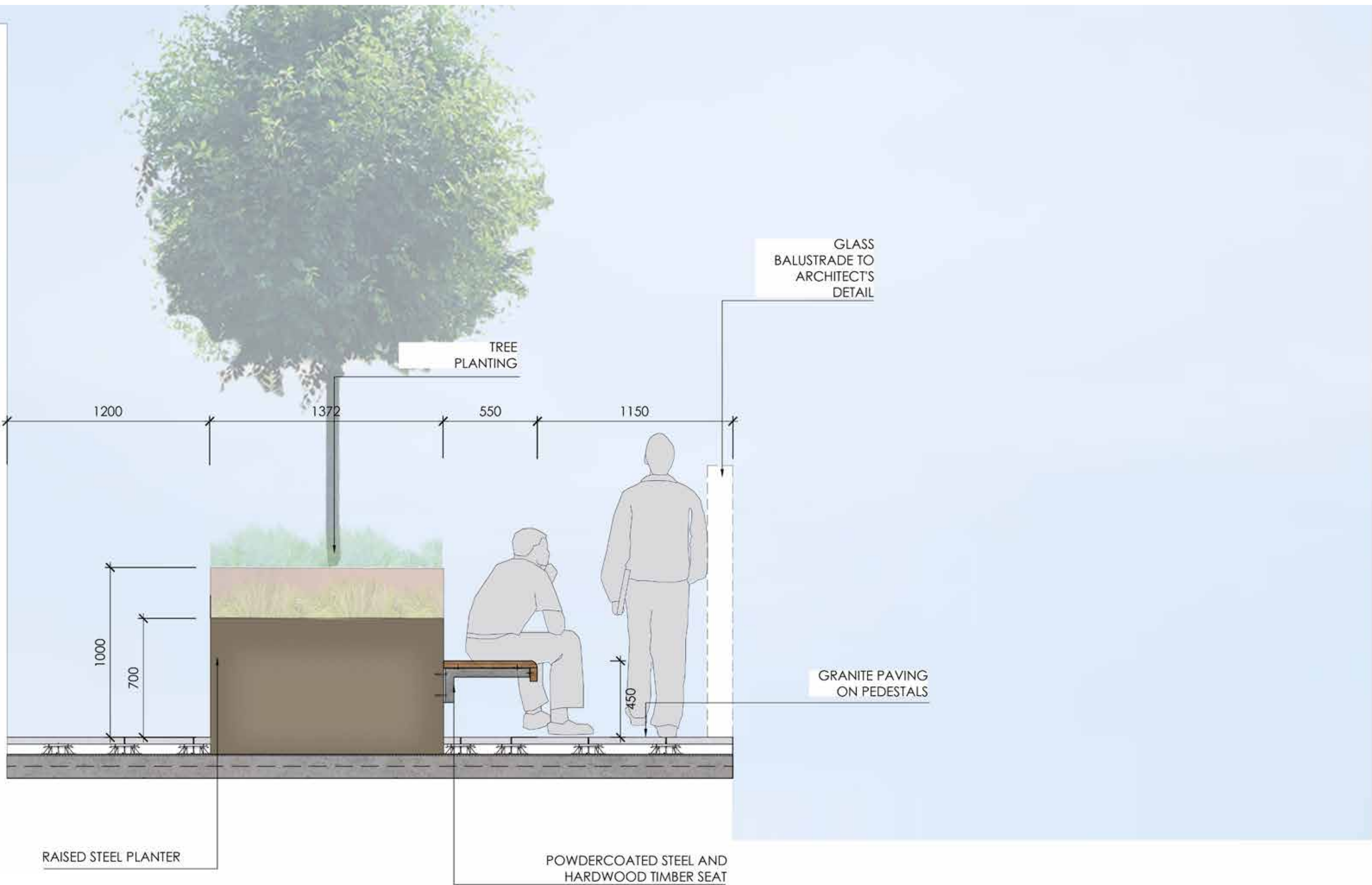
ELEVATION GG SCALE 1:50 @ A1
