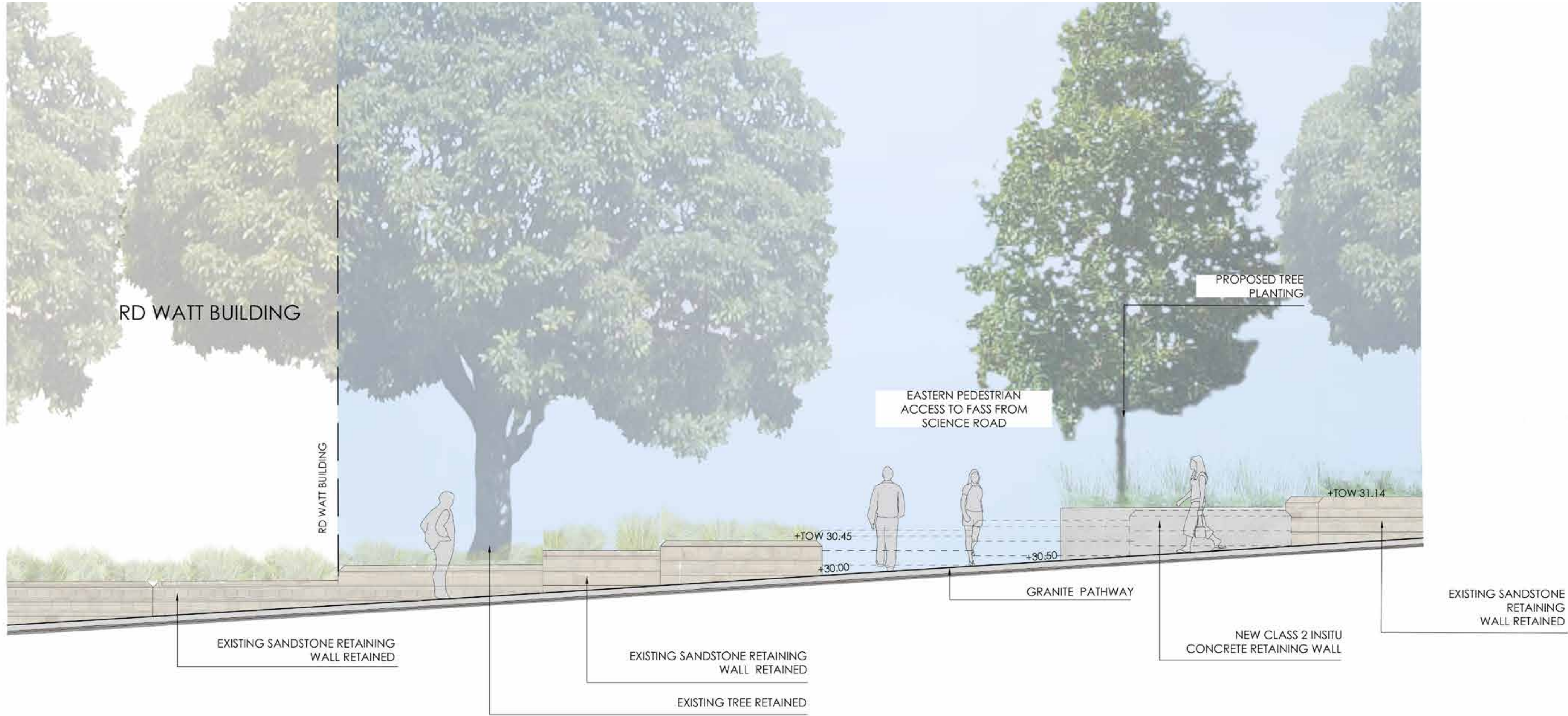
ELEVATION EE SCALE 1:50 @ A1
