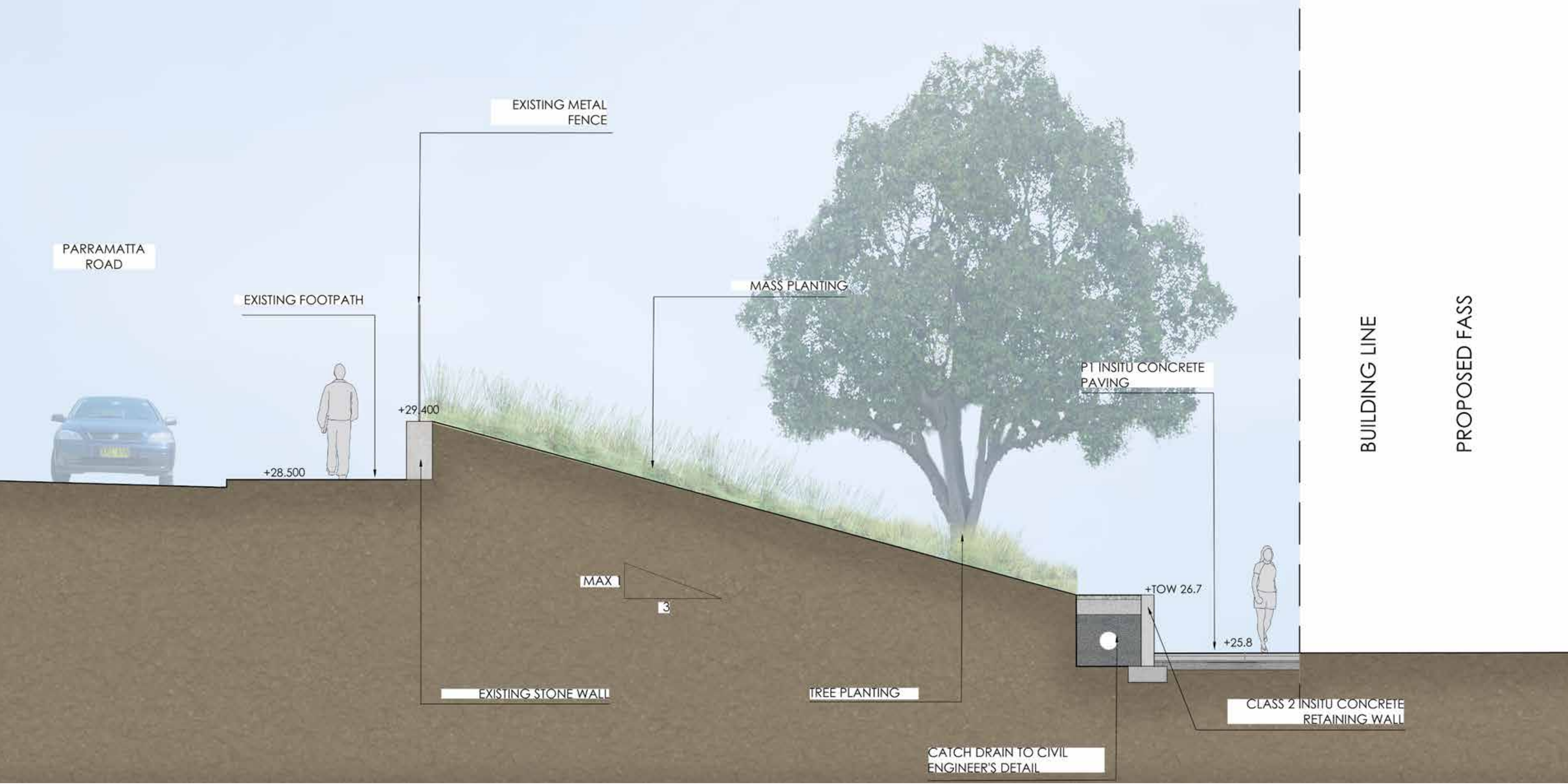
ELEVATION GG SCALE 1:50 @ A1
