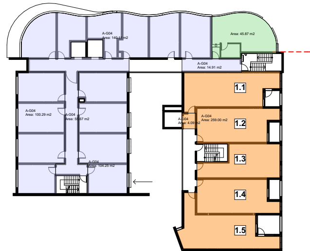
LEVEL 02
