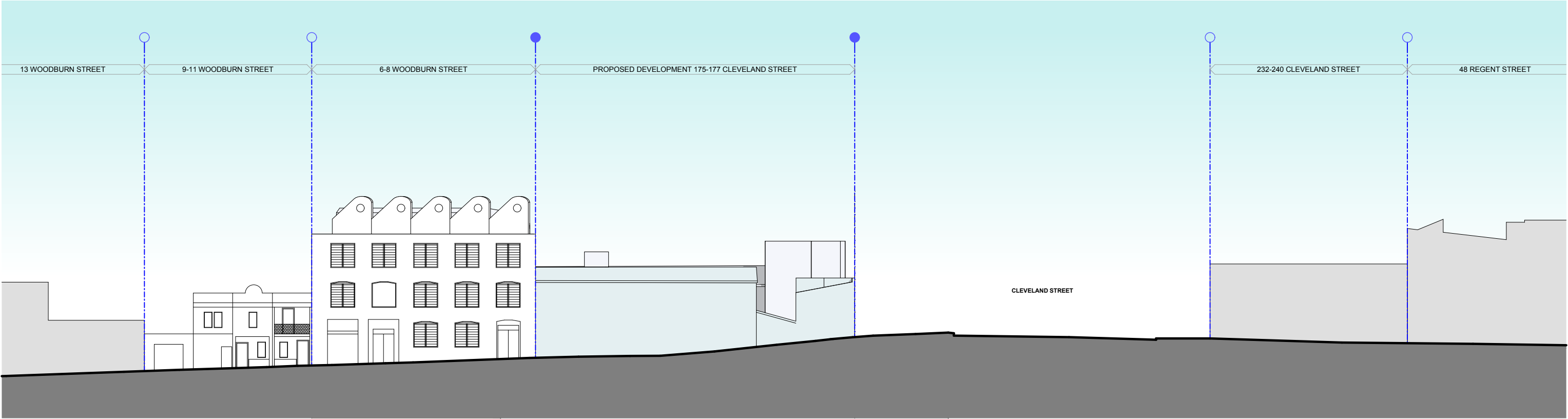
1 WOODBURN STREET 1:400
