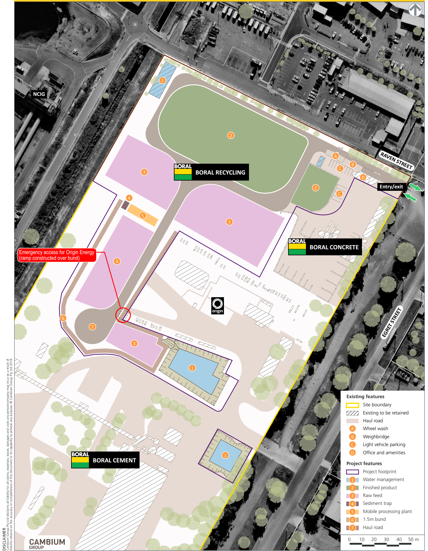
Figure 2 GENERAL ARRANGEMENT Boral Recycling Kooragang
