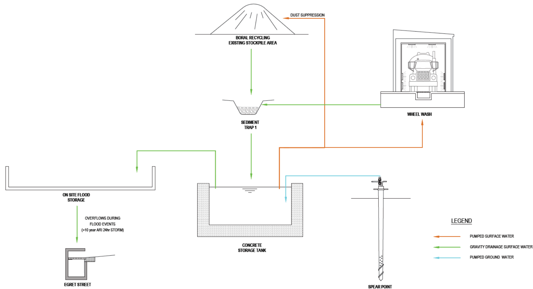
Figure 12 Conceptual flow diagram for existing WRF
