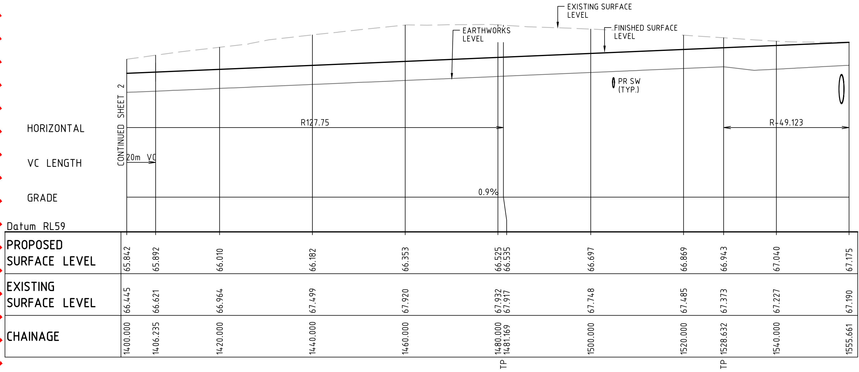
ROAD 01 LONGITUDINAL SECTION
