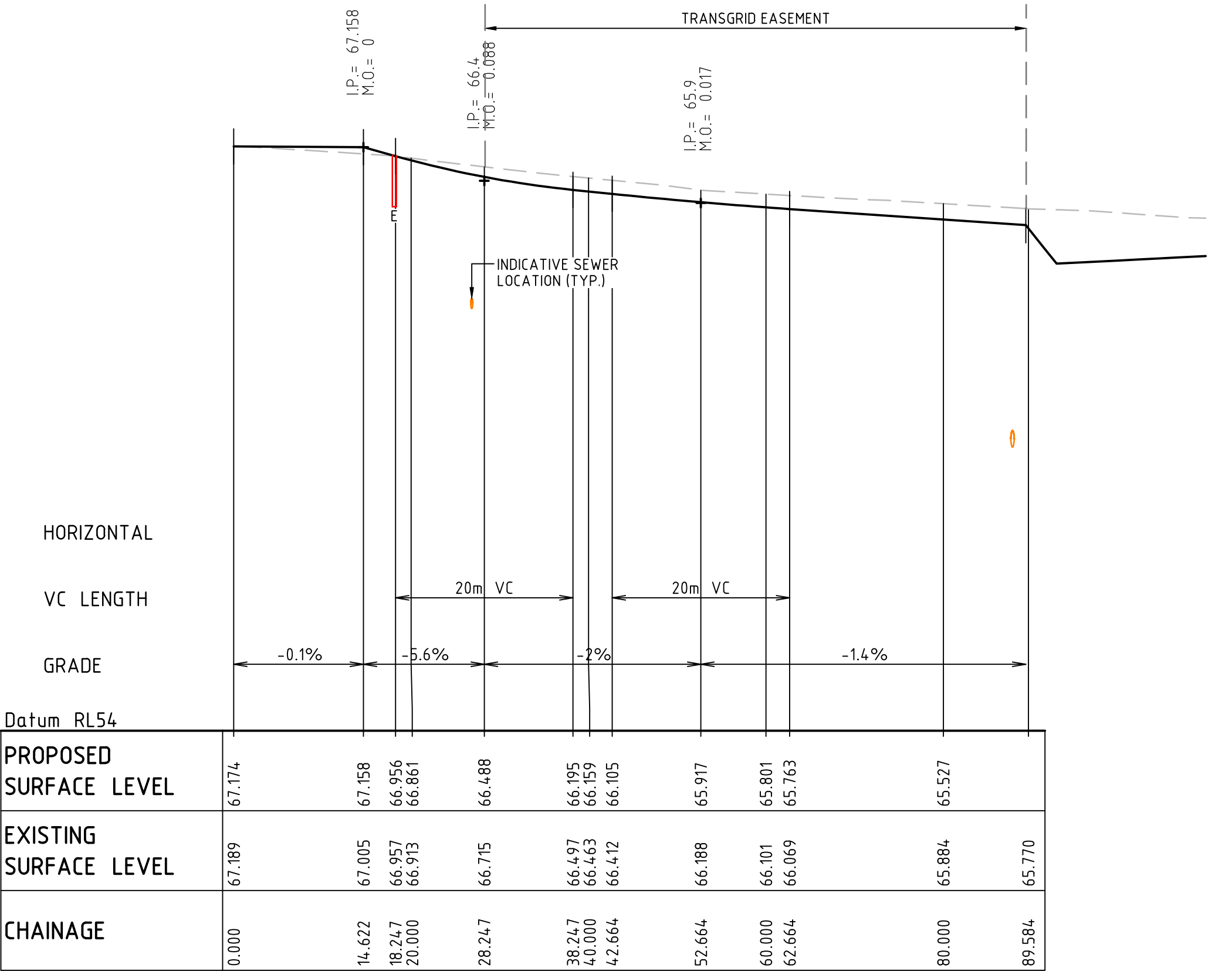
TRANSGRID EASEMENT ACCESS DRIVEWAY (ROAD 06) LONGITUDINAL SECTION
