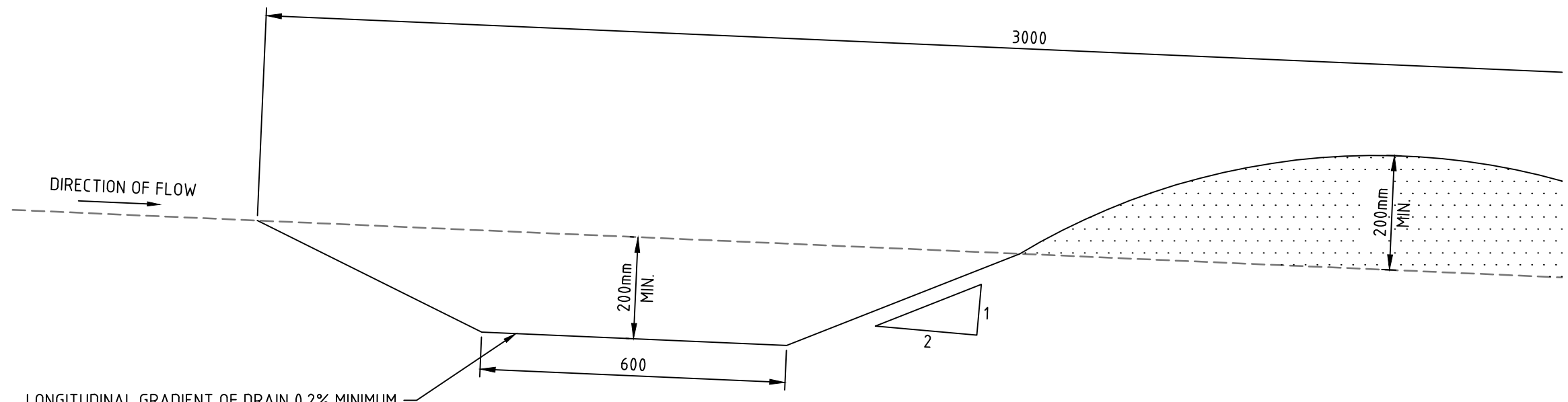
CATCH DRAIN DETAIL SCALE 1:10
