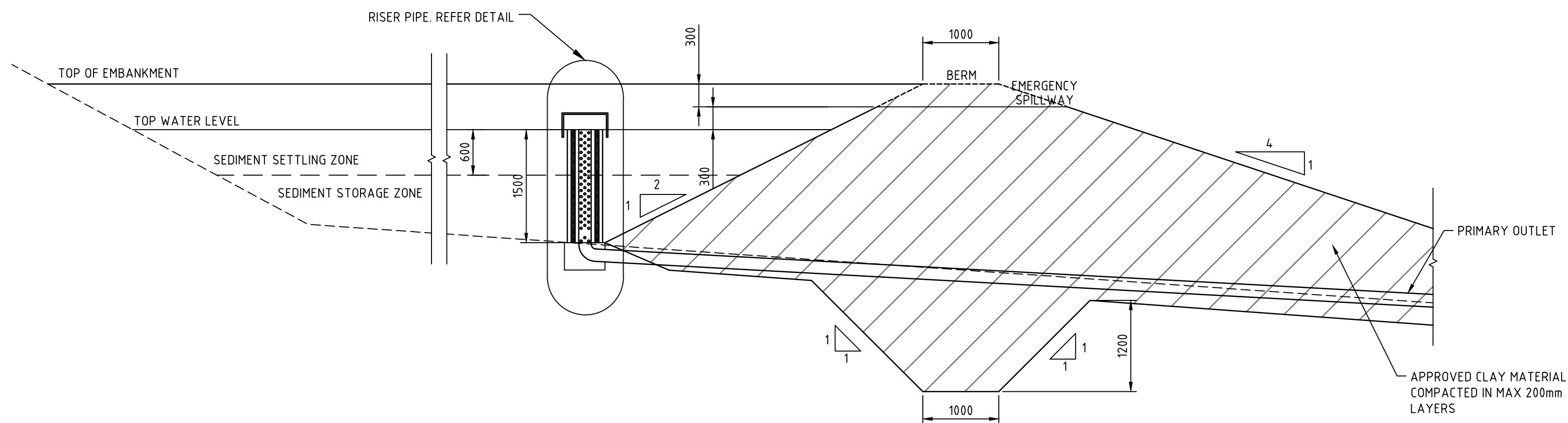
SEDIMENT BASIN TYPE 1 TYPICAL CROSS SECTION 1:50 TYPICAL FOR ALL SEDIMENT BASINS
